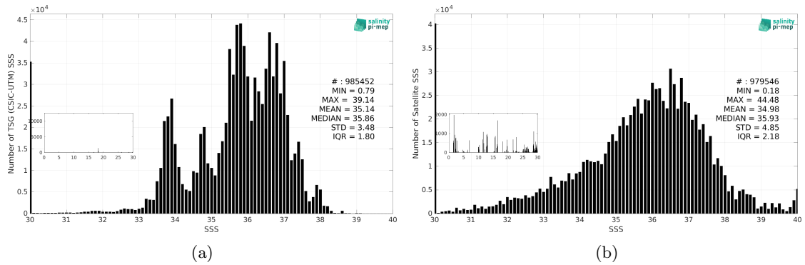
Figure 3: Histograms of SSS from TSG (CSIC-UTM) (a) and SMOS SSS L2Q v331 - With FLAG (CMEMS-CATDS-CPDC) (b) considering all match-up pairs per bins of 0.1 over the Global Ocean Pi-MEP region and for the full satellite product period.
