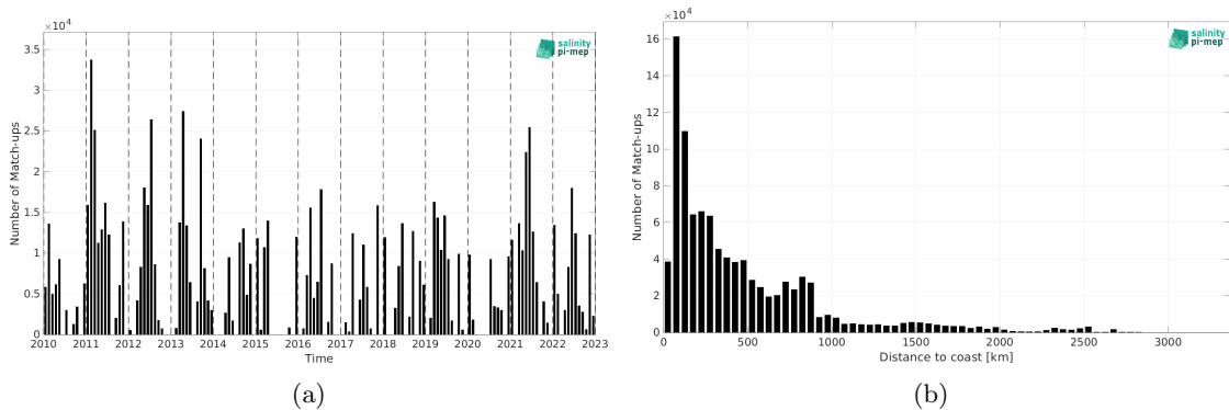
Figure 2: Number of match-ups between TSG (CSIC-UTM) and SMOS SSS L2Q v331 - With FLAG (CMEMS-CATDS-CPDC) SSS as a function of time (a) and as function of the distance to coast (b) over the Global Ocean Pi-MEP region and for the full satellite product period.
