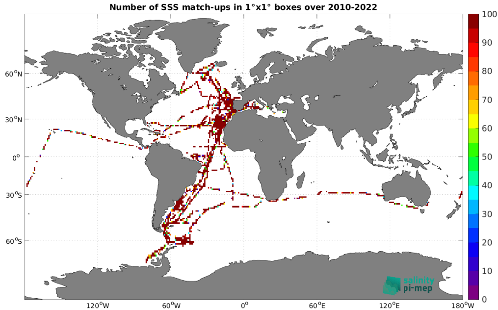
Figure 5: Number of SSS match-ups between TSG (CSIC-UTM) SSS and the SMOS SSS L2Q v331 - With FLAG (CMEMS-CATDS-CPDC) SSS product for the Global Ocean Pi-MEP region over 1^\circ \times 1^\circ boxes and for the full satellite product period.
