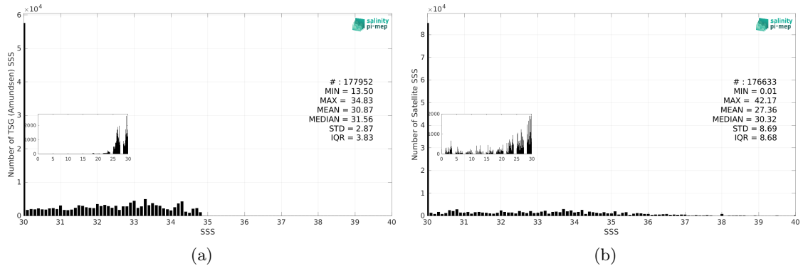
Figure 3: Histograms of SSS from TSG (Amundsen) (a) and SMOS SSS L2Q v331 - With FLAG (CMEMS-CATDS-CPDC) (b) considering all match-up pairs per bins of 0.1 over the Global Ocean Pi-MEP region and for the full satellite product period.
