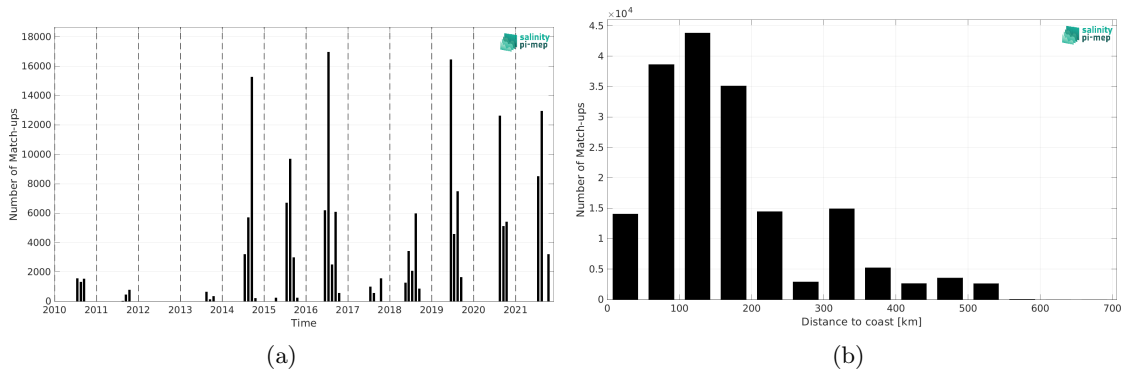
Figure 2: Number of match-ups between TSG (Amundsen) and SMOS SSS L2Q v331 - With FLAG (CMEMS-CATDS-CPDC) SSS as a function of time (a) and as function of the distance to coast (b) over the Global Ocean Pi-MEP region and for the full satellite product period.
