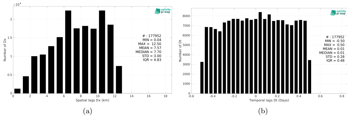
Figure 6: Histograms of the spatial (a) and temporal (b) lags between the location/time of the TSG (Amundsen) measurement and the date of the corresponding SMOS SSS L2Q v331 - With FLAG (CMEMS-CATDS-CPDC) SSS pixel.
