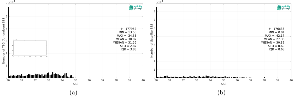
Figure 2: Histograms of SSS from TSG (Amundsen) (a) and SMOS SSS L2Q v331 - With FLAG (CMEMS-CATDS-CPDC) (b) considering all match-up pairs per bins of 0.1 over the Global Ocean Pi-MEP region and for the full satellite product period.
