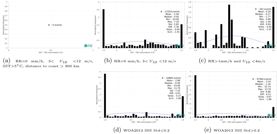
Figure 13: Normalized histogram of \Delta SSS (SMOS SSS L2Q v331 - With FLAG (CMEMS-CATDS-CPDC) - TSG (Amundsen)) for 5 different subdatasets corresponding to: RR=0 mm/h, 3 < U_{10} < 12 m/s, SST>5°C, distance to coast > 800 km (a), RR=0 mm/h, 3 < U_{10} < 12 m/s (b), RR>1mm/h and U_{10} < 4 m/s (c), WOA2013 SSS Std<0.2 (d), WOA2013 SSS Std>0.2 (e).
