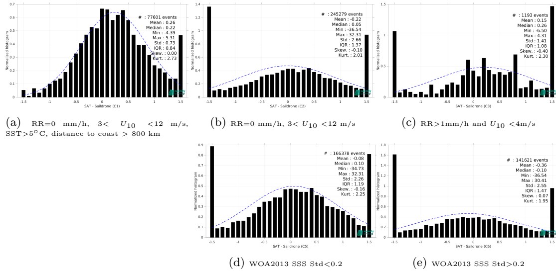
Figure 15: Normalized histogram of \Delta SSS (SMOS SSS L2Q v331 - With FLAG (CMEMS-CATDS-CPDC) - Saildrone) for 5 different subdatasets corresponding to: RR=0 mm/h, 3 < U_{10} < 12 m/s, SST>5°C, distance to coast > 800 km (a), RR=0 mm/h, 3 < U_{10} < 12 m/s (b), RR>1mm/h and U_{10} < 4 m/s (c), WOA2013 SSS Std<0.2 (d), WOA2013 SSS Std>0.2 (e).
