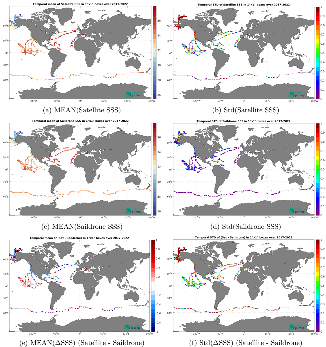
Figure 7: Temporal mean (left) and Std (right) of SSS from SMOS SSS L2Q v331 - With FLAG (CMEMS-CATDS-CPDC) (top), Saildrone (middle), and of \Delta SSS (Satellite - Saildrone). Only match-up pairs are used to generate these maps.
