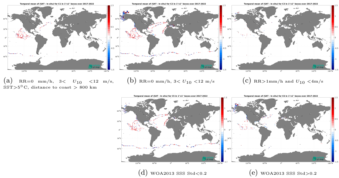
Figure 14: Temporal mean gridded over spatial boxes of size 1^\circ \times 1^\circ of \Delta SSS (SMOS SSS L2Q v331 - With FLAG (CMEMS-CATDS-CPDC) - Saildrone) for 5 different subdatasets corresponding to:RR=0 mm/h, 3 < U_{10} < 12 m/s, SST > 5^\circ\text{C} , distance to coast > 800 km (a), RR=0 mm/h, 3 < U_{10} < 12 m/s (b), RR > 1 mm/h and U_{10} < 4 m/s (c), WOA2013 SSS Std < 0.2 (d), WOA2013 SSS Std > 0.2 (e).
