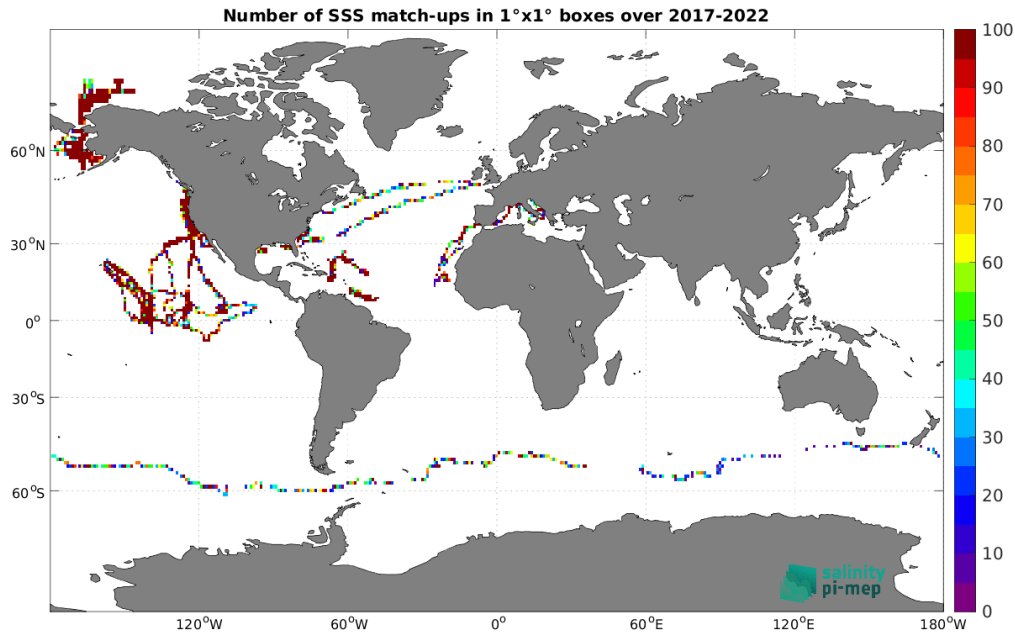
Figure 5: Number of SSS match-ups between Saildrone SSS and the SMOS SSS L2Q v331 - With FLAG (CMEMS-CATDS-CPDC) SSS product for the Global Ocean Pi-MEP region over 1^\circ \times 1^\circ boxes and for the full satellite product period.
