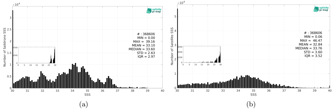
Figure 3: Histograms of SSS from Saildrone (a) and SMOS SSS L2Q v331 - With FLAG (CMEMS-CATDS-CPDC) (b) considering all match-up pairs per bins of 0.1 over the Global Ocean Pi-MEP region and for the full satellite product period.
