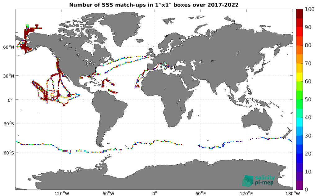
Figure 4: Number of SSS match-ups between Saildrone SSS and the SMOS SSS L2Q v331 - With FLAG (CMEMS-CATDS-CPDC) SSS product for the Global Ocean Pi-MEP region over 1^\circ \times 1^\circ boxes and for the full satellite product period.
