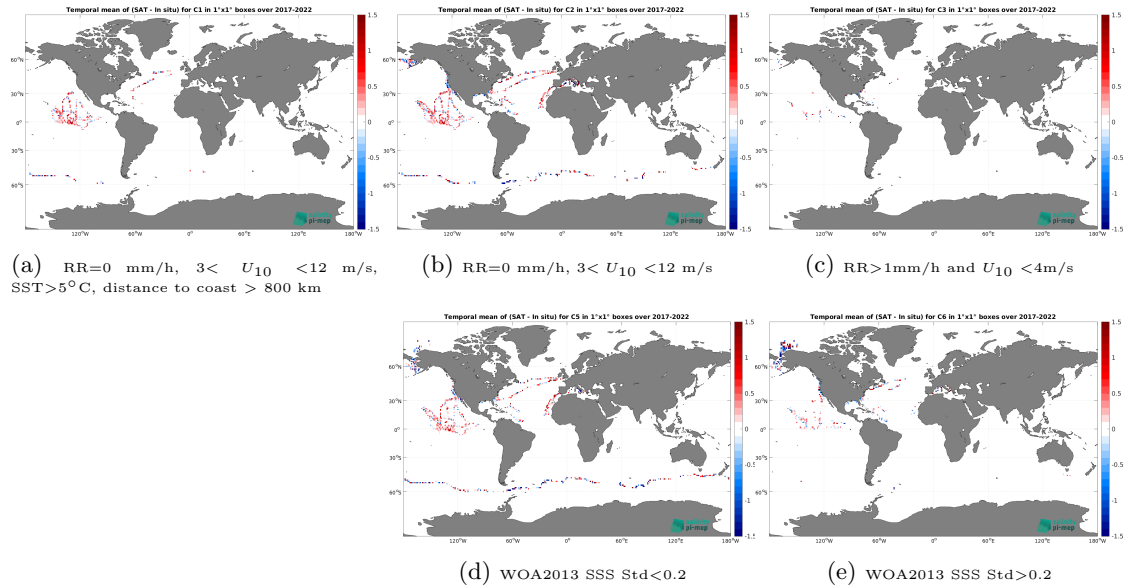
Figure 12: Temporal mean gridded over spatial boxes of size 1^\circ \times 1^\circ of \Delta SSS (SMOS SSS L2Q v331 - With FLAG (CMEMS-CATDS-CPDC) - Saildrone) for 5 different subdatasets corresponding to:RR=0 mm/h, 3 < U_{10} < 12 m/s, SST >5^\circ C, distance to coast > 800 km (a), RR=0 mm/h, 3 < U_{10} < 12 m/s (b), RR >1 mm/h and U_{10} < 4 m/s (c), WOA2013 SSS Std <0.2 (d), WOA2013 SSS Std >0.2 (e).
