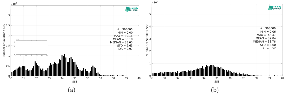
Figure 2: Histograms of SSS from Saildrone (a) and SMOS SSS L2Q v331 - With FLAG (CMEMS-CATDS-CPDC) (b) considering all match-up pairs per bins of 0.1 over the Global Ocean Pi-MEP region and for the full satellite product period.
