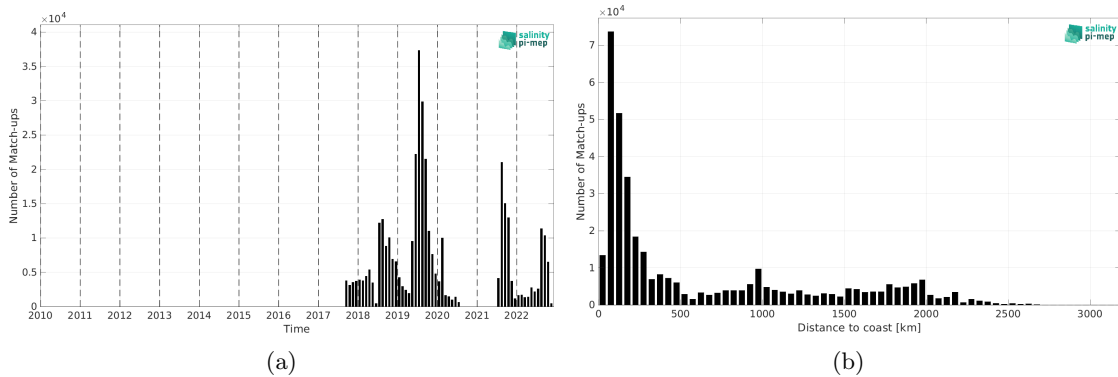
Figure 1: Number of match-ups between Saildrone and SMOS SSS L2Q v331 - With FLAG (CMEMS-CATDS-CPDC) SSS as a function of time (a) and as function of the distance to coast (b) over the Global Ocean Pi-MEP region and for the full satellite product period.
