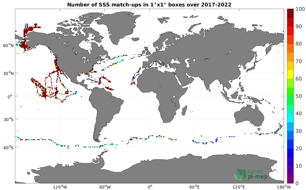
Figure 4: Number of SSS match-ups between Sairdrone SSS and the SMOS SSS L2Q v331 - With FLAG (CMEMS-CATDS-CPDC) SSS product for the Global Ocean Pi-MEP region over 1^\circ \times 1^\circ boxes and for the full satellite product period.
