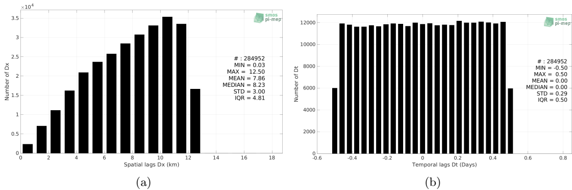
Figure 5: Histograms of the spatial (a) and temporal (b) lags between the location/time of the Sairdrone measurement and the date of the corresponding SMOS SSS L2Q v331 - With FLAG (CMEMS-CATDS-CPDC) SSS pixel.
