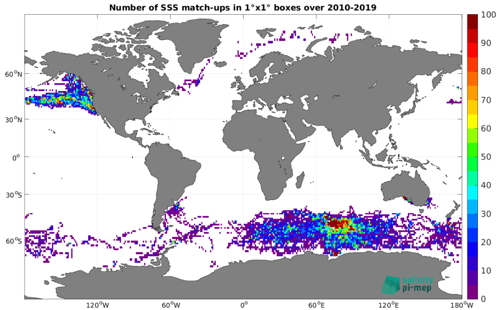
Figure 4: Number of SSS match-ups between Marine mammals SSS and the SMOS SSS L2Q v331 - With FLAG (CMEMS-CATDS-CPDC) SSS product for the Global Ocean Pi-MEP region over 1^\circ \times 1^\circ boxes and for the full satellite product period.
