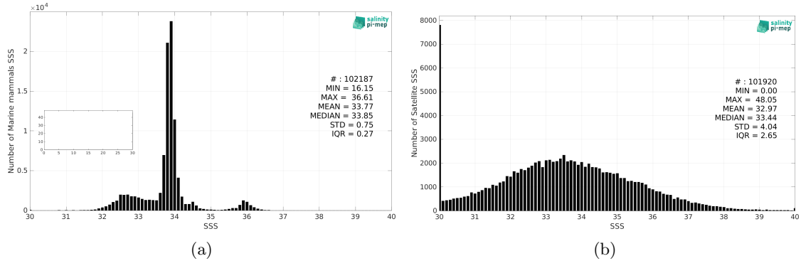
Figure 2: Histograms of SSS from Marine mammals (a) and SMOS SSS L2Q v331 - With FLAG (CMEMS-CATDS-CPDC) (b) considering all match-up pairs per bins of 0.1 over the Global Ocean Pi-MEP region and for the full satellite product period.
