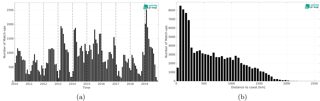
Figure 1: Number of match-ups between Marine mammals and SMOS SSS L2Q v331 - With FLAG (CMEMS-CATDS-CPDC) SSS as a function of time (a) and as function of the distance to coast (b) over the Global Ocean Pi-MEP region and for the full satellite product period.
