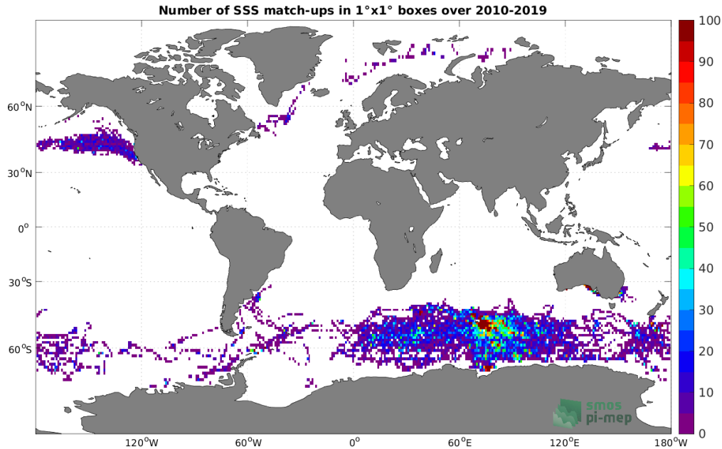
Figure 4: Number of SSS match-ups between Marine mammals SSS and the SMOS SSS L2Q v331 - With FLAG (CMEMS-CATDS-CPDC) SSS product for the Global Ocean Pi-MEP region over 1°×1° boxes and for the full satellite product period.
