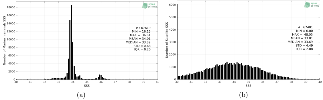
Figure 2: Histograms of SSS from Marine mammals (a) and SMOS SSS L2Q v331 - With FLAG (CMEMS-CATDS-CPDC) (b) considering all match-up pairs per bins of 0.1 over the Global Ocean Pi-MEP region and for the full satellite product period.
