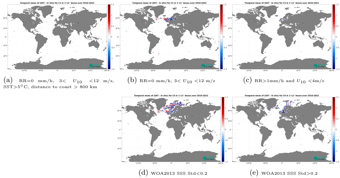
Figure 12: Temporal mean gridded over spatial boxes of size 1^\circ \times 1^\circ of \Delta SSS (SMOS SSS L2Q v331 - With FLAG (CMEMS-CATDS-CPDC) - ICES) for 5 different subdatasets corresponding to: RR=0 mm/h, 3 < U_{10} < 12 m/s, SST > 5^\circ\text{C} , distance to coast > 800 km (a), RR=0 mm/h, 3 < U_{10} < 12 m/s (b), RR > 1 mm/h and U_{10} < 4 m/s (c), WOA2013 SSS Std < 0.2 (d), WOA2013 SSS Std > 0.2 (e).
