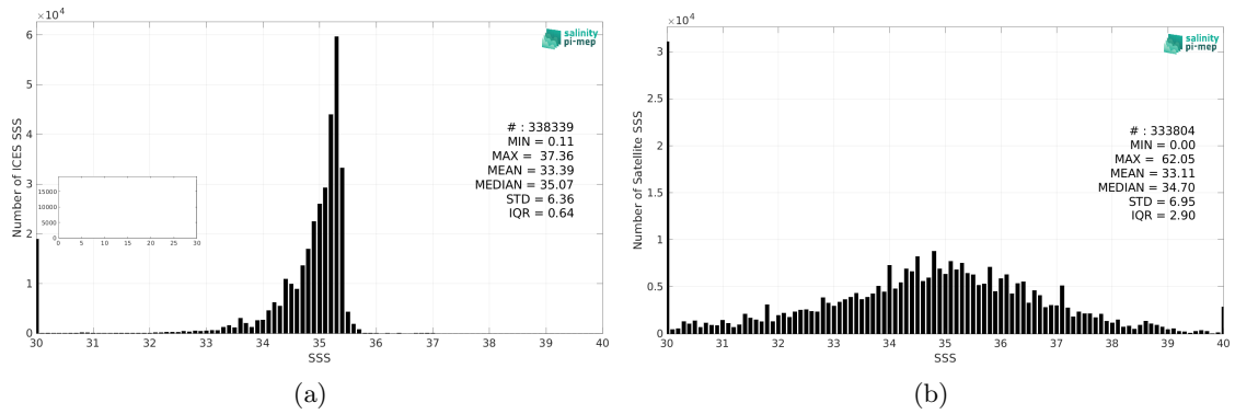
Figure 2: Histograms of SSS from ICES (a) and SMOS SSS L2Q v331 - With FLAG (CMEMS-CATDS-CPDC) (b) considering all match-up pairs per bins of 0.1 over the Global Ocean Pi-MEP region and for the full satellite product period.
