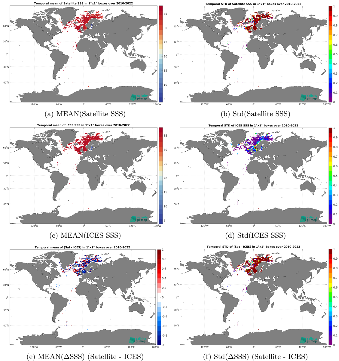
Figure 6: Temporal mean (left) and Std (right) of SSS from SMOS SSS L2Q v331 - With FLAG (CMEMS-CATDS-CPDC) (top), ICES (middle), and of \Delta SSS (Satellite - ICES). Only match-up pairs are used to generate these maps.
