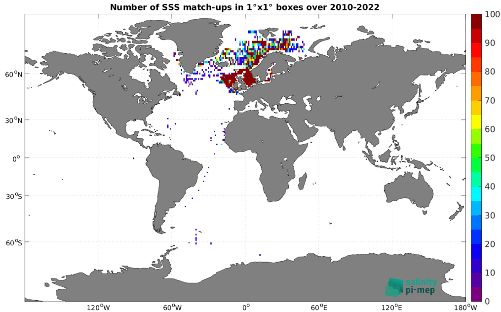
Figure 4: Number of SSS match-ups between ICES SSS and the SMOS SSS L2Q v331 - With FLAG (CMEMS-CATDS-CPDC) SSS product for the Global Ocean Pi-MEP region over 1^\circ \times 1^\circ boxes and for the full satellite product period.
