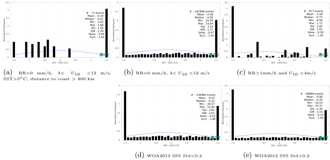
Figure 13: Normalized histogram of \Delta SSS (SMOS SSS L2Q v331 - With FLAG (CMEMS-CATDS-CPDC) - ICES) for 5 different subdatasets corresponding to: RR=0 mm/h, 3 < U_{10} < 12 m/s, SST > 5°C, distance to coast > 800 km (a), RR=0 mm/h, 3 < U_{10} < 12 m/s (b), RR > 1mm/h and U_{10} < 4 m/s (c), WOA2013 SSS Std < 0.2 (d), WOA2013 SSS Std > 0.2 (e).
