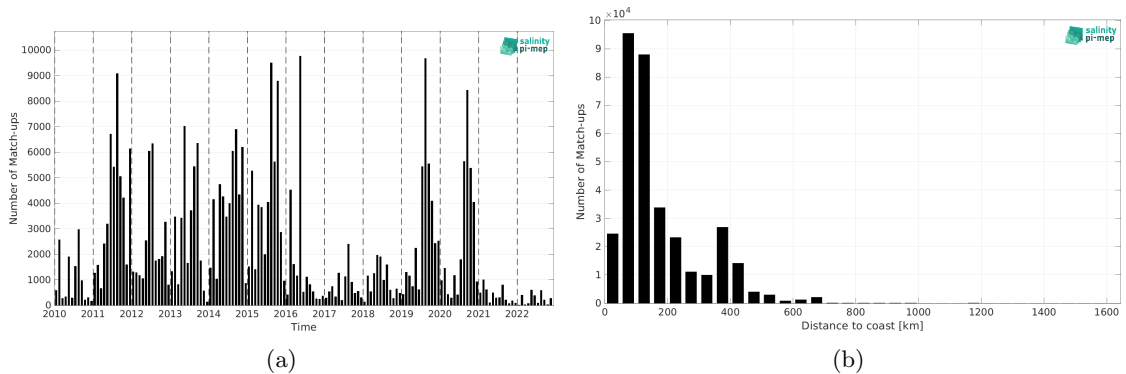
Figure 1: Number of match-ups between ICES and SMOS SSS L2Q v331 - With FLAG (CMEMS-CATDS-CPDC) SSS as a function of time (a) and as function of the distance to coast (b) over the Global Ocean Pi-MEP region and for the full satellite product period.
