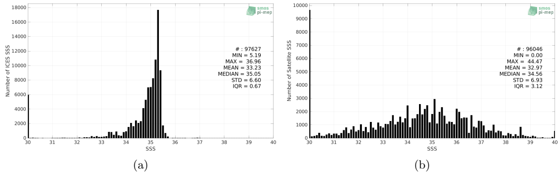
Figure 2: Histograms of SSS from ICES (a) and SMOS SSS L2Q v331 - With FLAG (CMEMS-CATDS-CPDC) (b) considering all match-up pairs per bins of 0.1 over the Global Ocean Pi-MEP region and for the full satellite product period.
