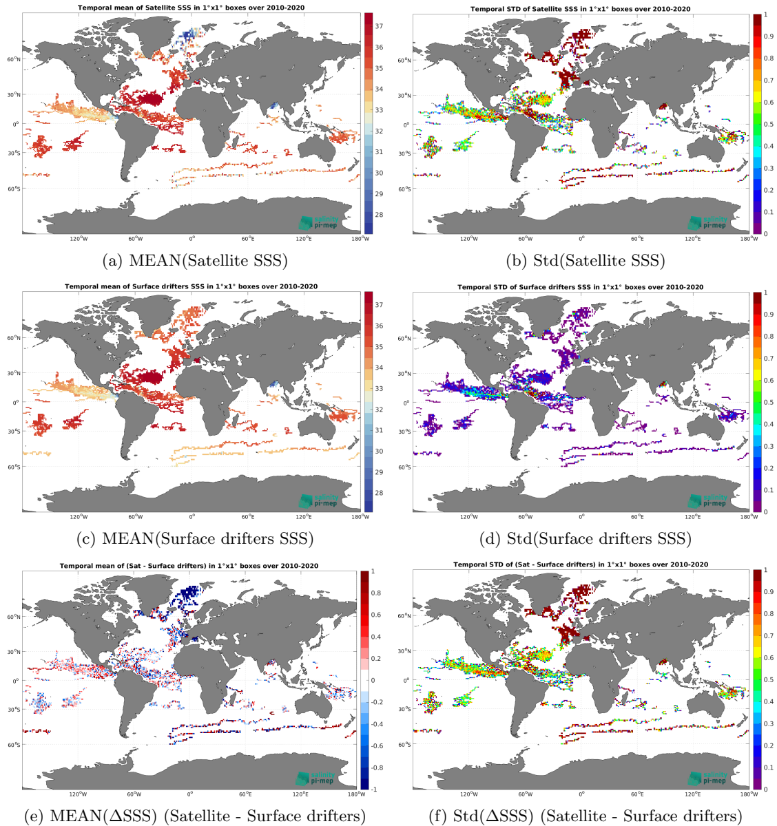
Figure 6: Temporal mean (left) and Std (right) of SSS from SMOS SSS L2Q v331 - With FLAG (CMEMS-CATDS-CPDC) (top), Surface drifters (middle), and of \Delta SSS (Satellite - Surface drifters). Only match-up pairs are used to generate these maps.
