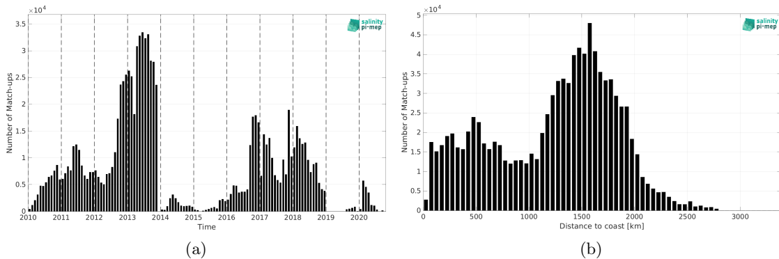
Figure 2: Number of match-ups between Surface drifters and SMOS SSS L2Q v331 - With FLAG (CMEMS-CATDS-CPDC) SSS as a function of time (a) and as function of the distance to coast (b) over the Global Ocean Pi-MEP region and for the full satellite product period.
