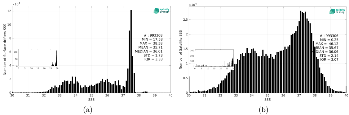
Figure 3: Histograms of SSS from Surface drifters (a) and SMOS SSS L2Q v331 - With FLAG (CMEMS-CATDS-CPDC) (b) considering all match-up pairs per bins of 0.1 over the Global Ocean Pi-MEP region and for the full satellite product period.
