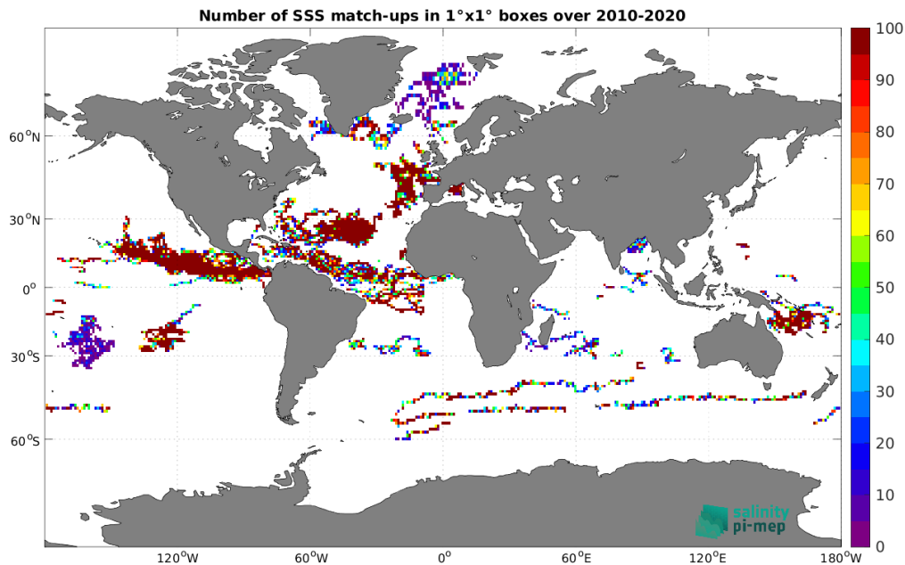
Figure 4: Number of SSS match-ups between Surface drifters SSS and the SMOS SSS L2Q v331 - With FLAG (CMEMS-CATDS-CPDC) SSS product for the Global Ocean Pi-MEP region over 1^\circ \times 1^\circ boxes and for the full satellite product period.
