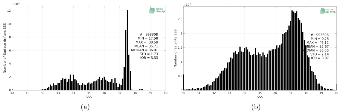
Figure 2: Histograms of SSS from Surface drifters (a) and SMOS SSS L2Q v331 - With FLAG (CMEMS-CATDS-CPDC) (b) considering all match-up pairs per bins of 0.1 over the Global Ocean Pi-MEP region and for the full satellite product period.
