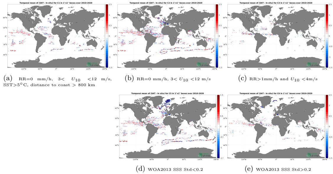
Figure 11: Temporal mean gridded over spatial boxes of size 1^\circ \times 1^\circ of \Delta SSS (SMOS SSS L2Q v331 - With FLAG (CMEMS-CATDS-CPDC) - Surface drifters) for 5 different subdatasets corresponding to: RR=0 mm/h, 3 < U_{10} < 12 m/s, SST > 5^\circ\text{C} , distance to coast > 800 km (a), RR=0 mm/h, 3 < U_{10} < 12 m/s (b), RR > 1 mm/h and U_{10} < 4 m/s (c), WOA2013 SSS Std < 0.2 (d), WOA2013 SSS Std > 0.2 (e).
