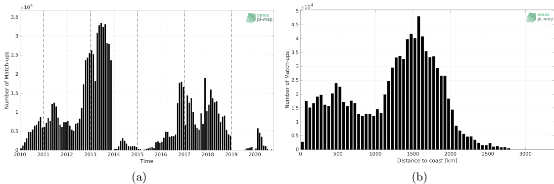
Figure 1: Number of match-ups between Surface drifters and SMOS SSS L2Q v331 - With FLAG (CMEMS-CATDS-CPDC) SSS as a function of time (a) and as function of the distance to coast (b) over the Global Ocean Pi-MEP region and for the full satellite product period.
