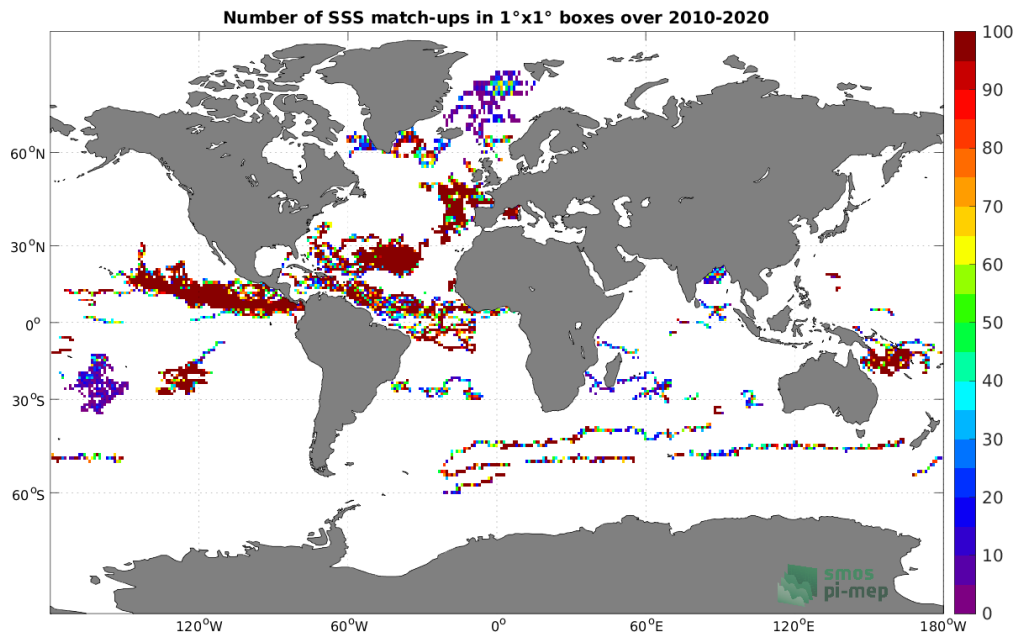
Figure 3: Number of SSS match-ups between Surface drifters SSS and the SMOS SSS L2Q v331 - With FLAG (CMEMS-CATDS-CPDC) SSS product for the Global Ocean Pi-MEP region over 1^\circ \times 1^\circ boxes and for the full satellite product period.
