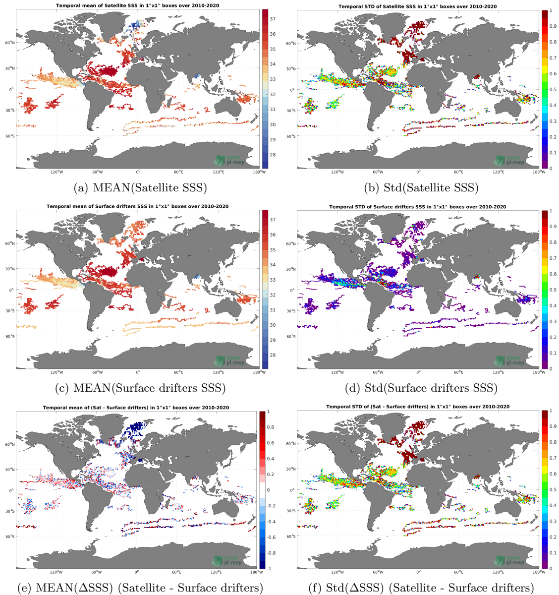
Figure 5: Temporal mean (left) and Std (right) of SSS from SMOS SSS L2Q v331 - With FLAG (CMEMS-CATDS-CPDC) (top), Surface drifters (middle), and of \Delta SSS (Satellite - Surface drifters). Only match-up pairs are used to generate these maps.
