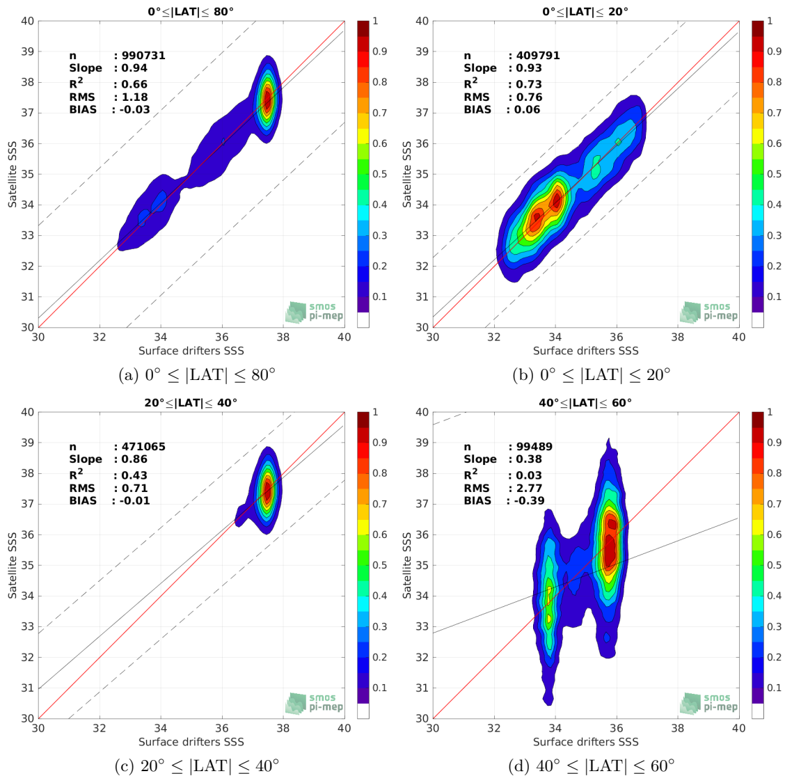
Figure 8: Contour maps of the concentration of SMOS SSS L2Q v331 - With FLAG (CMEMS-CATDS-CPDC) SSS (y-axis) versus Surface drifters SSS (x-axis) at match-up pairs for different latitude bands. For each plot, the red line shows x=y . The black thin and dashed lines indicate a linear fit through the data cloud and the \pm 95\% confidence levels, respectively. The number match-up pairs n , the slope and R^2 coefficient of the linear fit, the root mean square (RMS) and the mean bias between satellite and in situ data are indicated for each latitude band in each plots.
