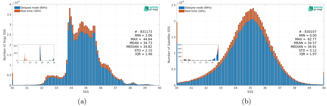
Figure 3: Histograms of SSS from Argo (a) and SMOS SSS L2Q v331 - With FLAG (CMEMS-CATDS-CPDC) (b) considering all match-up pairs per bins of 0.1 over the Global Ocean Pi-MEP region and for the full satellite product period.
