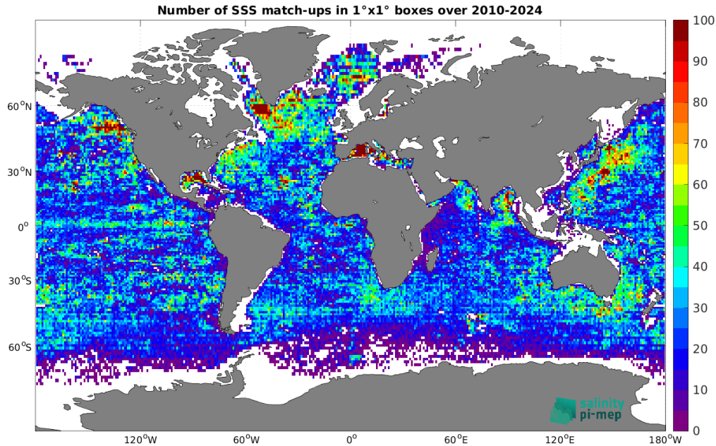
Figure 5: Number of SSS match-ups between Argo SSS and the SMOS SSS L2Q v331 - With FLAG (CMEMS-CATDS-CPDC) SSS product for the Global Ocean Pi-MEP region over 1^\circ \times 1^\circ boxes and for the full satellite product period.
