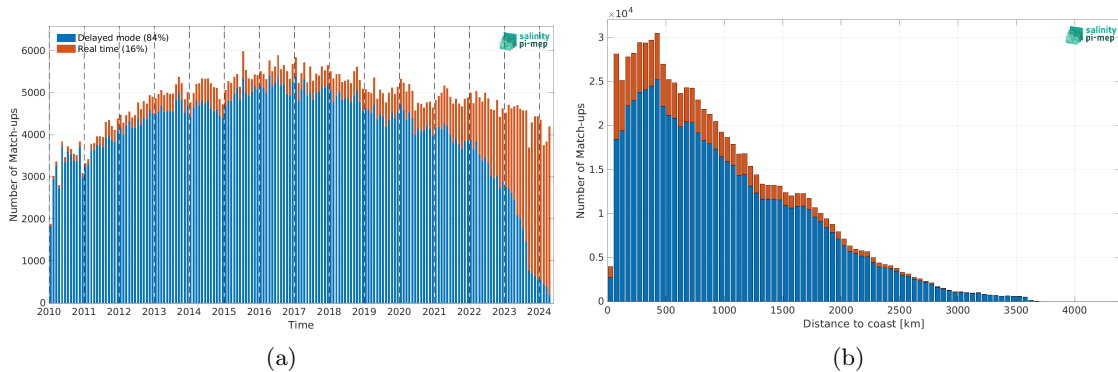
Figure 2: Number of match-ups between Argo and SMOS SSS L2Q v331 - With FLAG (CMEMS-CATDS-CPDC) SSS as a function of time (a) and as function of the distance to coast (b) over the Global Ocean Pi-MEP region and for the full satellite product period.
