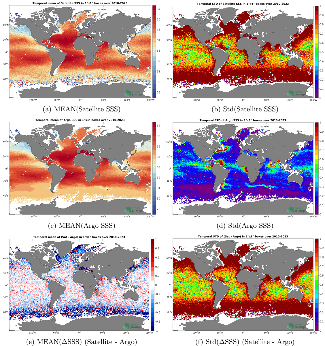
Figure 6: Temporal mean (left) and Std (right) of SSS from SMOS SSS L2Q v331 - With FLAG (CMEMS-CATDS-CPDC) (top), Argo (middle), and of \Delta SSS (Satellite - Argo). Only match-up pairs are used to generate these maps.
