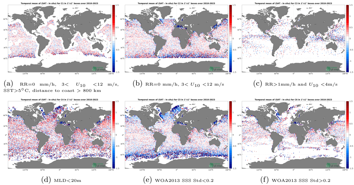
Figure 12: Temporal mean gridded over spatial boxes of size 1^\circ \times 1^\circ of \Delta SSS (SMOS SSS L2Q v331 - With FLAG (CMEMS-CATDS-CPDC) - Argo) for 6 different subdatasets corresponding to:RR=0 mm/h, 3 < U_{10} < 12 m/s, SST > 5^\circ\text{C} , distance to coast > 800 km (a), RR=0 mm/h, 3 < U_{10} < 12 m/s (b), RR > 1 mm/h and U_{10} < 4 m/s (c),MLD < 20 m (d),WOA2013 SSS Std < 0.2 (e),WOA2013 SSS Std > 0.2 (f).
