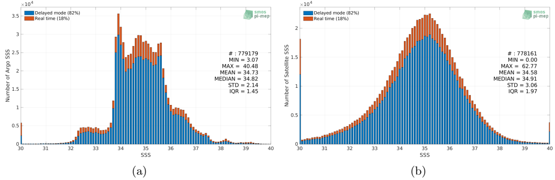
Figure 2: Histograms of SSS from Argo (a) and SMOS SSS L2Q v331 - With FLAG (CMEMS-CATDS-CPDC) (b) considering all match-up pairs per bins of 0.1 over the Global Ocean Pi-MEP region and for the full satellite product period.
