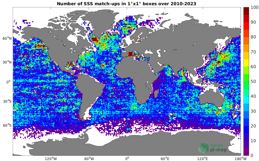
Figure 4: Number of SSS match-ups between Argo SSS and the SMOS SSS L2Q v331 - With FLAG (CMEMS-CATDS-CPDC) SSS product for the Global Ocean Pi-MEP region over 1^\circ \times 1^\circ boxes and for the full satellite product period.
