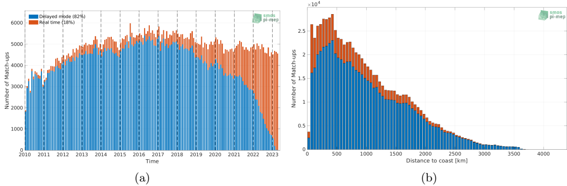
Figure 1: Number of match-ups between Argo and SMOS SSS L2Q v331 - With FLAG (CMEMS-CATDS-CPDC) SSS as a function of time (a) and as function of the distance to coast (b) over the Global Ocean Pi-MEP region and for the full satellite product period.
