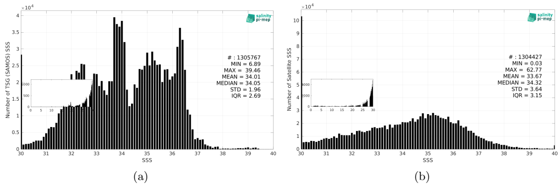
Figure 3: Histograms of SSS from TSG (SAMOS) (a) and SMOS SSS L2Q v331 - No FLAG (CMEMS-CATDS-CPDC) (b) considering all match-up pairs per bins of 0.1 over the Global Ocean Pi-MEP region and for the full satellite product period.
