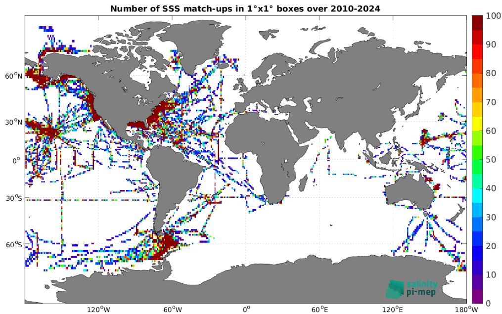
Figure 5: Number of SSS match-ups between TSG (SAMOS) SSS and the SMOS SSS L2Q v331 - No FLAG (CMEMS-CATDS-CPDC) SSS product for the Global Ocean Pi-MEP region over 1^\circ \times 1^\circ boxes and for the full satellite product period.
