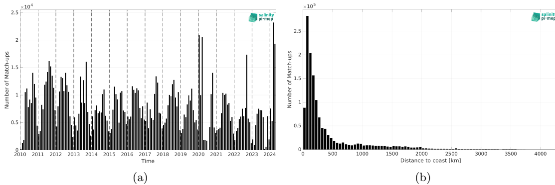
Figure 2: Number of match-ups between TSG (SAMOS) and SMOS SSS L2Q v331 - No FLAG (CMEMS-CATDS-CPDC) SSS as a function of time (a) and as function of the distance to coast (b) over the Global Ocean Pi-MEP region and for the full satellite product period.
