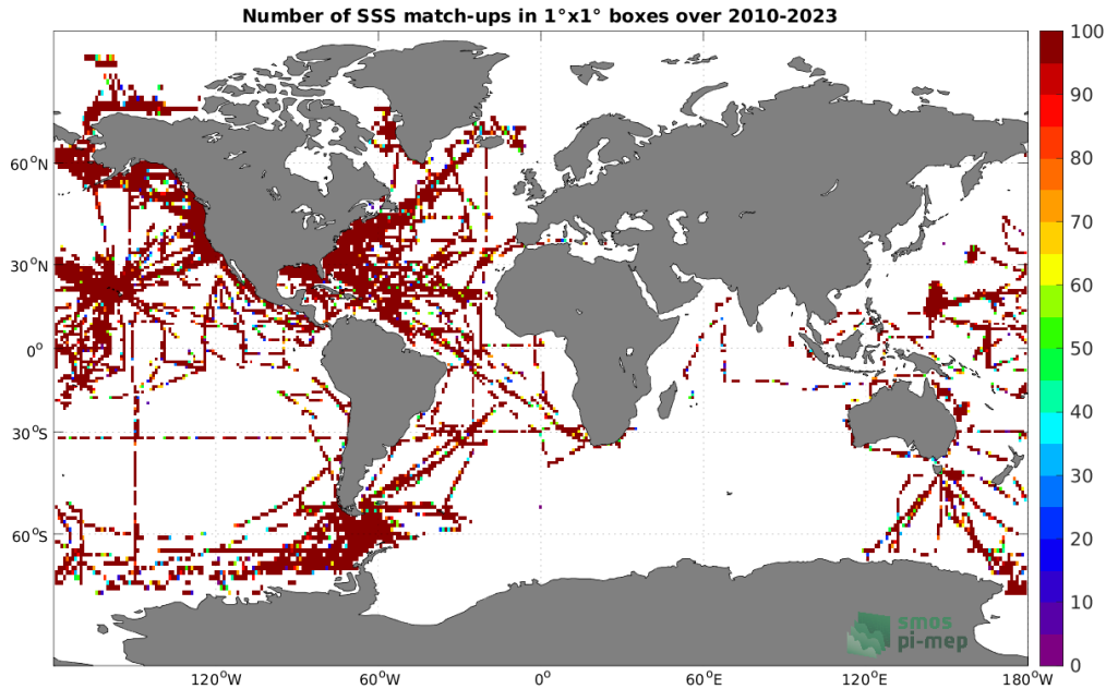
Figure 4: Number of SSS match-ups between TSG (SAMOS) SSS and the SMOS SSS L2Q v331 - No FLAG (CMEMS-CATDS-CPDC) SSS product for the Global Ocean Pi-MEP region over 1°×1° boxes and for the full satellite product period.
