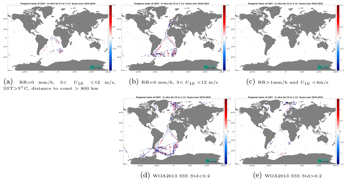
Figure 12: Temporal mean gridded over spatial boxes of size 1^\circ \times 1^\circ of \Delta SSS (SMOS SSS L2Q v331 - No FLAG (CMEMS-CATDS-CPDC) - TSG (Polarstern)) for 5 different subdatasets corresponding to: RR=0 mm/h, 3 < U_{10} < 12 m/s, SST > 5^\circ\text{C} , distance to coast > 800 km (a), RR=0 mm/h, 3 < U_{10} < 12 m/s (b), RR > 1 mm/h and U_{10} < 4 m/s (c), WOA2013 SSS Std < 0.2 (d), WOA2013 SSS Std > 0.2 (e).
