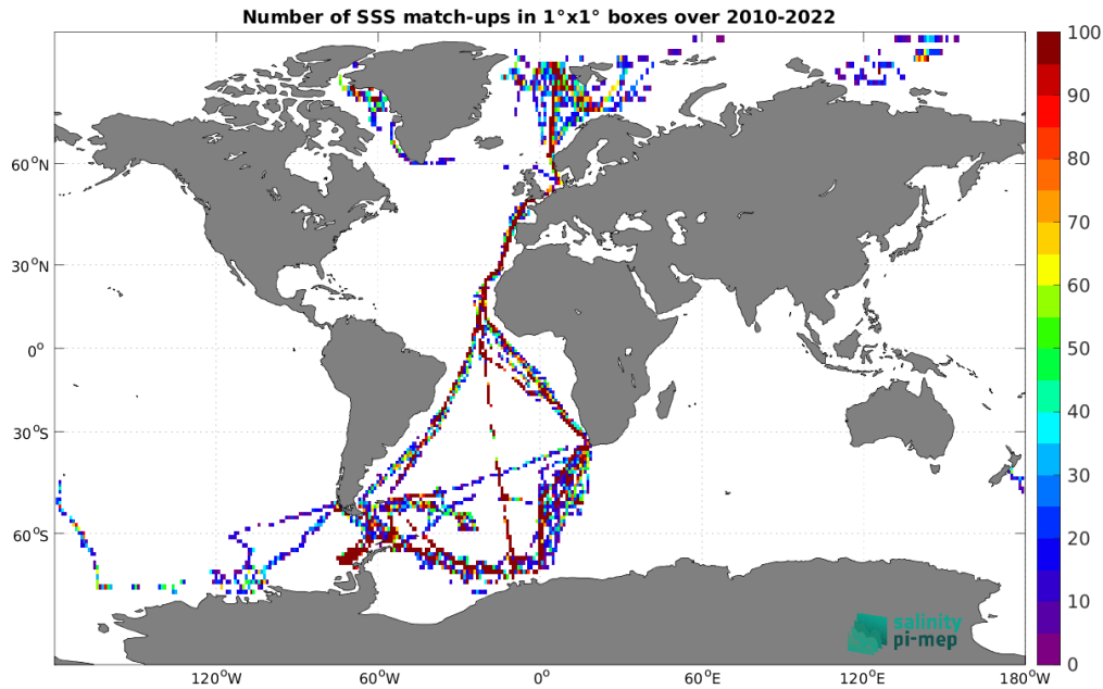
Figure 4: Number of SSS match-ups between TSG (Polarstern) SSS and the SMOS SSS L2Q v331 - No FLAG (CMEMS-CATDS-CPDC) SSS product for the Global Ocean Pi-MEP region over 1^\circ \times 1^\circ boxes and for the full satellite product period.
