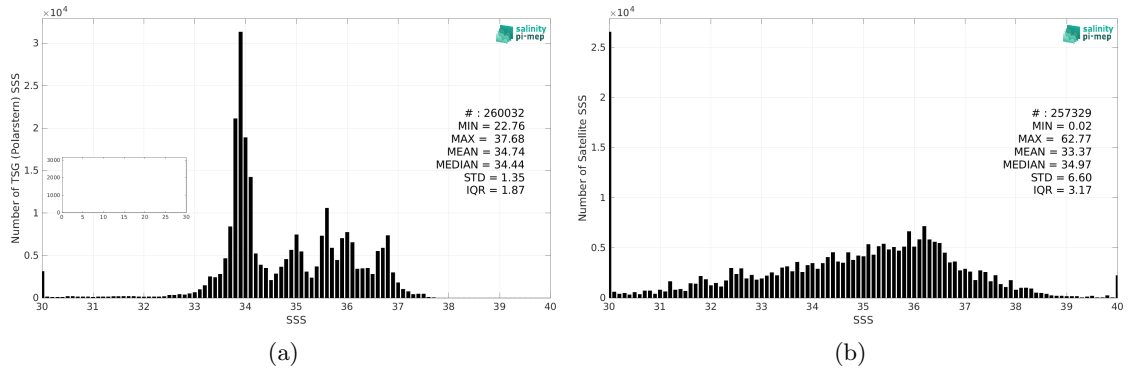
Figure 2: Histograms of SSS from TSG (Polarstern) (a) and SMOS SSS L2Q v331 - No FLAG (CMEMS-CATDS-CPDC) (b) considering all match-up pairs per bins of 0.1 over the Global Ocean Pi-MEP region and for the full satellite product period.
