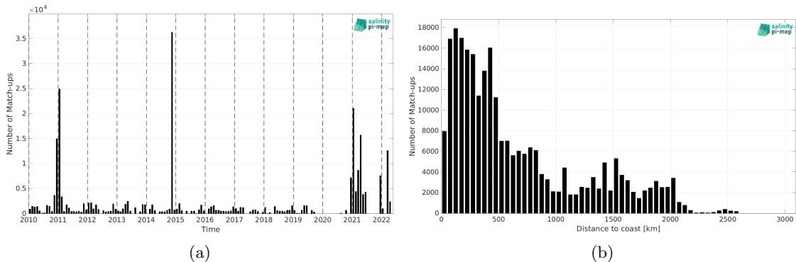
Figure 1: Number of match-ups between TSG (Polarstern) and SMOS SSS L2Q v331 - No FLAG (CMEMS-CATDS-CPDC) SSS as a function of time (a) and as function of the distance to coast (b) over the Global Ocean Pi-MEP region and for the full satellite product period.
