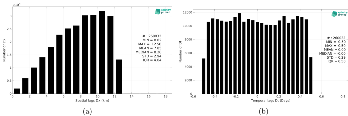
Figure 5: Histograms of the spatial (a) and temporal (b) lags between the location/time of the TSG (Polarstern) measurement and the date of the corresponding SMOS SSS L2Q v331 - No FLAG (CMEMS-CATDS-CPDC) SSS pixel.
