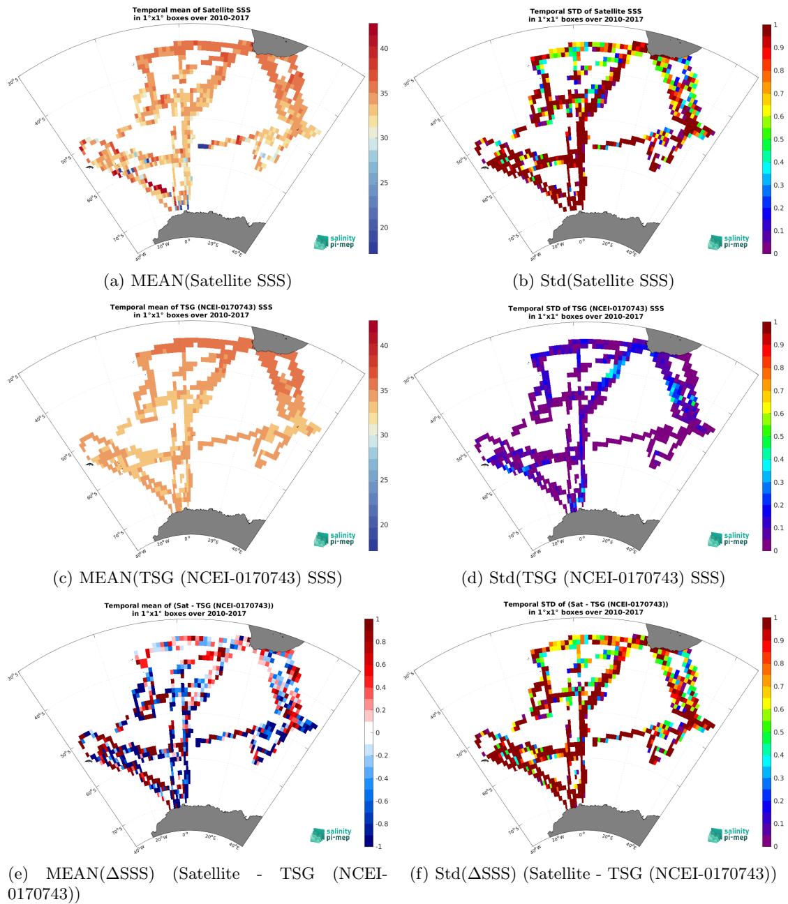
Figure 7: Temporal mean (left) and Std (right) of SSS from SMOS SSS L2Q v331 - No FLAG (CMEMS-CATDS-CPDC) (top), TSG (NCEI-0170743) (middle), and of \Delta SSS (Satellite - TSG (NCEI-0170743)). Only match-up pairs are used to generate these maps.
