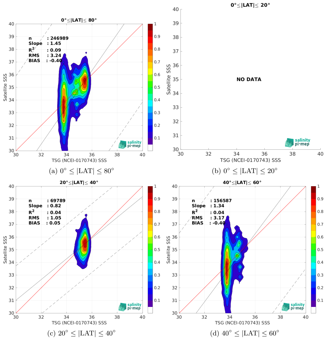
Figure 10: Contour maps of the concentration of SMOS SSS L2Q v331 - No FLAG (CMEMS-CATDS-CPDC) SSS (y-axis) versus TSG (NCEI-0170743) SSS (x-axis) at match-up pairs for different latitude bands. For each plot, the red line shows x=y . The black thin and dashed lines indicate a linear fit through the data cloud and the \pm 95\% confidence levels, respectively. The number match-up pairs n , the slope and R^2 coefficient of the linear fit, the root mean square (RMS) and the mean bias between satellite and in situ data are indicated for each latitude band in each plots.
