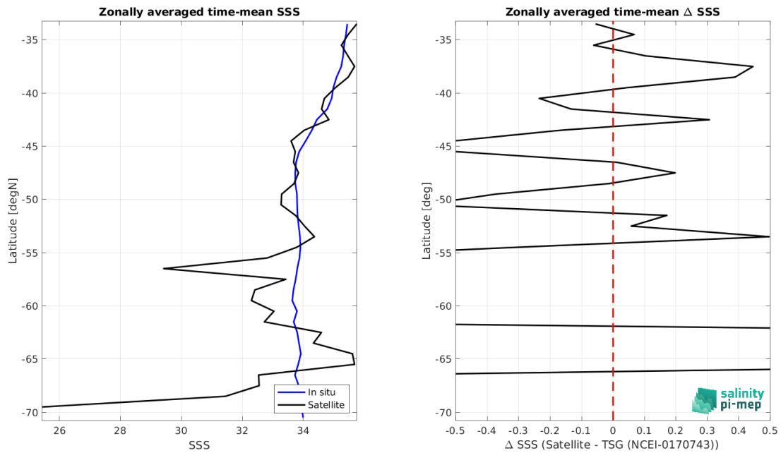
Figure 9: Left panel: Zonal mean SSS from SMOS SSS L2Q v331 - No FLAG (CMEMS-CATDS-CPDC) satellite product (black) and from TSG (NCEI-0170743) (blue). Right panel: Zonal mean of \Delta SSS (Satellite - TSG (NCEI-0170743)) for all the collected Pi-MEP match-up pairs estimated over the full satellite product period.
