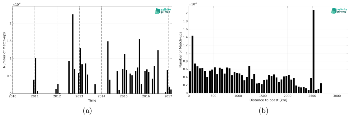
Figure 2: Number of match-ups between TSG (NCEI-0170743) and SMOS SSS L2Q v331 - No FLAG (CMEMS-CATDS-CPDC) SSS as a function of time (a) and as function of the distance to coast (b) over the Global Ocean Pi-MEP region and for the full satellite product period.
