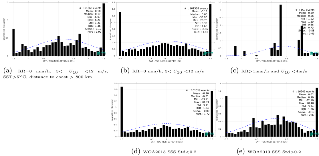
Figure 15: Normalized histogram of \Delta SSS (SMOS SSS L2Q v331 - No FLAG (CMEMS-CATDS-CPDC) - TSG (NCEI-0170743)) for 5 different subdatasets corresponding to: RR=0 mm/h, 3 < U_{10} < 12 m/s, SST > 5°C, distance to coast > 800 km (a), RR=0 mm/h, 3 < U_{10} < 12 m/s (b), RR > 1mm/h and U_{10} < 4 m/s (c), WOA2013 SSS Std < 0.2 (d), WOA2013 SSS Std > 0.2 (e).
