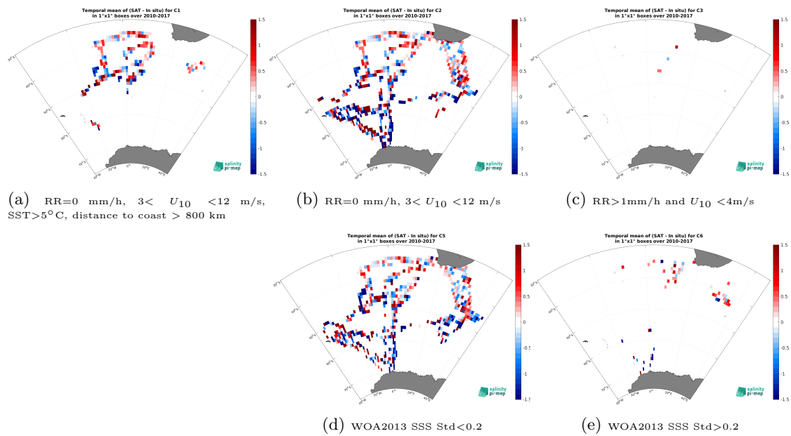
Figure 14: Temporal mean gridded over spatial boxes of size 1^\circ \times 1^\circ of \Delta\text{SSS} (SMOS SSS L2Q v331 - No FLAG (CMEMS-CATDS-CPDC) - TSG (NCEI-0170743)) for 5 different subdatasets corresponding to:RR=0 mm/h, 3 < U_{10} < 12 m/s, SST>5°C, distance to coast > 800 km (a), RR=0 mm/h, 3 < U_{10} < 12 m/s (b), RR>1mm/h and U_{10} < 4 m/s (c), WOA2013 SSS Std<0.2 (d), WOA2013 SSS Std>0.2 (e).
