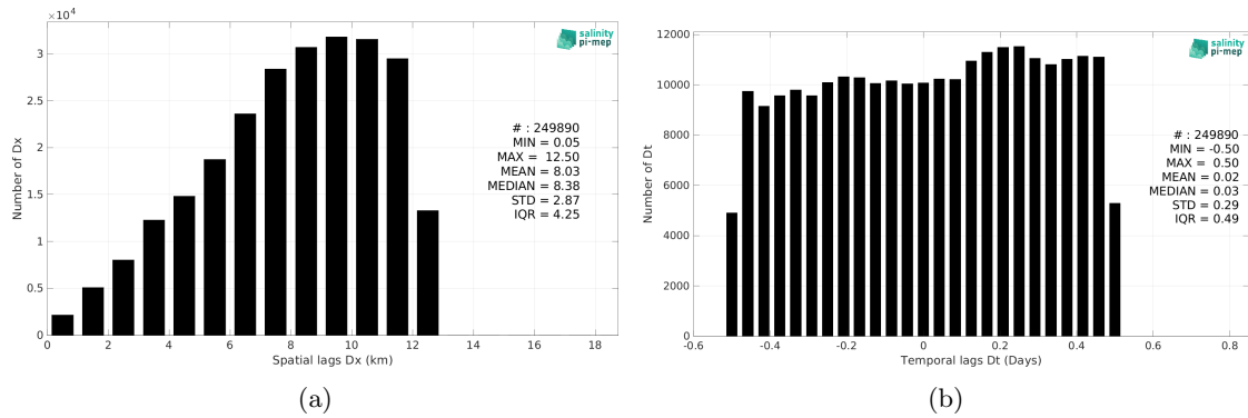
Figure 6: Histograms of the spatial (a) and temporal (b) lags between the location/time of the TSG (NCEI-0170743) measurement and the date of the corresponding SMOS SSS L2Q v331 - No FLAG (CMEMS-CATDS-CPDC) SSS pixel.
