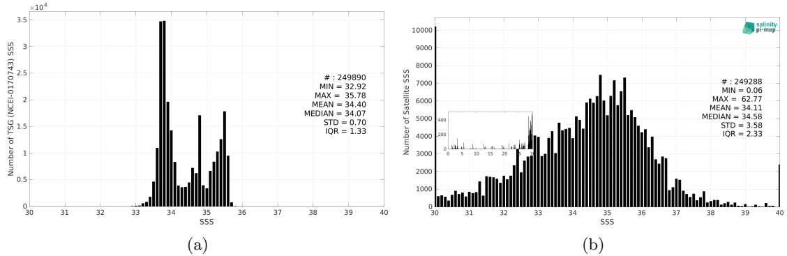
Figure 3: Histograms of SSS from TSG (NCEI-0170743) (a) and SMOS SSS L2Q v331 - No FLAG (CMEMS-CATDS-CPDC) (b) considering all match-up pairs per bins of 0.1 over the Global Ocean Pi-MEP region and for the full satellite product period.
