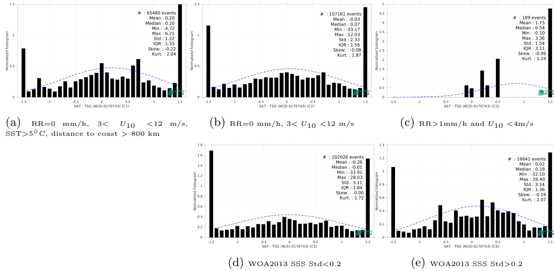
Figure 13: Normalized histogram of \Delta SSS (SMOS SSS L2Q v331 - No FLAG (CMEMS-CATDS-CPDC) - TSG (NCEI-0170743)) for 5 different subdatasets corresponding to: RR=0 mm/h, 3 < U_{10} < 12 m/s, SST>5°C, distance to coast > 800 km (a), RR=0 mm/h, 3 < U_{10} < 12 m/s (b), RR>1mm/h and U_{10} < 4 m/s (c), WOA2013 SSS Std<0.2 (d), WOA2013 SSS Std>0.2 (e).
