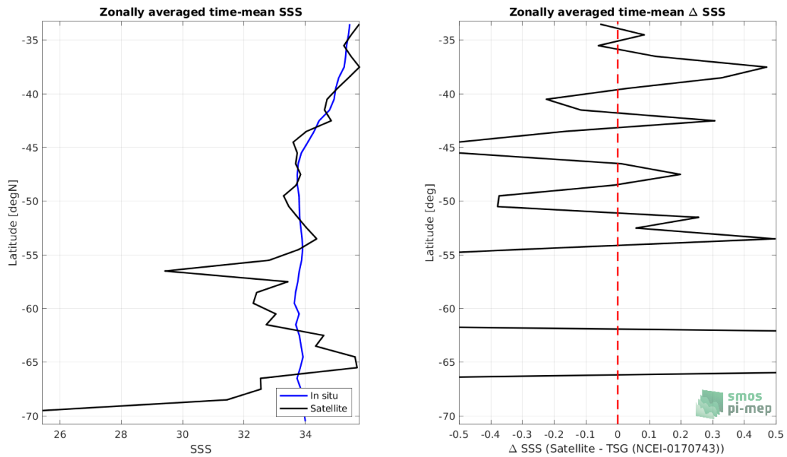
Figure 8: Left panel: Zonal mean SSS from SMOS SSS L2Q v331 - No FLAG (CMEMS-CATDS-CPDC) satellite product (black) and from TSG (NCEI-0170743) (blue). Right panel: Zonal mean of \Delta SSS (Satellite - TSG (NCEI-0170743)) for all the collected Pi-MEP match-up pairs estimated over the full satellite product period.
