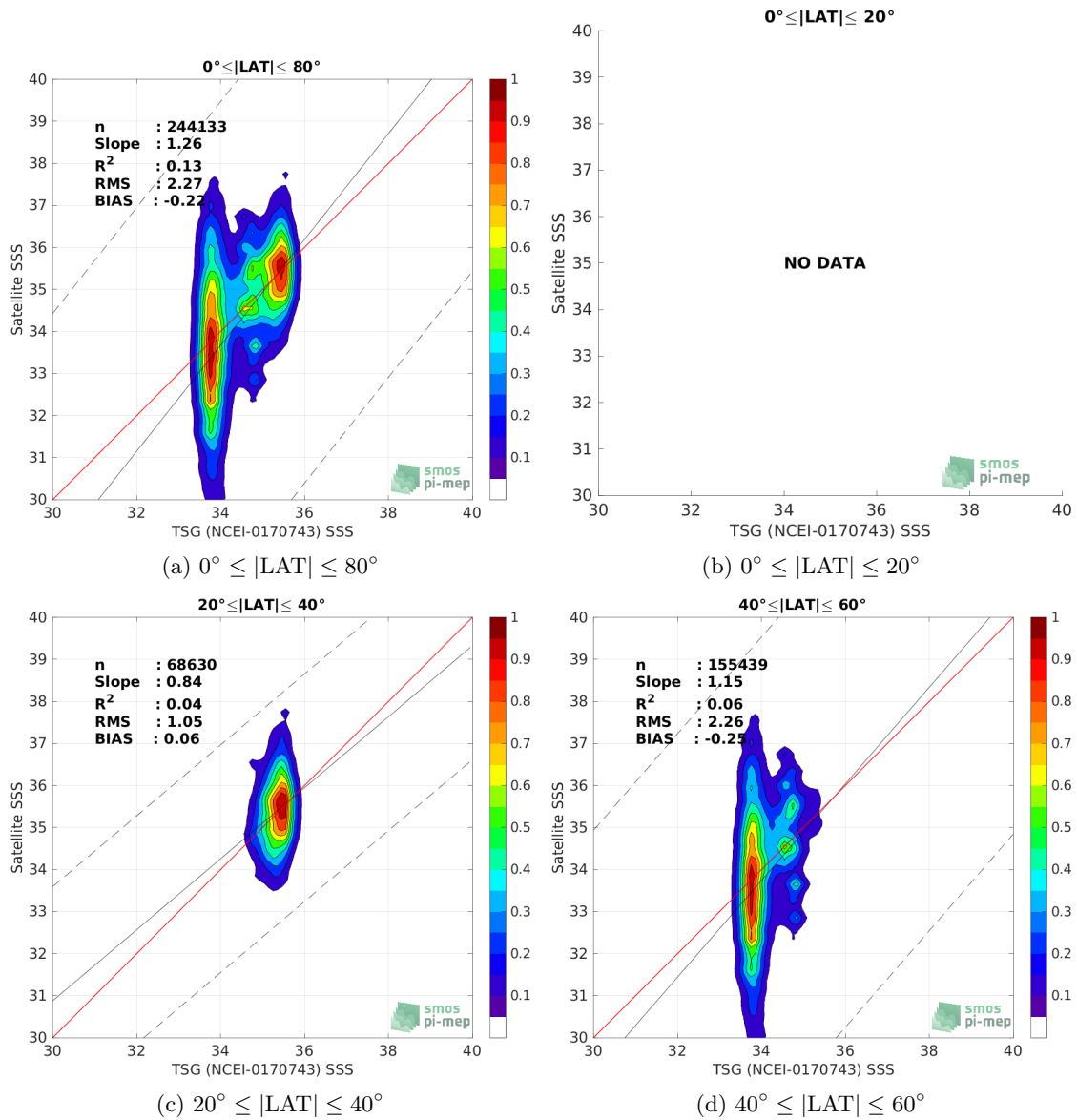
Figure 9: Contour maps of the concentration of SMOS SSS L2Q v331 - No FLAG (CMEMS-CATDS-CPDC) SSS (y-axis) versus TSG (NCEI-0170743) SSS (x-axis) at match-up pairs for different latitude bands. For each plot, the red line shows x=y . The black thin and dashed lines indicate a linear fit through the data cloud and the \pm 95\% confidence levels, respectively. The number match-up pairs n , the slope and R^2 coefficient of the linear fit, the root mean square (RMS) and the mean bias between satellite and in situ data are indicated for each latitude band in each plots.
