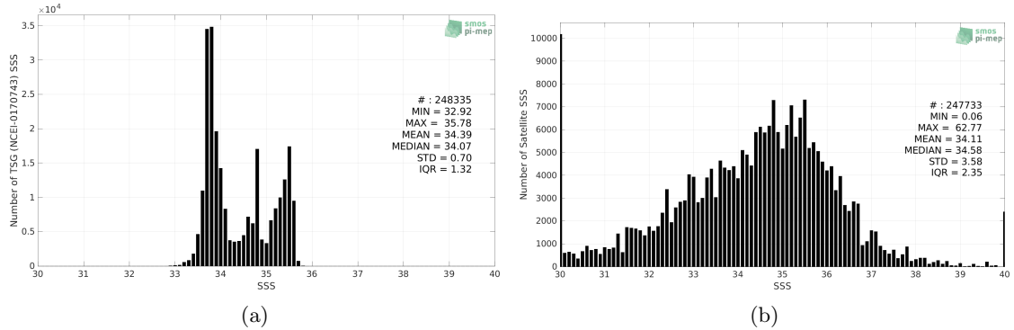
Figure 2: Histograms of SSS from TSG (NCEI-0170743) (a) and SMOS SSS L2Q v331 - No FLAG (CMEMS-CATDS-CPDC) (b) considering all match-up pairs per bins of 0.1 over the Global Ocean Pi-MEP region and for the full satellite product period.
