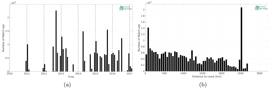
Figure 1: Number of match-ups between TSG (NCEI-0170743) and SMOS SSS L2Q v331 - No FLAG (CMEMS-CATDS-CPDC) SSS as a function of time (a) and as function of the distance to coast (b) over the Global Ocean Pi-MEP region and for the full satellite product period.
