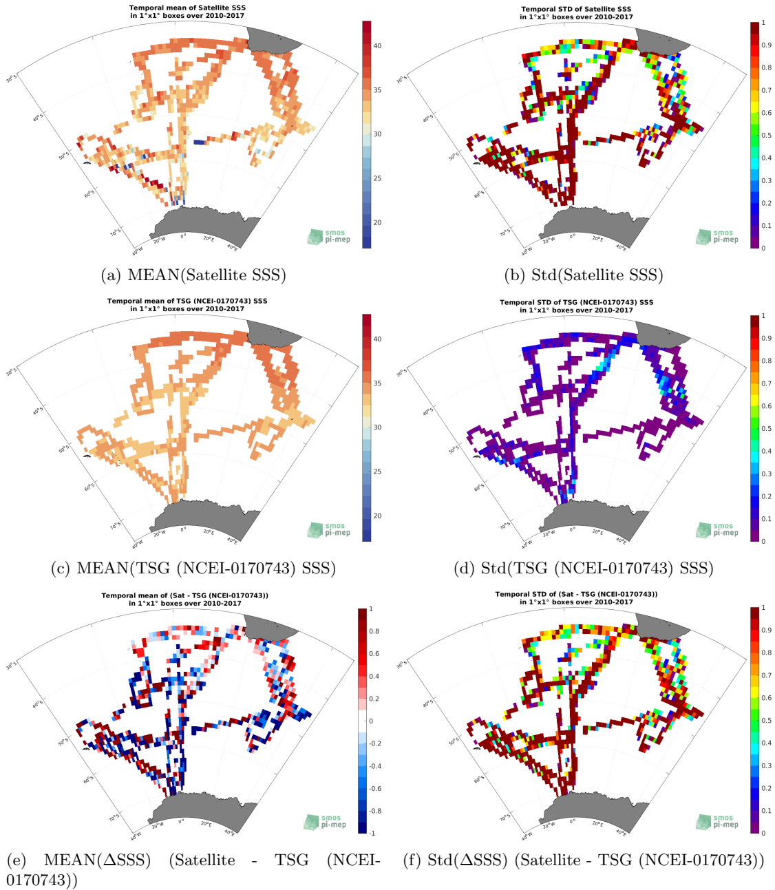
Figure 6: Temporal mean (left) and Std (right) of SSS from SMOS SSS L2Q v331 - No FLAG (CMEMS-CATDS-CPDC) (top), TSG (NCEI-0170743) (middle), and of \Delta SSS (Satellite - TSG (NCEI-0170743)). Only match-up pairs are used to generate these maps.
