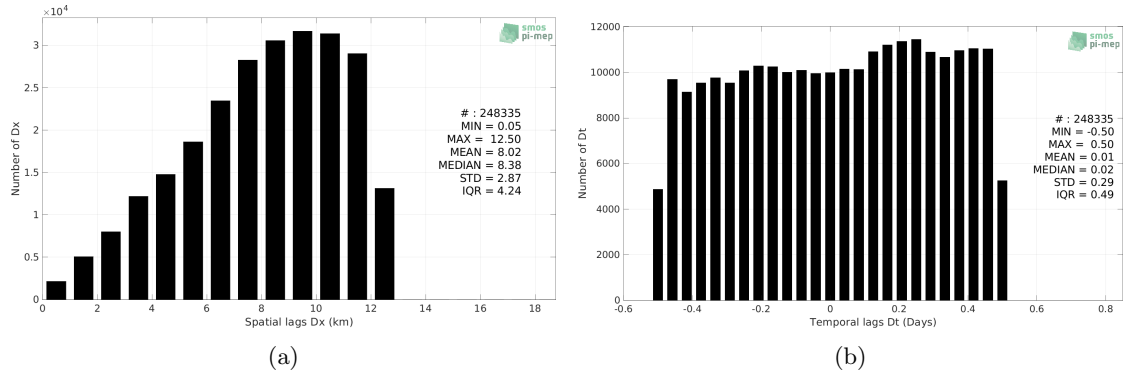
Figure 5: Histograms of the spatial (a) and temporal (b) lags between the location/time of the TSG (NCEI-0170743) measurement and the date of the corresponding SMOS SSS L2Q v331 - No FLAG (CMEMS-CATDS-CPDC) SSS pixel.
