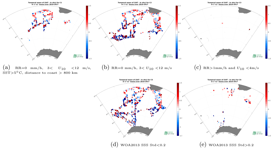
Figure 12: Temporal mean gridded over spatial boxes of size 1^{\circ}\times 1^{\circ} of \Delta\text{SSS} (SMOS SSS L2Q v331 - No FLAG (CMEMS-CATDS-CPDC) - TSG (NCEI-0170743)) for 5 different subdatasets corresponding to:RR=0 mm/h, 3 < U_{10} < 12 m/s, SST >5^{\circ}\text{C} , distance to coast > 800 km (a), RR=0 mm/h, 3 < U_{10} < 12 m/s (b), RR >1 mm/h and U_{10} < 4 m/s (c), WOA2013 SSS Std <0.2 (d), WOA2013 SSS Std >0.2 (e).
