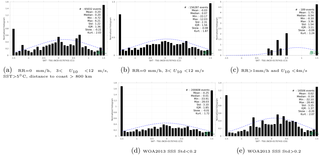
Figure 13: Normalized histogram of \Delta SSS (SMOS SSS L2Q v331 - No FLAG (CMEMS-CATDS-CPDC) - TSG (NCEI-0170743)) for 5 different subdatasets corresponding to: RR=0 mm/h, 3 < U_{10} < 12 m/s, SST > 5°C, distance to coast > 800 km (a), RR=0 mm/h, 3 < U_{10} < 12 m/s (b), RR > 1mm/h and U_{10} < 4 m/s (c), WOA2013 SSS Std < 0.2 (d), WOA2013 SSS Std > 0.2 (e).
