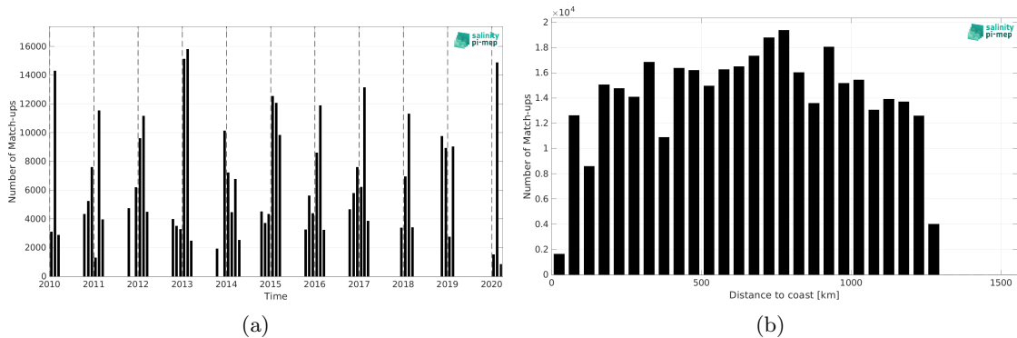
Figure 2: Number of match-ups between TSG (LEGOS-Survostral) and SMOS SSS L2Q v331 - No FLAG (CMEMS-CATDS-CPDC) SSS as a function of time (a) and as function of the distance to coast (b) over the Global Ocean Pi-MEP region and for the full satellite product period.
