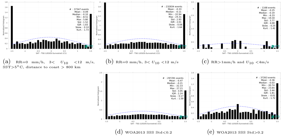
Figure 15: Normalized histogram of \Delta SSS (SMOS SSS L2Q v331 - No FLAG (CMEMS-CATDS-CPDC) - TSG (LEGOs-Survostral)) for 5 different subdatasets corresponding to: RR=0 mm/h, 3 < U_{10} < 12 m/s, SST > 5°C, distance to coast > 800 km (a), RR=0 mm/h, 3 < U_{10} < 12 m/s (b), RR > 1mm/h and U_{10} < 4 m/s (c), WOA2013 SSS Std < 0.2 (d), WOA2013 SSS Std > 0.2 (e).
