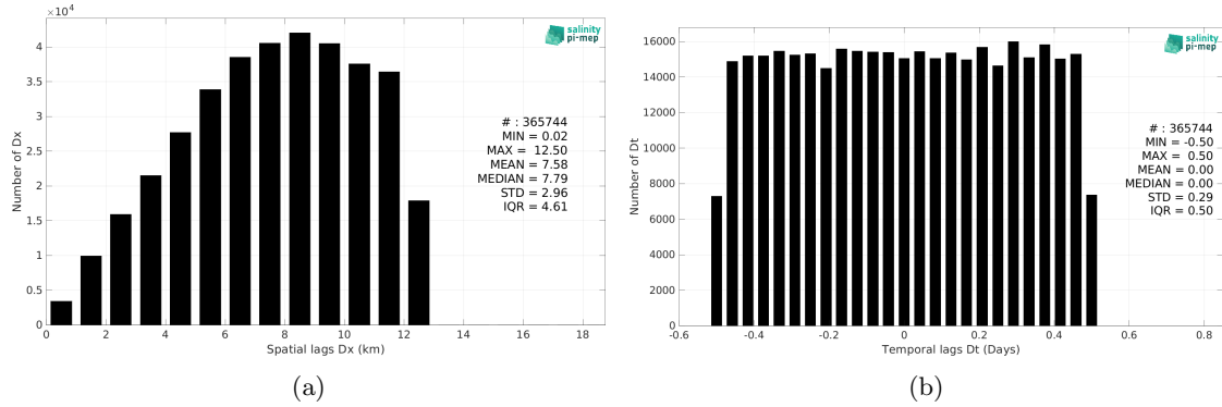
Figure 6: Histograms of the spatial (a) and temporal (b) lags between the location/time of the TSG (LEGOS-Survostral) measurement and the date of the corresponding SMOS SSS L2Q v331 - No FLAG (CMEMS-CATDS-CPDC) SSS pixel.
