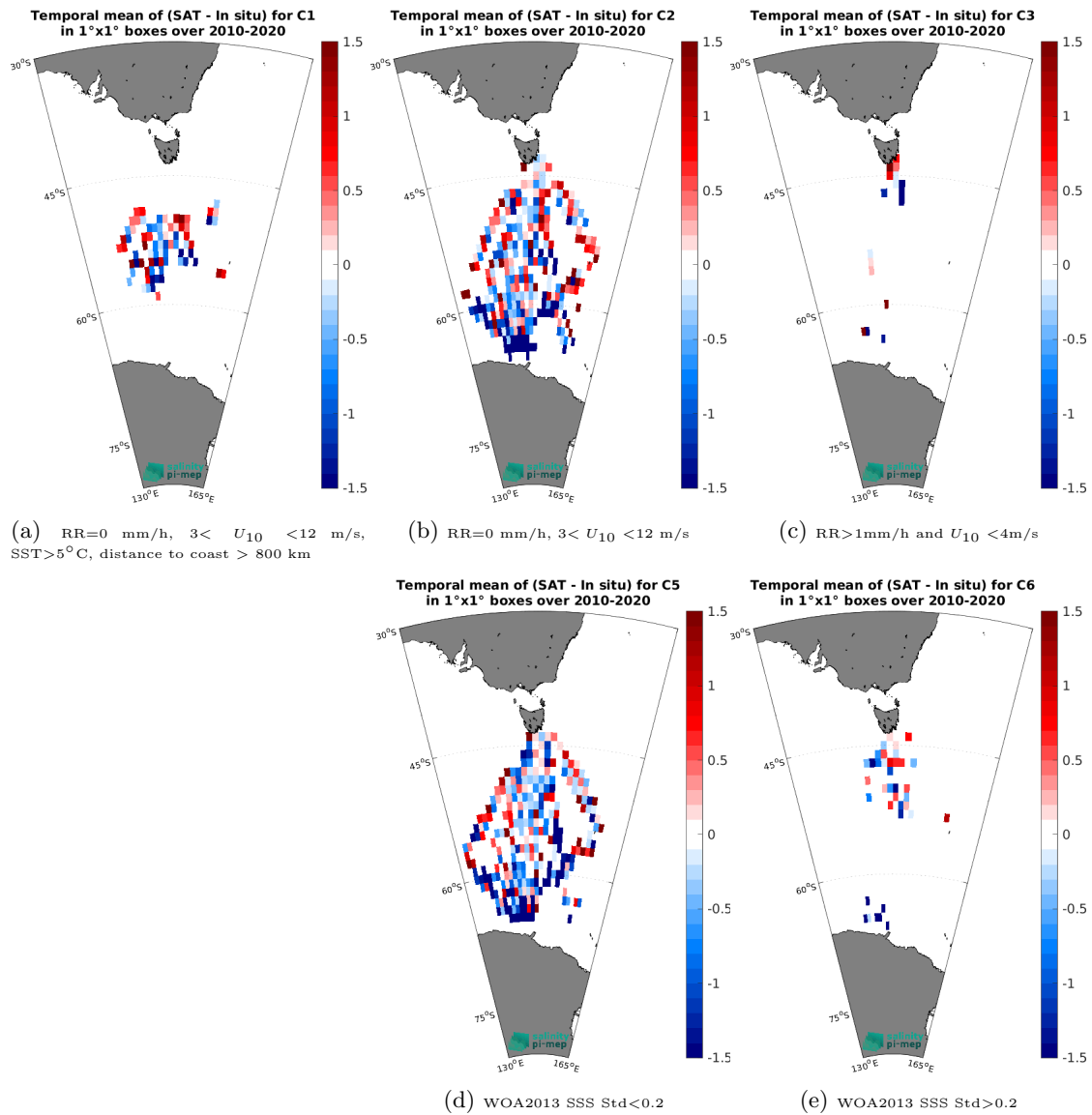
Figure 14: Temporal mean gridded over spatial boxes of size 1^\circ \times 1^\circ of \Delta\text{SSS} (SMOS SSS L2Q v331 - No FLAG (CMEMS-CATDS-CPDC) - TSG (LEGOS-Survostral)) for 5 different sub-datasets corresponding to: RR=0 mm/h, 3 < U_{10} < 12 m/s, SST > 5^\circ\text{C} , distance to coast > 800 km (a), RR=0 mm/h, 3 < U_{10} < 12 m/s (b), RR > 1 mm/h and U_{10} < 4 m/s (c), WOA2013 SSS Std < 0.2 (d), WOA2013 SSS Std > 0.2 (e).
