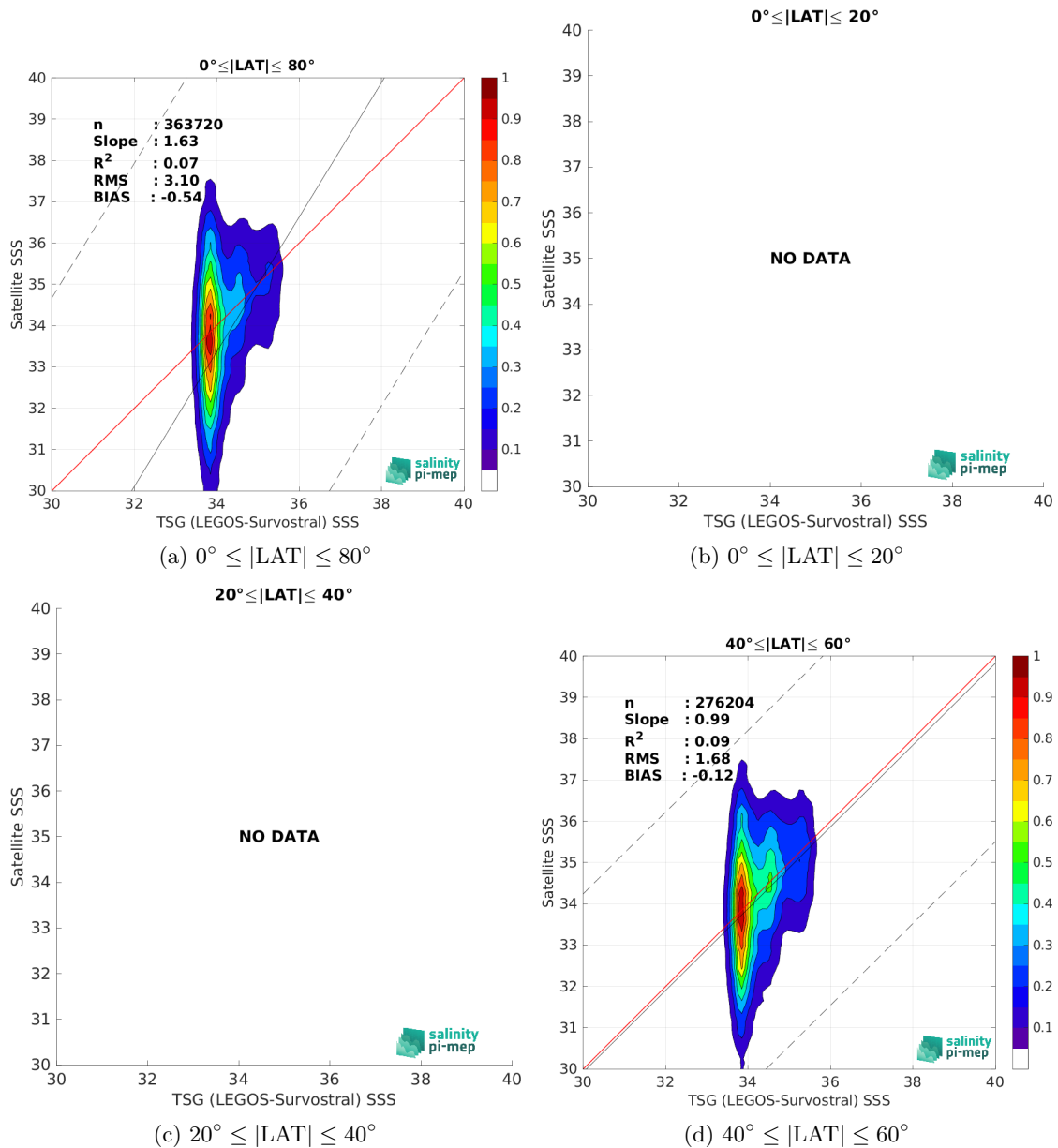
Figure 10: Contour maps of the concentration of SMOS SSS L2Q v331 - No FLAG (CMEMS-CATDS-CPDC) SSS (y-axis) versus TSG (LEGOS-Survostral) SSS (x-axis) at match-up pairs for different latitude bands. For each plot, the red line shows x=y . The black thin and dashed lines indicate a linear fit through the data cloud and the \pm 95\% confidence levels, respectively. The number match-up pairs n , the slope and R^2 coefficient of the linear fit, the root mean square (RMS) and the mean bias between satellite and in situ data are indicated for each latitude band in each plots.
