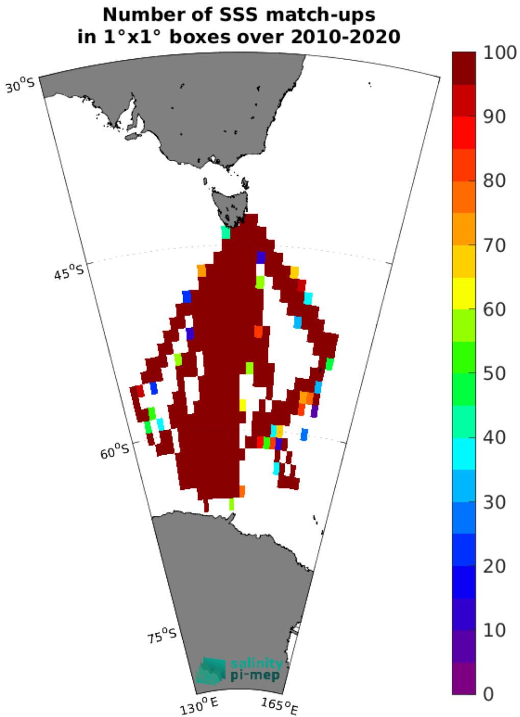
Figure 5: Number of SSS match-ups between TSG (LEGOS-Survostral) SSS and the SMOS SSS L2Q v331 - No FLAG (CMEMS-CATDS-CPDC) SSS product for the Global Ocean Pi-MEP region over 1°x1° boxes and for the full satellite product period.
