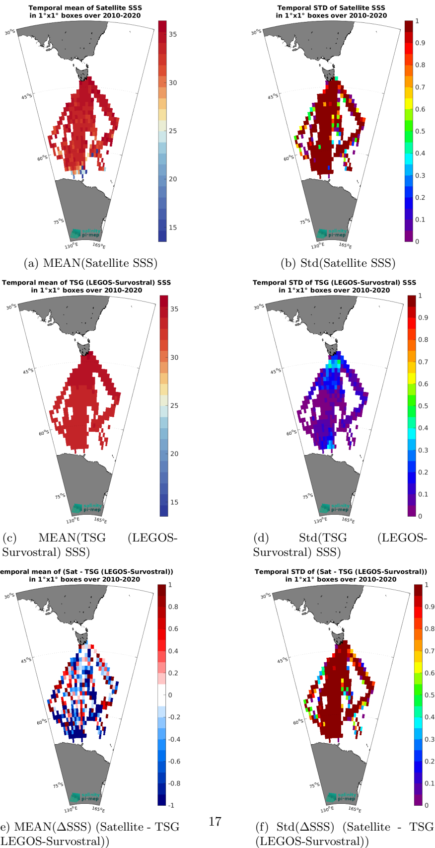
Figure 7: Temporal mean (left) and Std (right) of SSS from SMOS SSS L2Q v331 - No FLAG (CMEMS-CATDS-CPDC) (top), TSG (LEGOS-Survostral) (middle), and of \Delta SSS (Satellite - TSG (LEGOS-Survostral)). Only match-up pairs are used to generate these maps.
