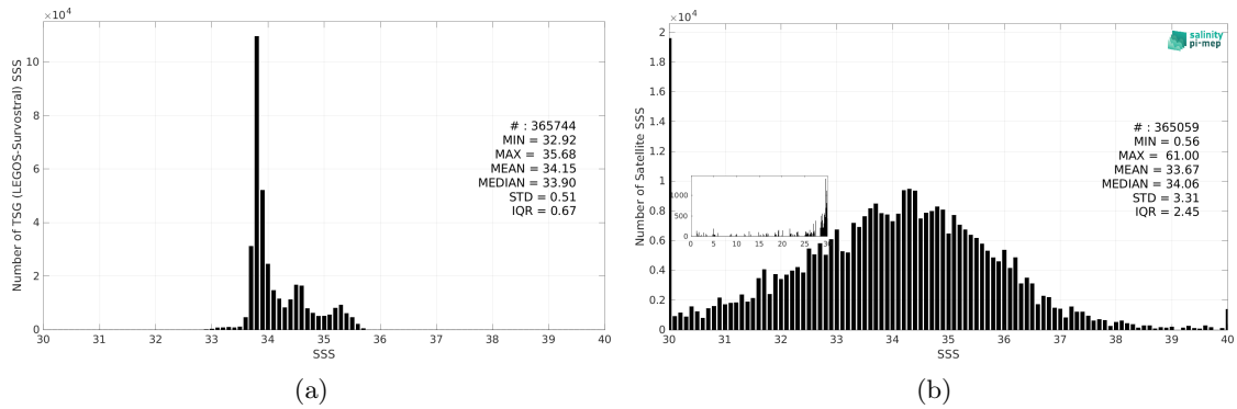
Figure 3: Histograms of SSS from TSG (LEGOS-Survostral) (a) and SMOS SSS L2Q v331 - No FLAG (CMEMS-CATDS-CPDC) (b) considering all match-up pairs per bins of 0.1 over the Global Ocean Pi-MEP region and for the full satellite product period.
