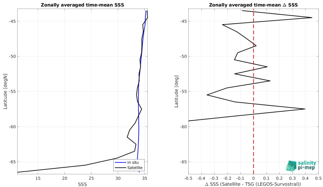
Figure 9: Left panel: Zonal mean SSS from SMOS SSS L2Q v331 - No FLAG (CMEMS-CATDS-CPDC) satellite product (black) and from TSG (LEGOS-Survostral) (blue). Right panel: Zonal mean of \Delta SSS (Satellite - TSG (LEGOS-Survostral)) for all the collected Pi-MEP match-up pairs estimated over the full satellite product period.
