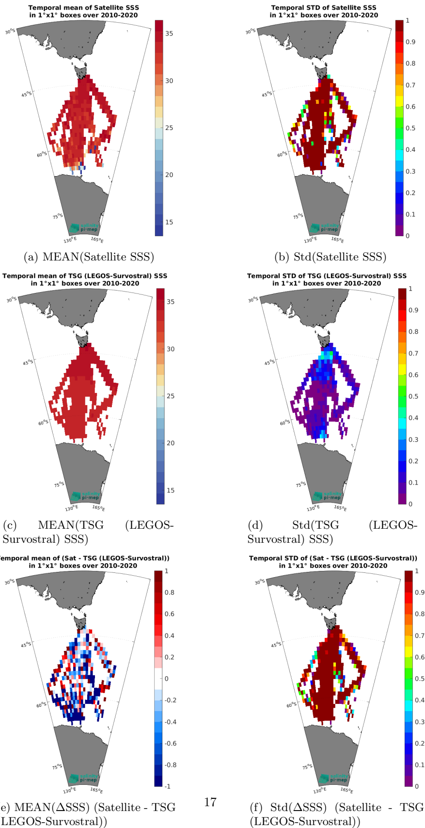
Figure 6: Temporal mean (left) and Std (right) of SSS from SMOS SSS L2Q v331 - No FLAG (CMEMS-CATDS-CPDC) (top), TSG (LEGOS-Survostral) (middle), and of \Delta SSS (Satellite - TSG (LEGOS-Survostral)). Only match-up pairs are used to generate these maps.
