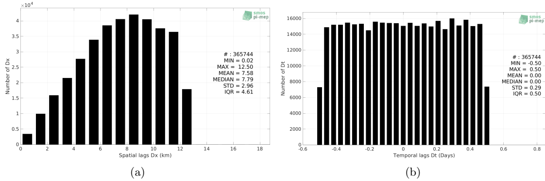
Figure 5: Histograms of the spatial (a) and temporal (b) lags between the location/time of the TSG (LEGOS-Survostral) measurement and the date of the corresponding SMOS SSS L2Q v331 - No FLAG (CMEMS-CATDS-CPDC) SSS pixel.
