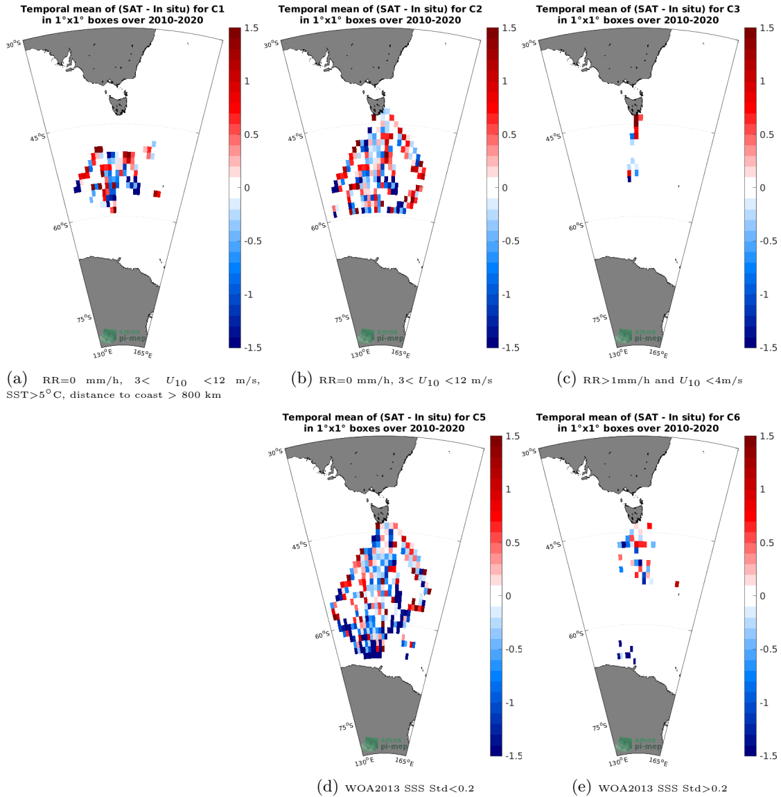
Figure 12: Temporal mean gridded over spatial boxes of size 1^\circ \times 1^\circ of \Delta SSS (SMOS SSS L2Q v331 - No FLAG (CMEMS-CATDS-CPDC) - TSG (LEGOS-Survostral)) for 5 different sub-datasets corresponding to:RR=0 mm/h, 3 < U_{10} < 12 m/s, SST>5°C, distance to coast > 800 km (a), RR=0 mm/h, 3 < U_{10} < 12 m/s (b), RR>1mm/h and U_{10} < 4 m/s (c), WOA2013 SSS Std<0.2 (d), WOA2013 SSS Std>0.2 (e).
