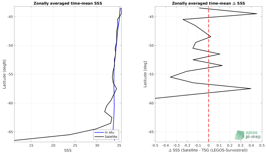
Figure 8: Left panel: Zonal mean SSS from SMOS SSS L2Q v331 - No FLAG (CMEMS-CATDS-CPDC) satellite product (black) and from TSG (LEGOS-Survostral) (blue). Right panel: Zonal mean of \Delta SSS (Satellite - TSG (LEGOS-Survostral)) for all the collected Pi-MEP match-up pairs estimated over the full satellite product period.
