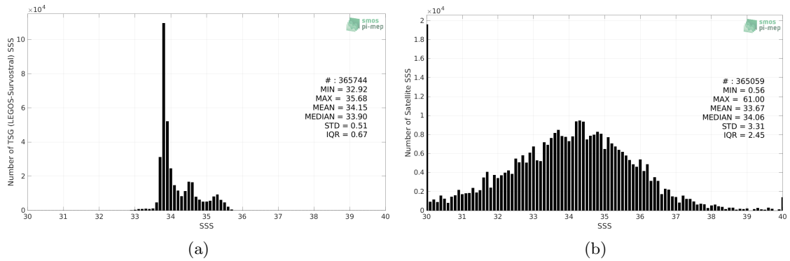
Figure 2: Histograms of SSS from TSG (LEGOS-Survostral) (a) and SMOS SSS L2Q v331 - No FLAG (CMEMS-CATDS-CPDC) (b) considering all match-up pairs per bins of 0.1 over the Global Ocean Pi-MEP region and for the full satellite product period.
