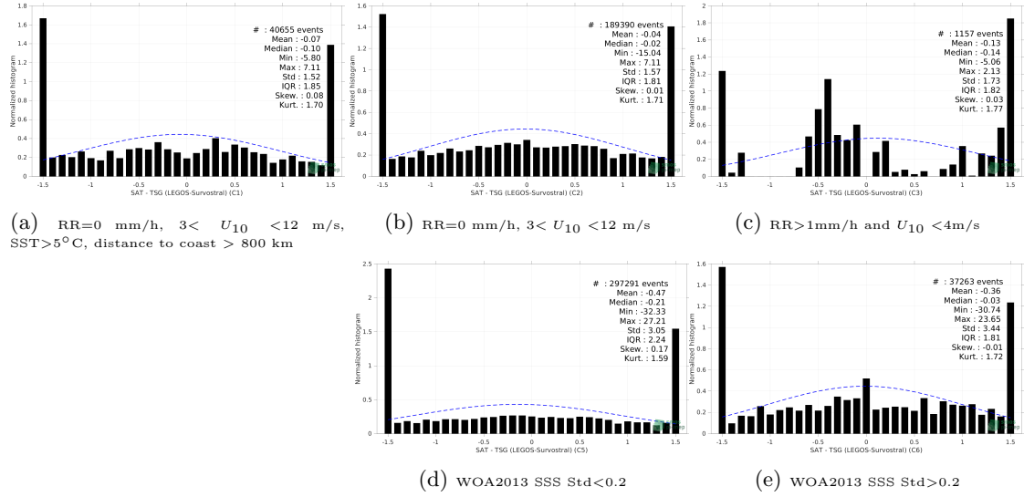
Figure 13: Normalized histogram of \Delta SSS (SMOS SSS L2Q v331 - No FLAG (CMEMS-CATDS-CPDC) - TSG (LEGOs-Survostral)) for 5 different subdatasets corresponding to: RR=0 mm/h, 3 < U_{10} < 12 m/s, SST>5°C, distance to coast > 800 km (a), RR=0 mm/h, 3 < U_{10} < 12 m/s (b), RR>1mm/h and U_{10} < 4 m/s (c), WOA2013 SSS Std<0.2 (d), WOA2013 SSS Std>0.2 (e).
