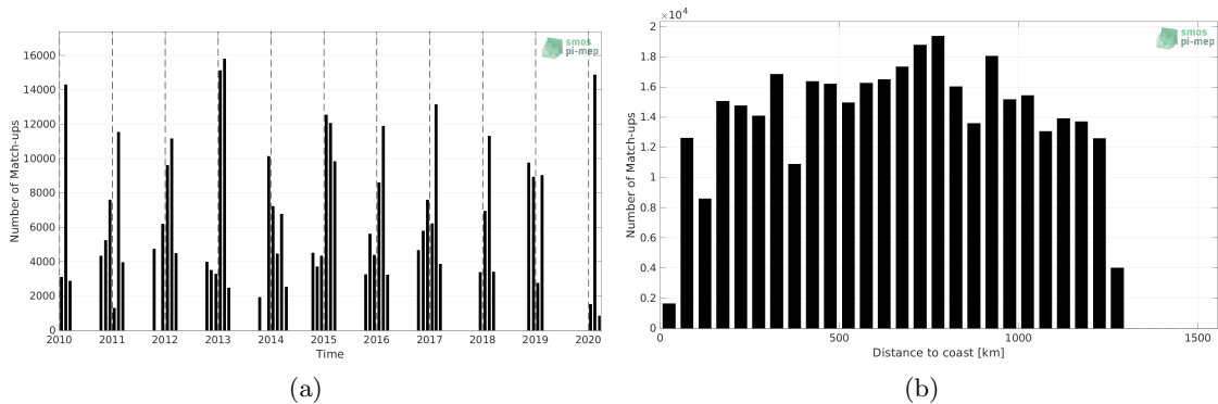
Figure 1: Number of match-ups between TSG (LEGOS-Survostral) and SMOS SSS L2Q v331 - No FLAG (CMEMS-CATDS-CPDC) SSS as a function of time (a) and as function of the distance to coast (b) over the Global Ocean Pi-MEP region and for the full satellite product period.
