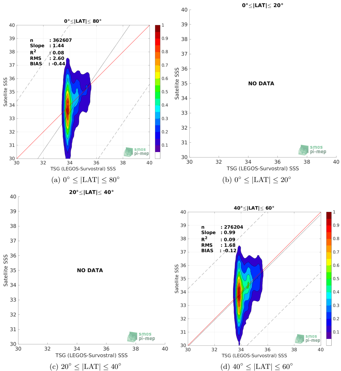
Figure 9: Contour maps of the concentration of SMOS SSS L2Q v331 - No FLAG (CMEMS-CATDS-CPDC) SSS (y-axis) versus TSG (LEGOS-Survostral) SSS (x-axis) at match-up pairs for different latitude bands. For each plot, the red line shows x=y . The black thin and dashed lines indicate a linear fit through the data cloud and the \pm 95\% confidence levels, respectively. The number match-up pairs n , the slope and R^2 coefficient of the linear fit, the root mean square (RMS) and the mean bias between satellite and in situ data are indicated for each latitude band in each plots.
