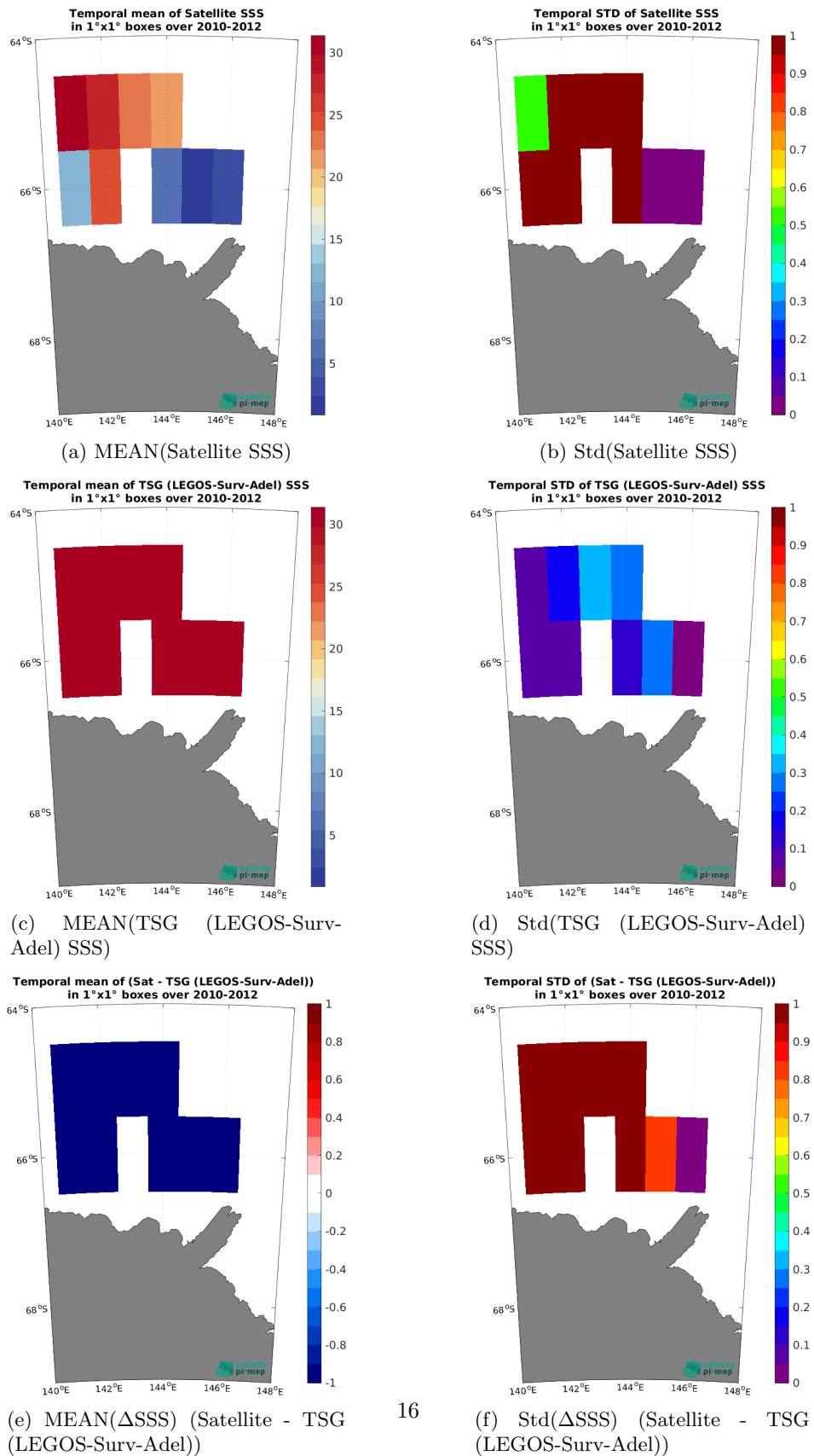
Figure 6: Temporal mean (left) and Std (right) of SSS from SMOS SSS L2Q v331 - No FLAG (CMEMS-CATDS-CPDC) (top), TSG (LEGOS-Surv-Adel) (middle), and of \Delta SSS (Satellite - TSG (LEGOS-Surv-Adel)). Only match-up pairs are used to generate these maps.
