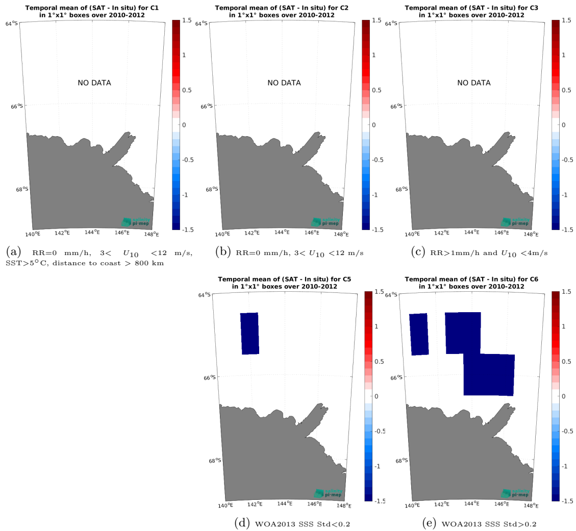
Figure 12: Temporal mean gridded over spatial boxes of size 1^{\circ} \times 1^{\circ} of \Delta SSS (SMOS SSS L2Q v331 - No FLAG (CMEMS-CATDS-CPDC) - TSG (LEGOS-Surv-Adel)) for 5 different sub-datasets corresponding to: RR=0 mm/h, 3 < U_{10} < 12 m/s, SST>5°C, distance to coast > 800 km (a), RR=0 mm/h, 3 < U_{10} < 12 m/s (b), RR>1mm/h and U_{10} < 4 m/s (c), WOA2013 SSS Std<0.2 (d), WOA2013 SSS Std>0.2 (e).
