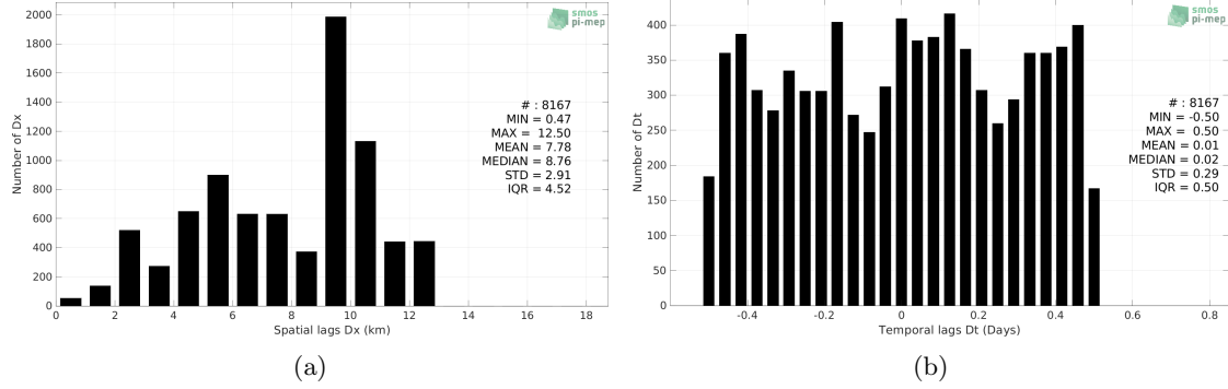
Figure 5: Histograms of the spatial (a) and temporal (b) lags between the location/time of the TSG (LEGOS-Surv-Adel) measurement and the date of the corresponding SMOS SSS L2Q v331 - No FLAG (CMEMS-CATDS-CPDC) SSS pixel.
