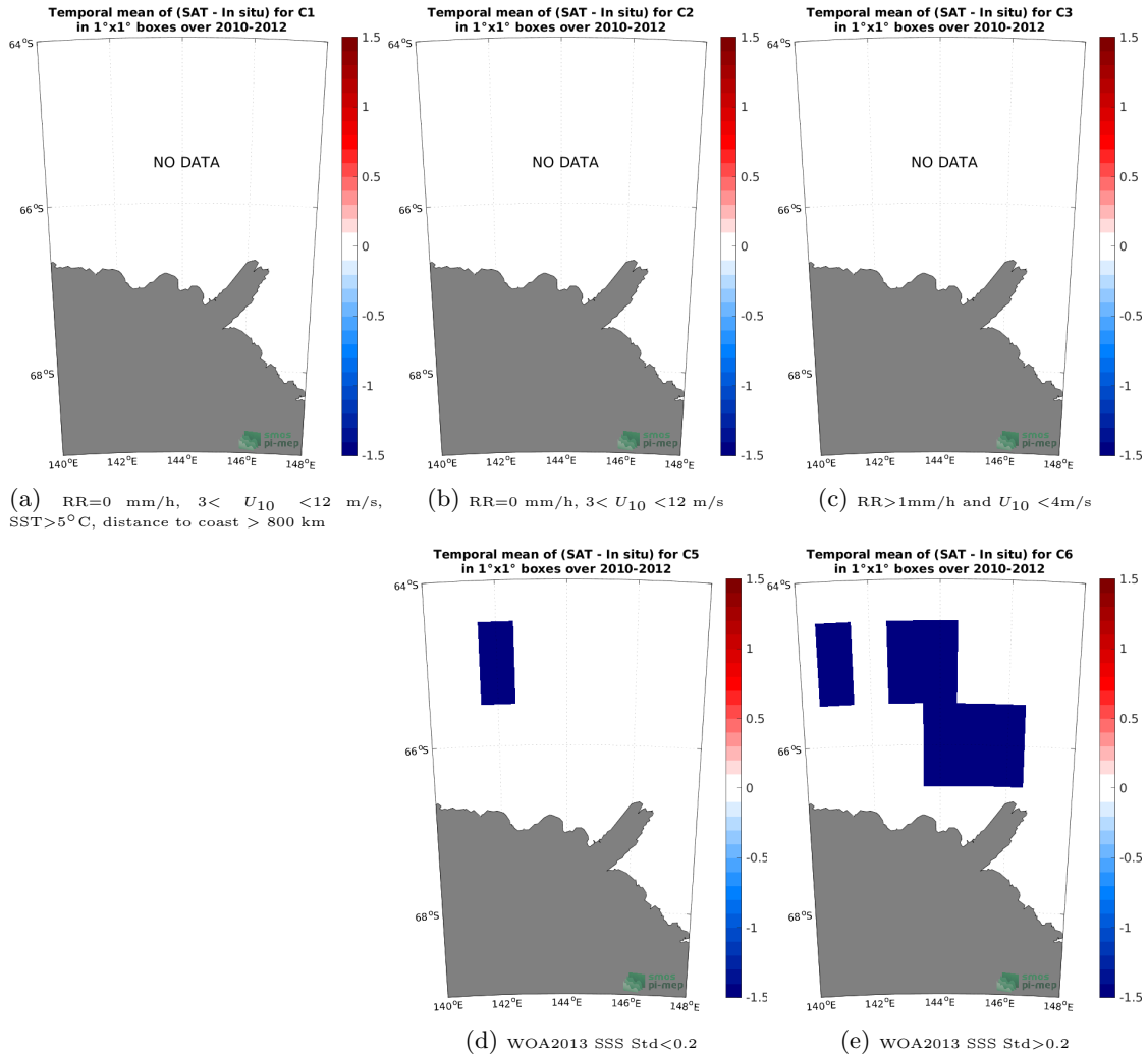
Figure 12: Temporal mean gridded over spatial boxes of size 1^\circ \times 1^\circ of \Delta SSS (SMOS SSS L2Q v331 - No FLAG (CMEMS-CATDS-CPDC) - TSG (LEGOS-Surv-Adel)) for 5 different sub-datasets corresponding to:RR=0 mm/h, 3 < U_{10} < 12 m/s, SST>5°C, distance to coast > 800 km (a), RR=0 mm/h, 3 < U_{10} < 12 m/s (b), RR>1mm/h and U_{10} < 4 m/s (c), WOA2013 SSS Std<0.2 (d), WOA2013 SSS Std>0.2 (e).
