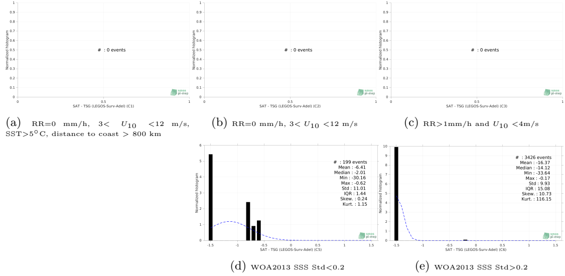
Figure 13: Normalized histogram of \Delta SSS (SMOS SSS L2Q v331 - No FLAG (CMEMS-CATDS-CPDC) - TSG (LEGOS-Surv-Adel)) for 5 different subdatasets corresponding to: RR=0 mm/h, 3 < U_{10} < 12 m/s, SST>5°C, distance to coast > 800 km (a), RR=0 mm/h, 3 < U_{10} < 12 m/s (b), RR>1mm/h and U_{10} < 4 m/s (c), WOA2013 SSS Std<0.2 (d), WOA2013 SSS Std>0.2 (e).
