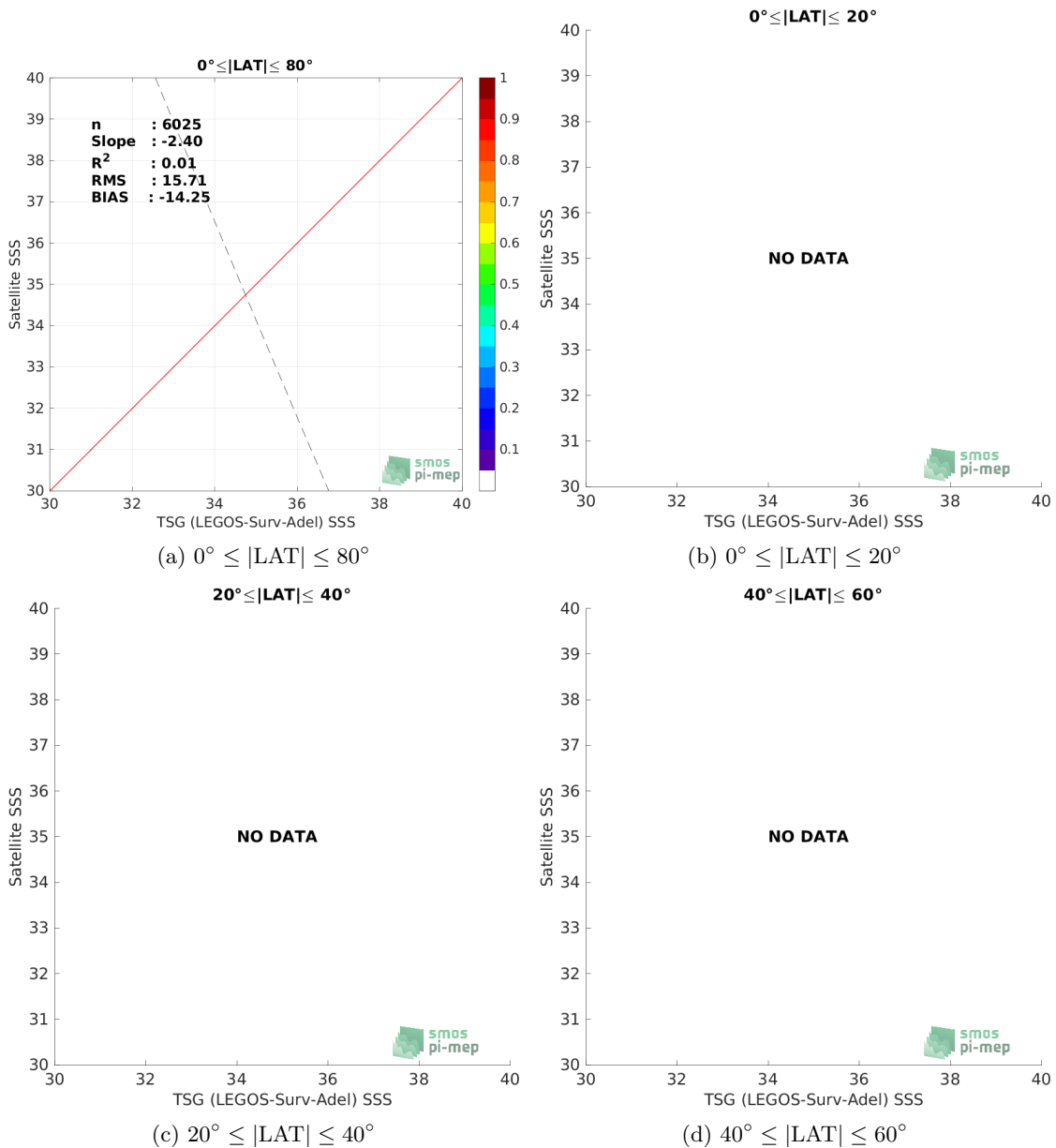
Figure 9: Contour maps of the concentration of SMOS SSS L2Q v331 - No FLAG (CMEMS-CATDS-CPDC) SSS (y-axis) versus TSG (LEGOS-Surv-Adel) SSS (x-axis) at match-up pairs for different latitude bands. For each plot, the red line shows x=y . The black thin and dashed lines indicate a linear fit through the data cloud and the \pm 95\% confidence levels, respectively. The number match-up pairs n , the slope and R^2 coefficient of the linear fit, the root mean square (RMS) and the mean bias between satellite and in situ data are indicated for each latitude band in each plots.
