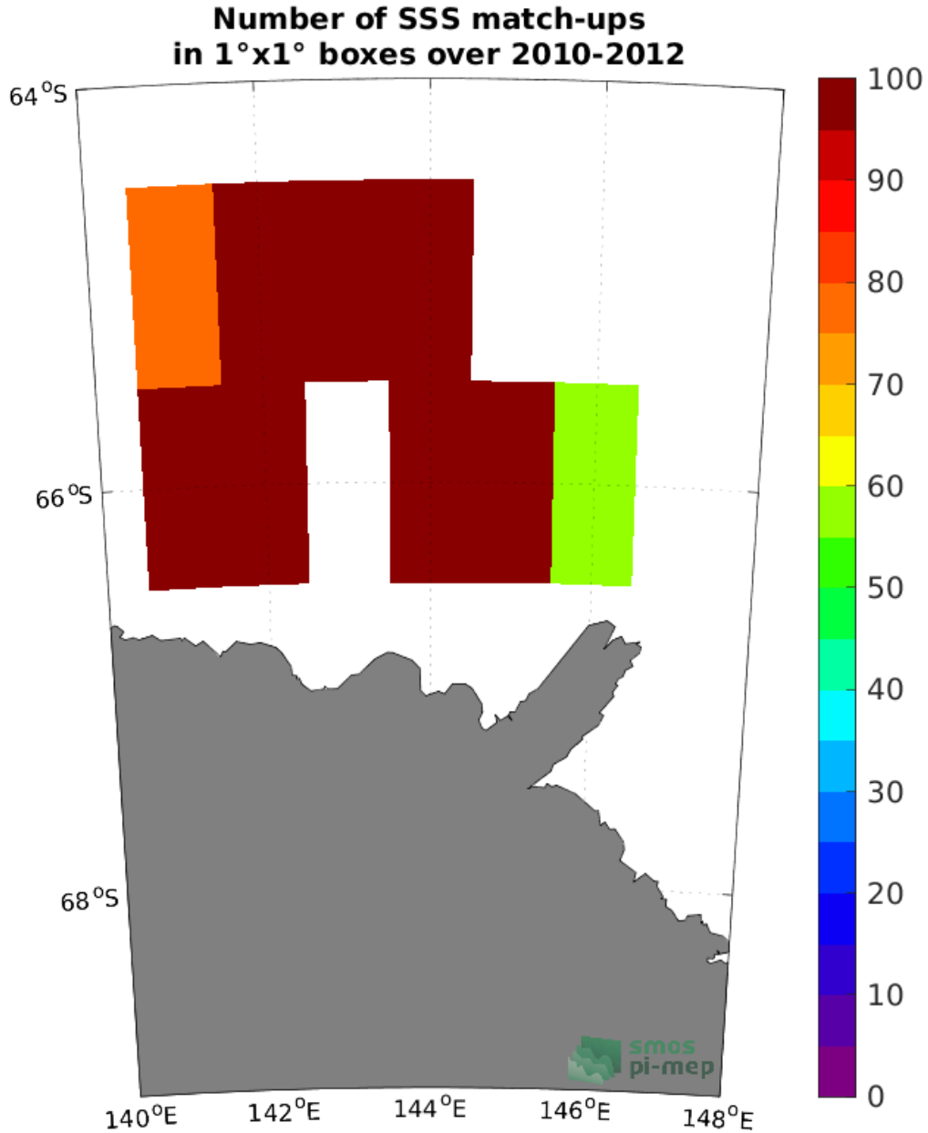
Figure 4: Number of SSS match-ups between TSG (LEGOS-Surv-Adel) SSS and the SMOS SSS L2Q v331 - No FLAG (CMEMS-CATDS-CPDC) SSS product for the Global Ocean Pi-MEP region over 1^\circ \times 1^\circ boxes and for the full satellite product period.
