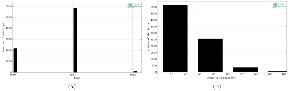
Figure 1: Number of match-ups between TSG (LEGOS-Surv-Adel) and SMOS SSS L2Q v331 - No FLAG (CMEMS-CATDS-CPDC) SSS as a function of time (a) and as function of the distance to coast (b) over the Global Ocean Pi-MEP region and for the full satellite product period.
