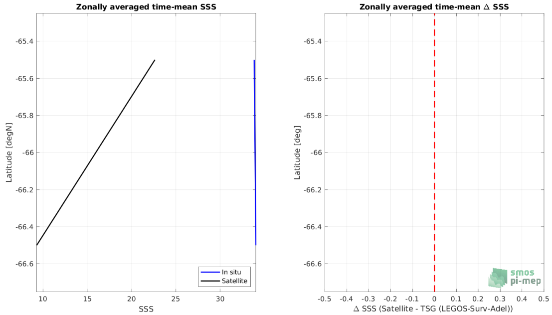
Figure 8: Left panel: Zonal mean SSS from SMOS SSS L2Q v331 - No FLAG (CMEMS-CATDS-CPDC) satellite product (black) and from TSG (LEGOS-Surv-Adel) (blue). Right panel: Zonal mean of \Delta SSS (Satellite - TSG (LEGOS-Surv-Adel)) for all the collected Pi-MEP match-up pairs estimated over the full satellite product period.
