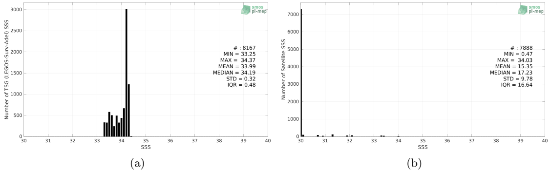
Figure 2: Histograms of SSS from TSG (LEGOS-Surv-Adel) (a) and SMOS SSS L2Q v331 - No FLAG (CMEMS-CATDS-CPDC) (b) considering all match-up pairs per bins of 0.1 over the Global Ocean Pi-MEP region and for the full satellite product period.
