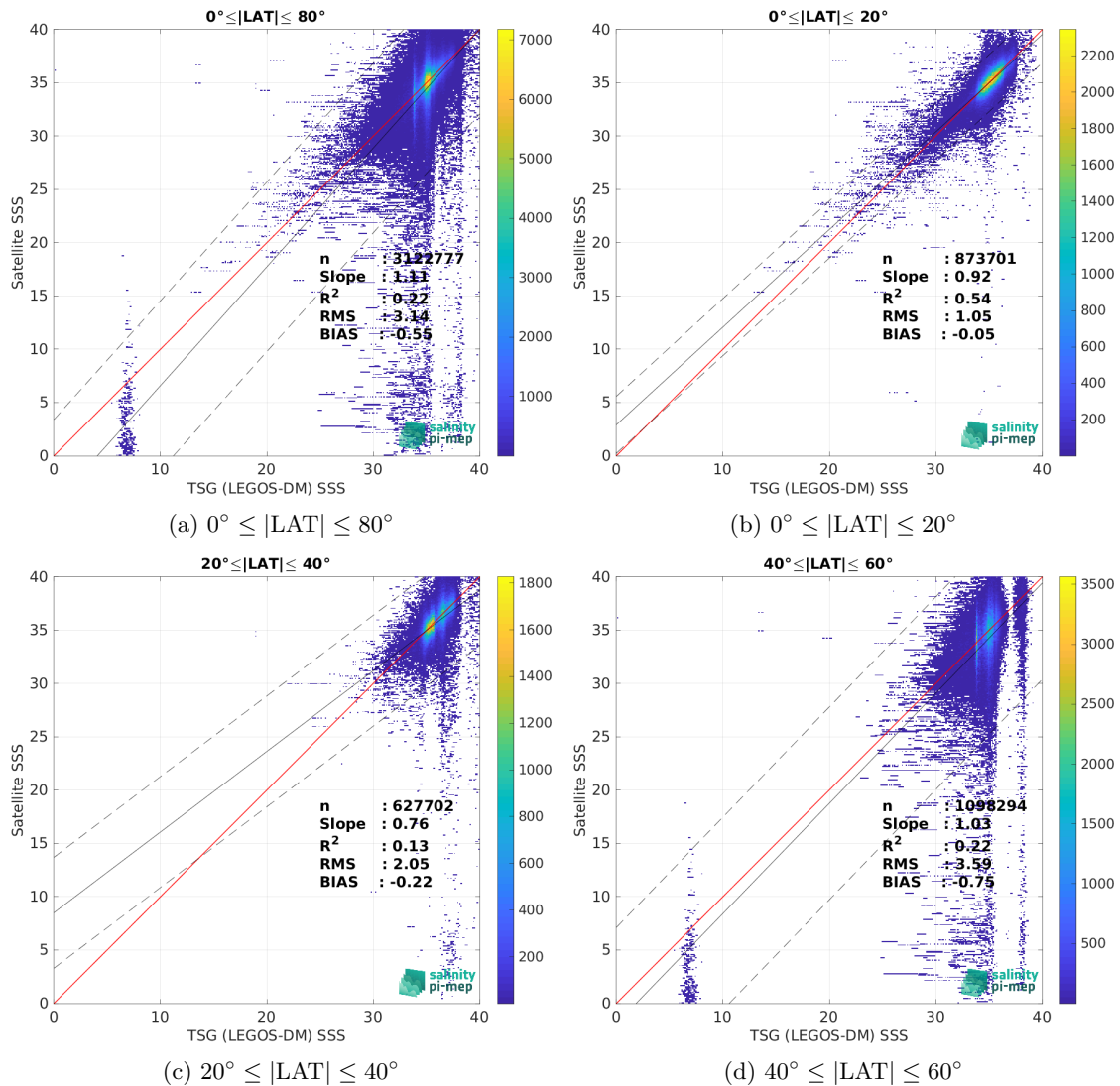
Figure 9: Contour maps of the concentration of SMOS SSS L2Q v331 - No FLAG (CMEMS-CATDS-CPDC) SSS (y-axis) versus TSG (LEGOS-DM) SSS (x-axis) at match-up pairs for different latitude bands. For each plot, the red line shows x=y . The black thin and dashed lines indicate a linear fit through the data cloud and the \pm 95\% confidence levels, respectively. The number match-up pairs n , the slope and R^2 coefficient of the linear fit, the root mean square (RMS) and the mean bias between satellite and in situ data are indicated for each latitude band in each plots.
