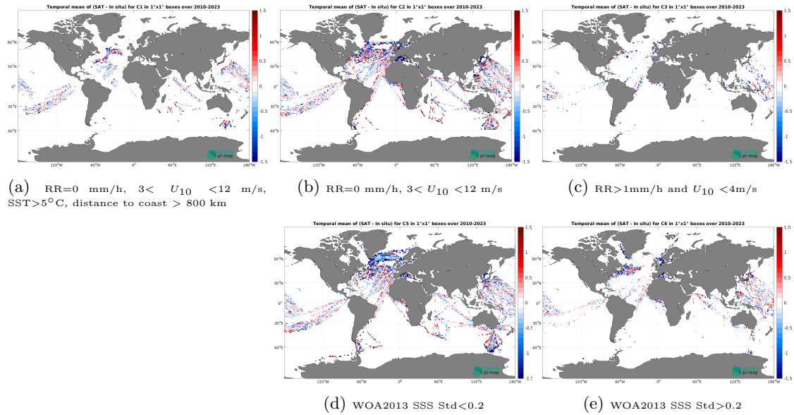
Figure 12: Temporal mean gridded over spatial boxes of size 1^\circ \times 1^\circ of \Delta\text{SSS} (SMOS SSS L2Q v331 - No FLAG (CMEMS-CATDS-CPDC) - TSG (LEGOS-DM)) for 5 different subdatasets corresponding to:RR=0 mm/h, 3 < U_{10} < 12 m/s, SST >5^\circ\text{C} , distance to coast > 800 km (a), RR=0 mm/h, 3 < U_{10} < 12 m/s (b), RR >1 mm/h and U_{10} < 4 m/s (c), WOA2013 SSS Std <0.2 (d), WOA2013 SSS Std >0.2 (e).
