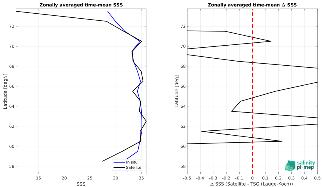
Figure 9: Left panel: Zonal mean SSS from SMOS SSS L2Q v331 - No FLAG (CMEMS-CATDS-CPDC) satellite product (black) and from TSG (Lauge-Koch) (blue). Right panel: Zonal mean of \Delta SSS (Satellite - TSG (Lauge-Koch)) for all the collected Pi-MEP match-up pairs estimated over the full satellite product period.
