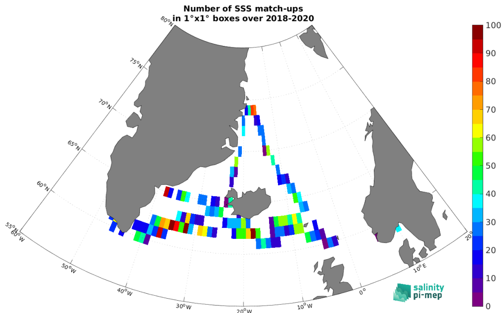
Figure 5: Number of SSS match-ups between TSG (Lauge-Koch) SSS and the SMOS SSS L2Q v331 - No FLAG (CMEMS-CATDS-CPDC) SSS product for the Global Ocean Pi-MEP region over 1^\circ \times 1^\circ boxes and for the full satellite product period.
