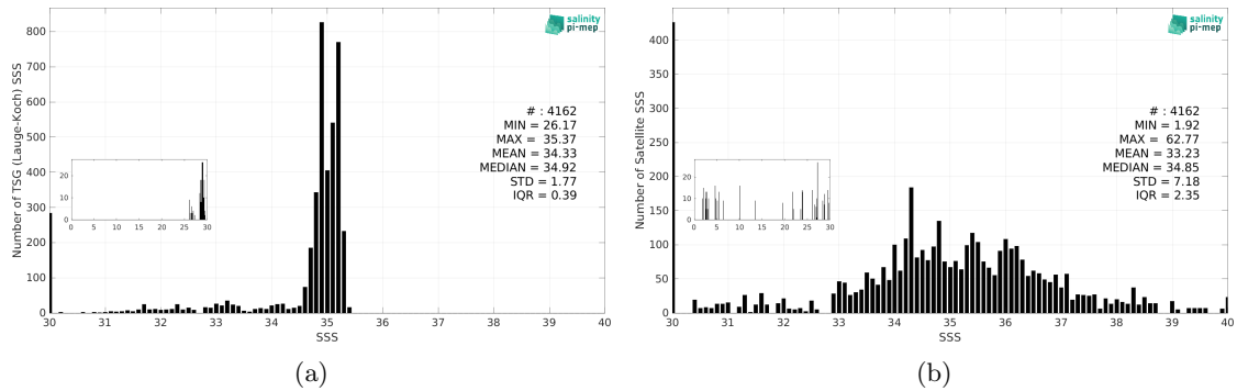
Figure 3: Histograms of SSS from TSG (Lauge-Koch) (a) and SMOS SSS L2Q v331 - No FLAG (CMEMS-CATDS-CPDC) (b) considering all match-up pairs per bins of 0.1 over the Global Ocean Pi-MEP region and for the full satellite product period.
