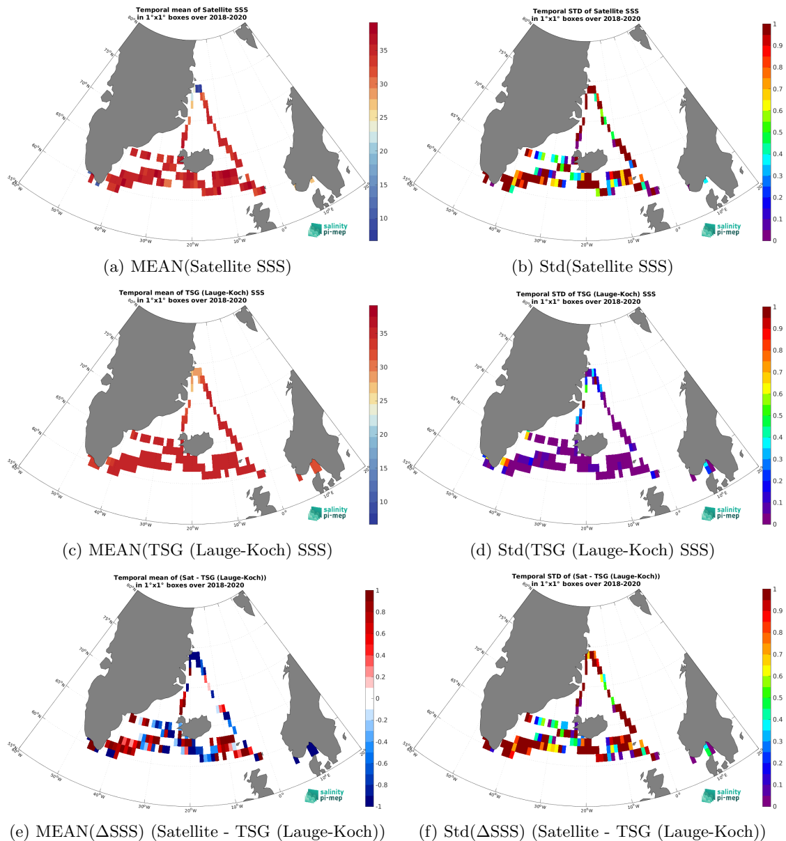
Figure 7: Temporal mean (left) and Std (right) of SSS from SMOS SSS L2Q v331 - No FLAG (CMEMS-CATDS-CPDC) (top), TSG (Lauge-Koch) (middle), and of \Delta SSS (Satellite - TSG (Lauge-Koch)). Only match-up pairs are used to generate these maps.
