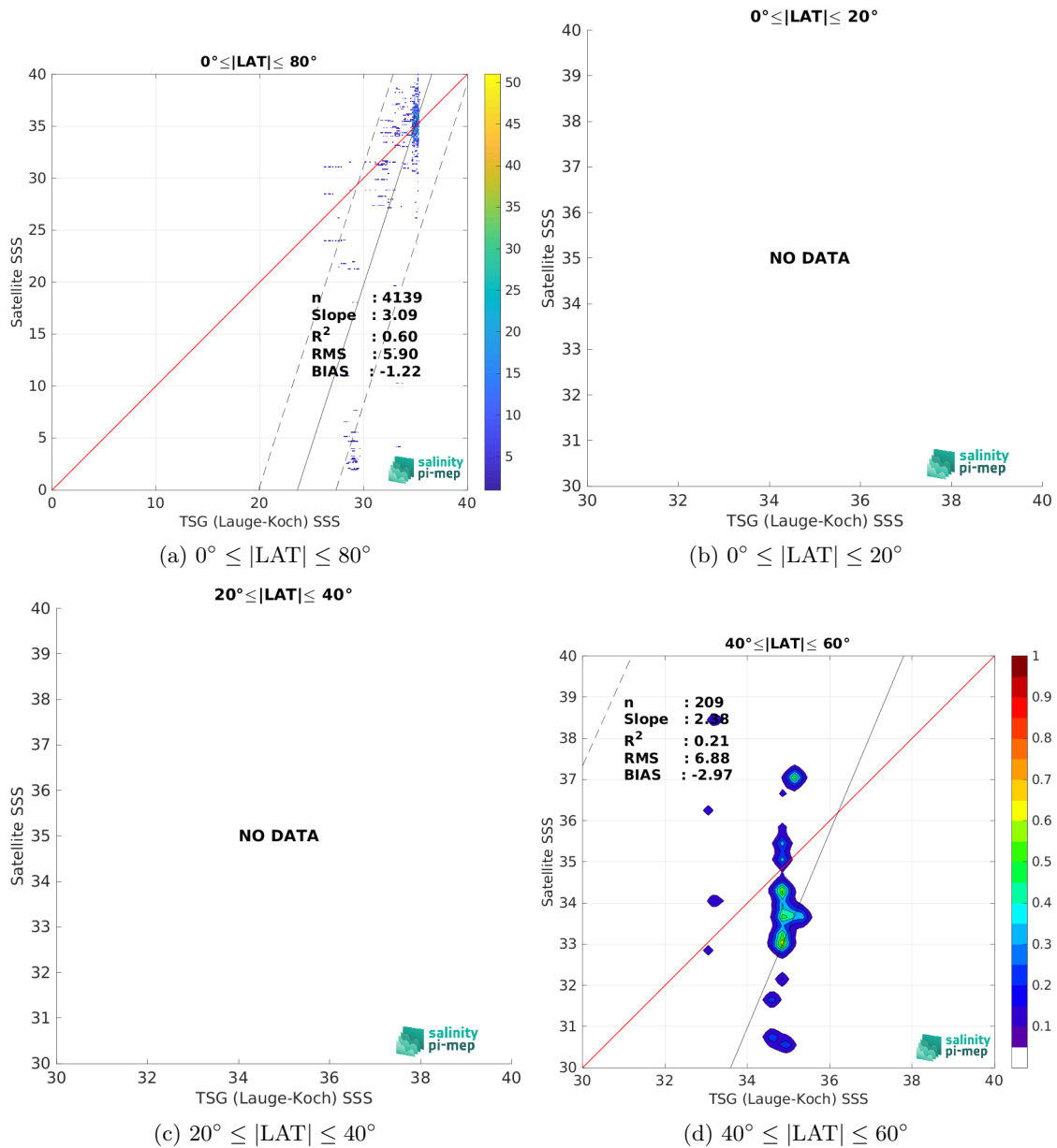
Figure 10: Contour maps of the concentration of SMOS SSS L2Q v331 - No FLAG (CMEMS-CATDS-CPDC) SSS (y-axis) versus TSG (Lauge-Koch) SSS (x-axis) at match-up pairs for different latitude bands. For each plot, the red line shows x=y . The black thin and dashed lines indicate a linear fit through the data cloud and the \pm 95\% confidence levels, respectively. The number match-up pairs n , the slope and R^2 coefficient of the linear fit, the root mean square (RMS) and the mean bias between satellite and in situ data are indicated for each latitude band in each plots.
