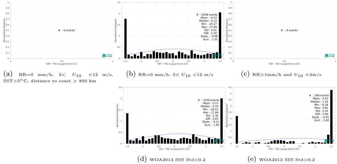
Figure 15: Normalized histogram of \Delta SSS (SMOS SSS L2Q v331 - No FLAG (CMEMS-CATDS-CPDC) - TSG (Laue-Koch)) for 5 different subdatasets corresponding to: RR=0 mm/h, 3 < U_{10} < 12 m/s, SST>5°C, distance to coast > 800 km (a), RR=0 mm/h, 3 < U_{10} < 12 m/s (b), RR>1mm/h and U_{10} < 4 m/s (c), WOA2013 SSS Std<0.2 (d), WOA2013 SSS Std>0.2 (e).
