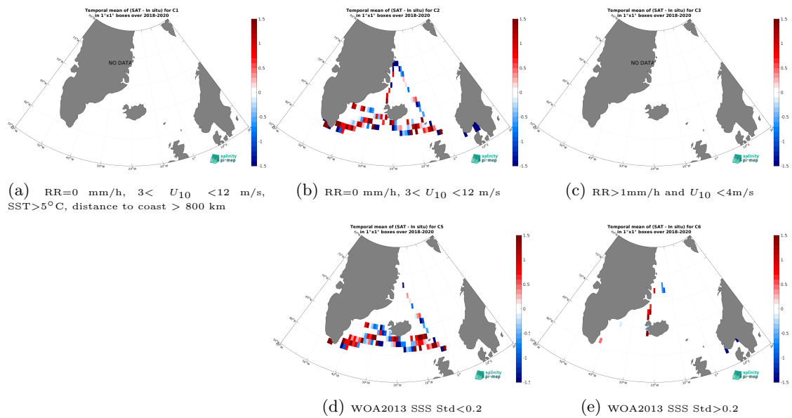
Figure 14: Temporal mean gridded over spatial boxes of size 1^\circ \times 1^\circ of \Delta SSS (SMOS SSS L2Q v331 - No FLAG (CMEMS-CATDS-CPDC) - TSG (Lauge-Koch)) for 5 different subdatasets corresponding to:RR=0 mm/h, 3 < U_{10} < 12 m/s, SST > 5^\circ\text{C} , distance to coast > 800 km (a), RR=0 mm/h, 3 < U_{10} < 12 m/s (b), RR > 1 mm/h and U_{10} < 4 m/s (c), WOA2013 SSS Std < 0.2 (d), WOA2013 SSS Std > 0.2 (e).
