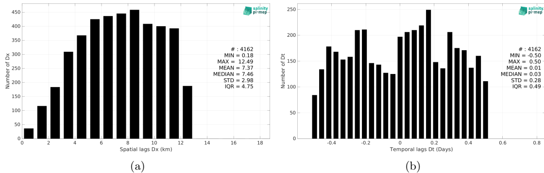
Figure 6: Histograms of the spatial (a) and temporal (b) lags between the location/time of the TSG (Lauge-Koch) measurement and the date of the corresponding SMOS SSS L2Q v331 - No FLAG (CMEMS-CATDS-CPDC) SSS pixel.
