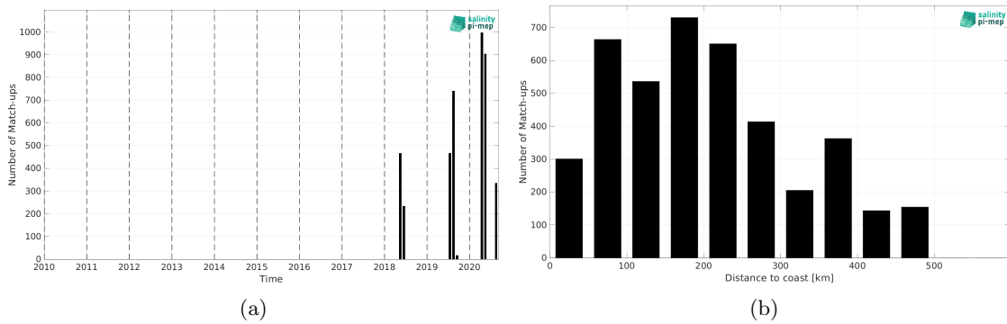
Figure 1: Number of match-ups between TSG (Lauge-Koch) and SMOS SSS L2Q v331 - No FLAG (CMEMS-CATDS-CPDC) SSS as a function of time (a) and as function of the distance to coast (b) over the Global Ocean Pi-MEP region and for the full satellite product period.
