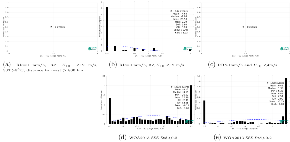
Figure 13: Normalized histogram of \Delta SSS (SMOS SSS L2Q v331 - No FLAG (CMEMS-CATDS-CPDC) - TSG (Lauge-Koch)) for 5 different subdatasets corresponding to: RR=0 mm/h, 3 < U_{10} < 12 m/s, SST>5°C, distance to coast > 800 km (a), RR=0 mm/h, 3 < U_{10} < 12 m/s (b), RR>1mm/h and U_{10} < 4 m/s (c), WOA2013 SSS Std<0.2 (d), WOA2013 SSS Std>0.2 (e).
