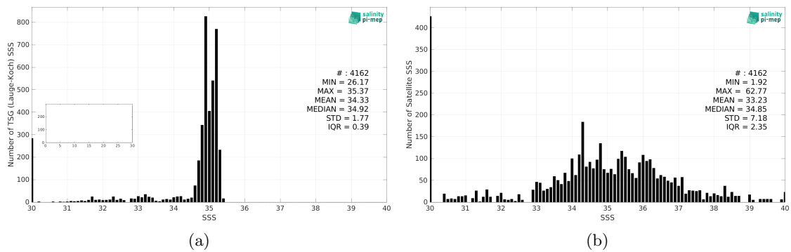
Figure 2: Histograms of SSS from TSG (Lauge-Koch) (a) and SMOS SSS L2Q v331 - No FLAG (CMEMS-CATDS-CPDC) (b) considering all match-up pairs per bins of 0.1 over the Global Ocean Pi-MEP region and for the full satellite product period.
