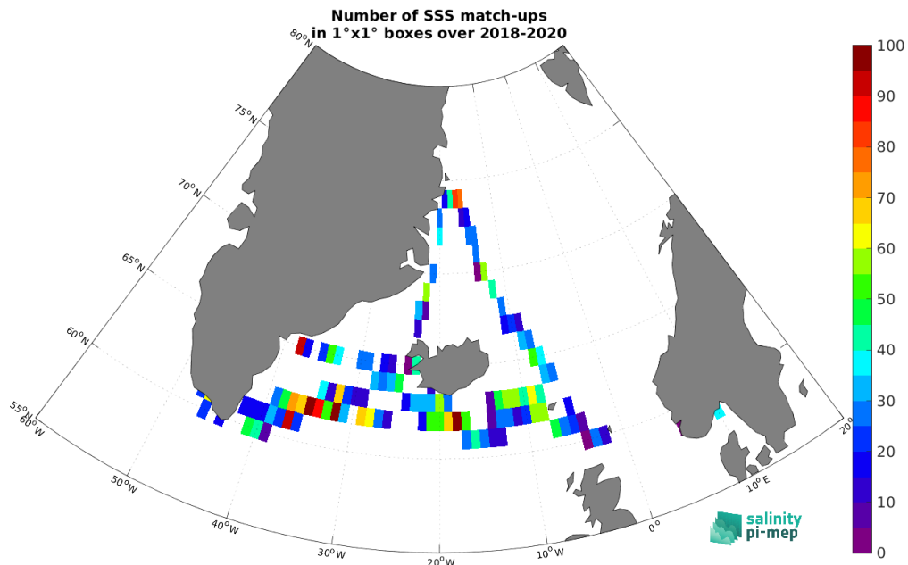
Figure 4: Number of SSS match-ups between TSG (Lauge-Koch) SSS and the SMOS SSS L2Q v331 - No FLAG (CMEMS-CATDS-CPDC) SSS product for the Global Ocean Pi-MEP region over 1^\circ \times 1^\circ boxes and for the full satellite product period.
