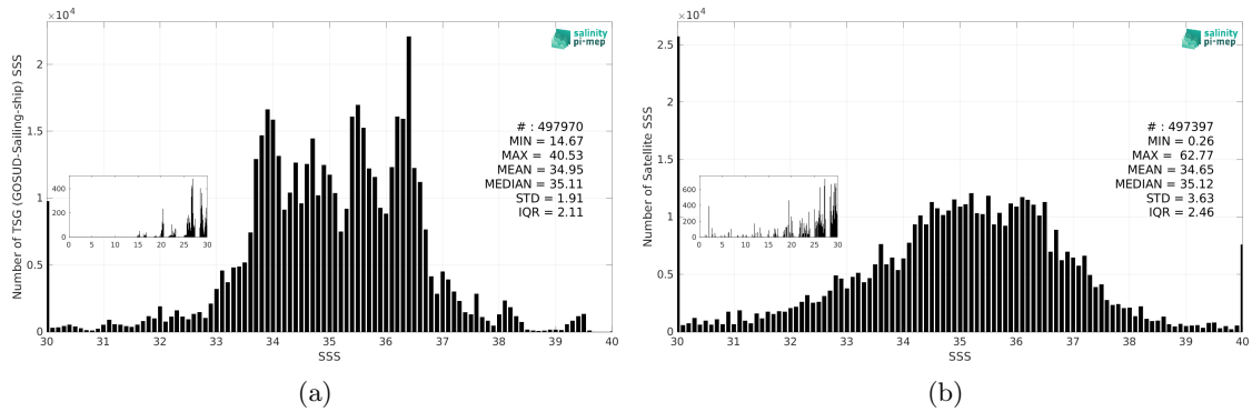
Figure 3: Histograms of SSS from TSG (GOSUD-Sailing-ship) (a) and SMOS SSS L2Q v331 - No FLAG (CMEMS-CATDS-CPDC) (b) considering all match-up pairs per bins of 0.1 over the Global Ocean Pi-MEP region and for the full satellite product period.
