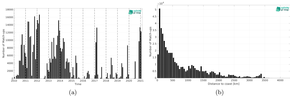
Figure 2: Number of match-ups between TSG (GOSUD-Sailing-ship) and SMOS SSS L2Q v331 - No FLAG (CMEMS-CATDS-CPDC) SSS as a function of time (a) and as function of the distance to coast (b) over the Global Ocean Pi-MEP region and for the full satellite product period.
