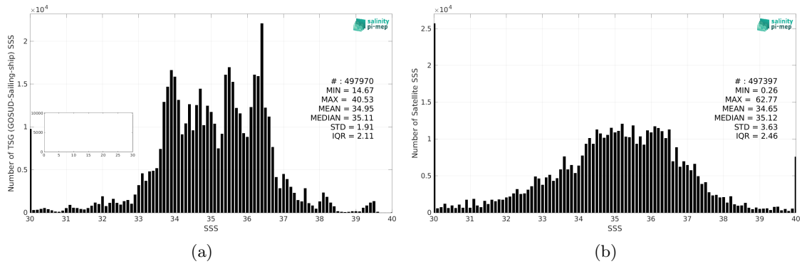
Figure 2: Histograms of SSS from TSG (GOSUD-Sailing-ship) (a) and SMOS SSS L2Q v331 - No FLAG (CMEMS-CATDS-CPDC) (b) considering all match-up pairs per bins of 0.1 over the Global Ocean Pi-MEP region and for the full satellite product period.
