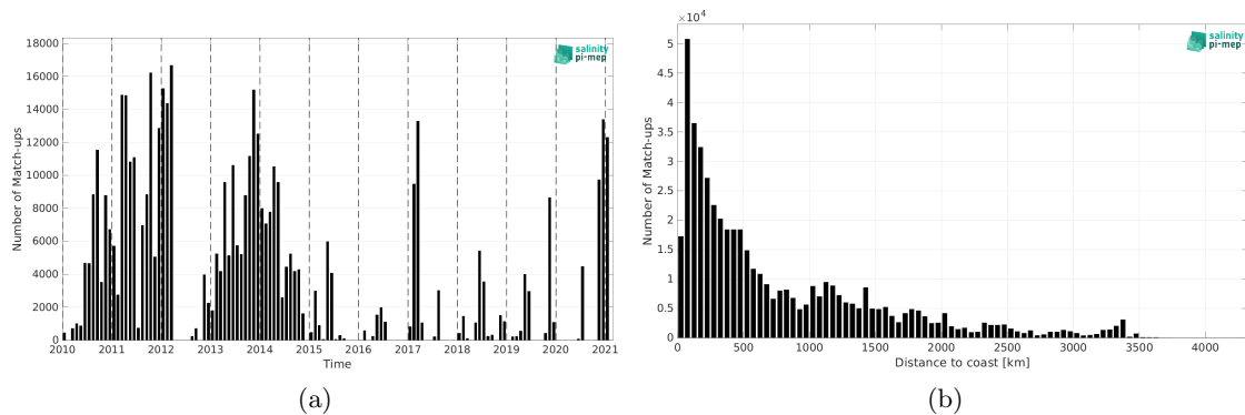
Figure 1: Number of match-ups between TSG (GOSUD-Sailing-ship) and SMOS SSS L2Q v331 - No FLAG (CMEMS-CATDS-CPDC) SSS as a function of time (a) and as function of the distance to coast (b) over the Global Ocean Pi-MEP region and for the full satellite product period.
