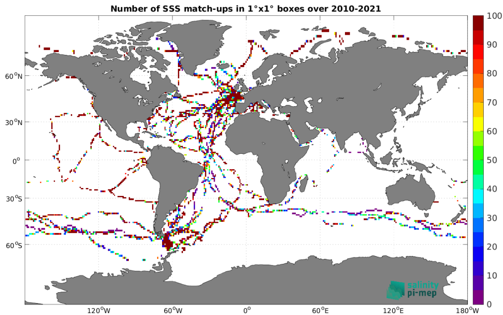
Figure 4: Number of SSS match-ups between TSG (GOSUD-Sailing-ship) SSS and the SMOS SSS L2Q v331 - No FLAG (CMEMS-CATDS-CPDC) SSS product for the Global Ocean Pi-MEP region over 1^\circ \times 1^\circ boxes and for the full satellite product period.
