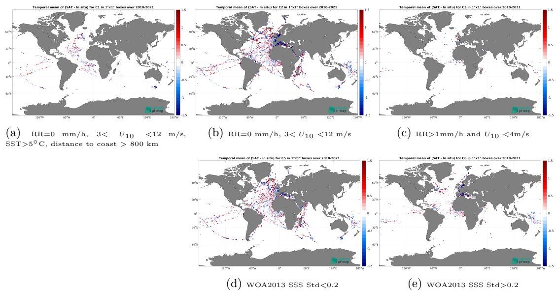
Figure 14: Temporal mean gridded over spatial boxes of size 1^\circ \times 1^\circ of \Delta\text{SSS} (SMOS SSS L2Q v331 - No FLAG (CMEMS-CATDS-CPDC) - TSG (GOSUD-Research-vessel)) for 5 different subdatasets corresponding to:RR=0 mm/h, 3 < U_{10} < 12 m/s, SST > 5^\circ\text{C} , distance to coast > 800 km (a), RR=0 mm/h, 3 < U_{10} < 12 m/s (b), RR > 1 mm/h and U_{10} < 4 m/s (c), WOA2013 SSS Std < 0.2 (d), WOA2013 SSS Std > 0.2 (e).
