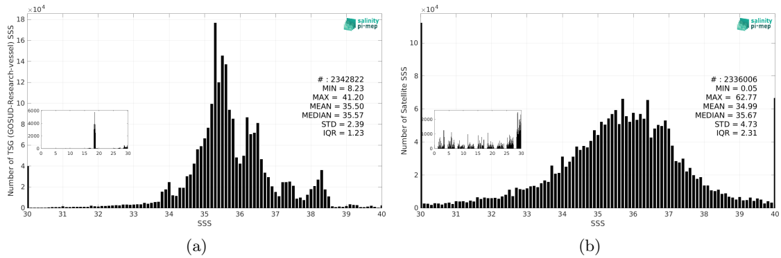
Figure 3: Histograms of SSS from TSG (GOSUD-Research-vessel) (a) and SMOS SSS L2Q v331 - No FLAG (CMEMS-CATDS-CPDC) (b) considering all match-up pairs per bins of 0.1 over the Global Ocean Pi-MEP region and for the full satellite product period.
