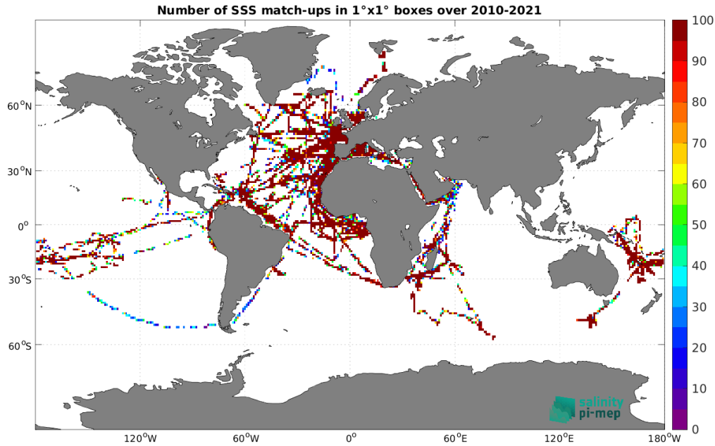
Figure 5: Number of SSS match-ups between TSG (GOSUD-Research-vessel) SSS and the SMOS SSS L2Q v331 - No FLAG (CMEMS-CATDS-CPDC) SSS product for the Global Ocean Pi-MEP region over 1^\circ \times 1^\circ boxes and for the full satellite product period.
