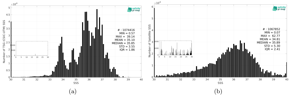
Figure 3: Histograms of SSS from TSG (CSIC-UTM) (a) and SMOS SSS L2Q v331 - No FLAG (CMEMS-CATDS-CPDC) (b) considering all match-up pairs per bins of 0.1 over the Global Ocean Pi-MEP region and for the full satellite product period.
