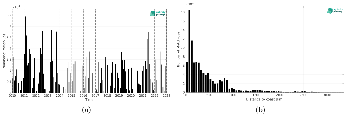
Figure 2: Number of match-ups between TSG (CSIC-UTM) and SMOS SSS L2Q v331 - No FLAG (CMEMS-CATDS-CPDC) SSS as a function of time (a) and as function of the distance to coast (b) over the Global Ocean Pi-MEP region and for the full satellite product period.
