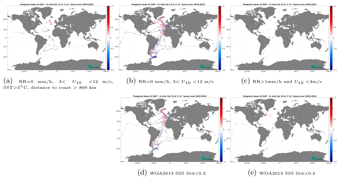
Figure 14: Temporal mean gridded over spatial boxes of size 1^\circ \times 1^\circ of \Delta\text{SSS} (SMOS SSS L2Q v331 - No FLAG (CMEMS-CATDS-CPDC) - TSG (CSIC-UTM)) for 5 different subdatasets corresponding to:RR=0 mm/h, 3 < U_{10} < 12 m/s, SST > 5^\circ\text{C} , distance to coast > 800 km (a), RR=0 mm/h, 3 < U_{10} < 12 m/s (b), RR > 1 mm/h and U_{10} < 4 m/s (c), WOA2013 SSS Std < 0.2 (d), WOA2013 SSS Std > 0.2 (e).
