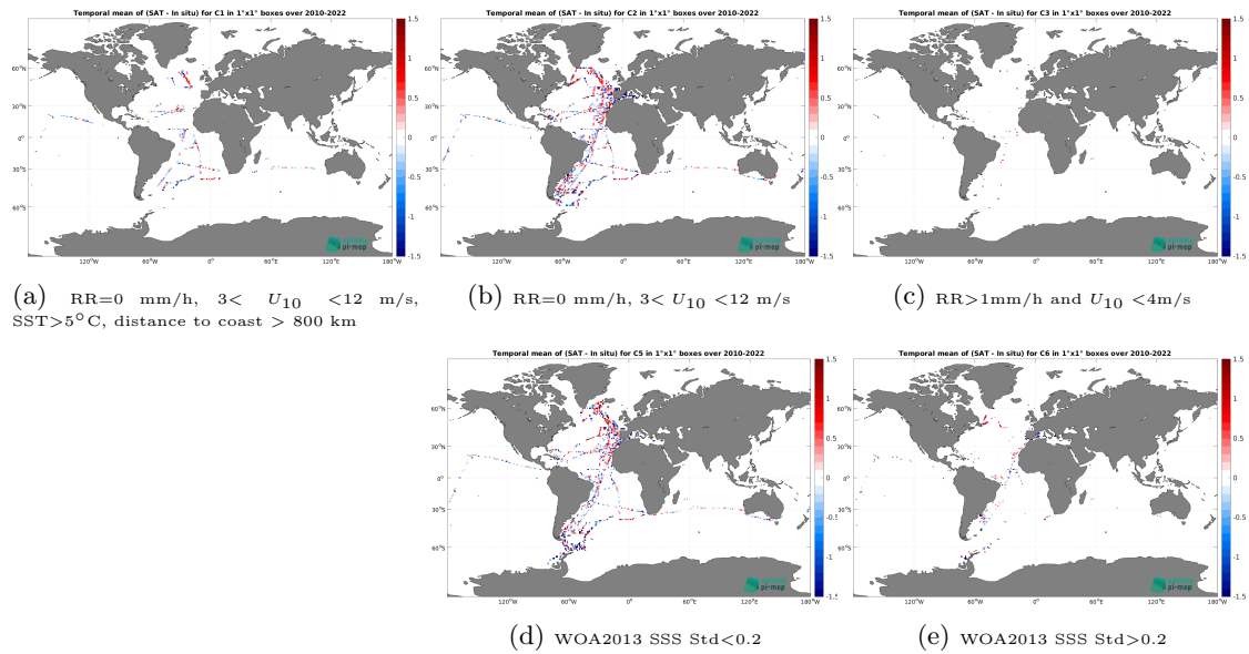
Figure 12: Temporal mean gridded over spatial boxes of size 1^\circ \times 1^\circ of \Delta\text{SSS} (SMOS SSS L2Q v331 - No FLAG (CMEMS-CATDS-CPDC) - TSG (CSIC-UTM)) for 5 different subdatasets corresponding to:RR=0 mm/h, 3 < U_{10} < 12 m/s, SST >5^\circ\text{C} , distance to coast > 800 km (a), RR=0 mm/h, 3 < U_{10} < 12 m/s (b), RR >1 mm/h and U_{10} < 4 m/s (c), WOA2013 SSS Std <0.2 (d), WOA2013 SSS Std >0.2 (e).
