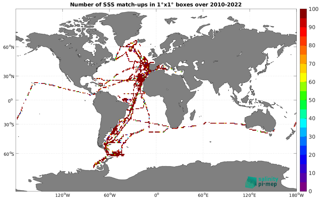
Figure 4: Number of SSS match-ups between TSG (CSIC-UTM) SSS and the SMOS SSS L2Q v331 - No FLAG (CMEMS-CATDS-CPDC) SSS product for the Global Ocean Pi-MEP region over 1^\circ \times 1^\circ boxes and for the full satellite product period.
