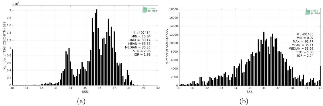
Figure 2: Histograms of SSS from TSG (CSIC-UTM) (a) and SMOS SSS L2Q v331 - No FLAG (CMEMS-CATDS-CPDC) (b) considering all match-up pairs per bins of 0.1 over the Global Ocean Pi-MEP region and for the full satellite product period.
