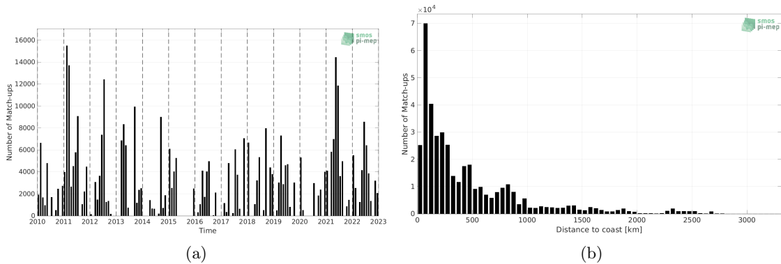
Figure 1: Number of match-ups between TSG (CSIC-UTM) and SMOS SSS L2Q v331 - No FLAG (CMEMS-CATDS-CPDC) SSS as a function of time (a) and as function of the distance to coast (b) over the Global Ocean Pi-MEP region and for the full satellite product period.
