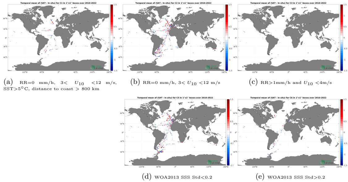
Figure 12: Temporal mean gridded over spatial boxes of size 1^\circ \times 1^\circ of \Delta SSS (SMOS SSS L2Q v331 - No FLAG (CMEMS-CATDS-CPDC) - TSG (CSIC-UTM)) for 5 different subdatasets corresponding to:RR=0 mm/h, 3 < U_{10} < 12 m/s, SST >5^\circ\text{C} , distance to coast > 800 km (a), RR=0 mm/h, 3 < U_{10} < 12 m/s (b), RR >1 mm/h and U_{10} < 4 m/s (c), WOA2013 SSS Std <0.2 (d), WOA2013 SSS Std >0.2 (e).
