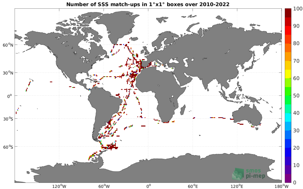
Figure 4: Number of SSS match-ups between TSG (CSIC-UTM) SSS and the SMOS SSS L2Q v331 - No FLAG (CMEMS-CATDS-CPDC) SSS product for the Global Ocean Pi-MEP region over 1°×1° boxes and for the full satellite product period.
