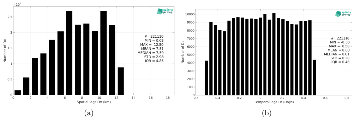
Figure 5: Histograms of the spatial (a) and temporal (b) lags between the location/time of the TSG (Amundsen) measurement and the date of the corresponding SMOS SSS L2Q v331 - No FLAG (CMEMS-CATDS-CPDC) SSS pixel.
