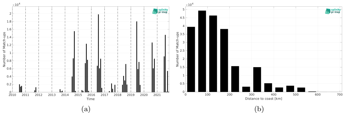
Figure 1: Number of match-ups between TSG (Amundsen) and SMOS SSS L2Q v331 - No FLAG (CMEMS-CATDS-CPDC) SSS as a function of time (a) and as function of the distance to coast (b) over the Global Ocean Pi-MEP region and for the full satellite product period.
