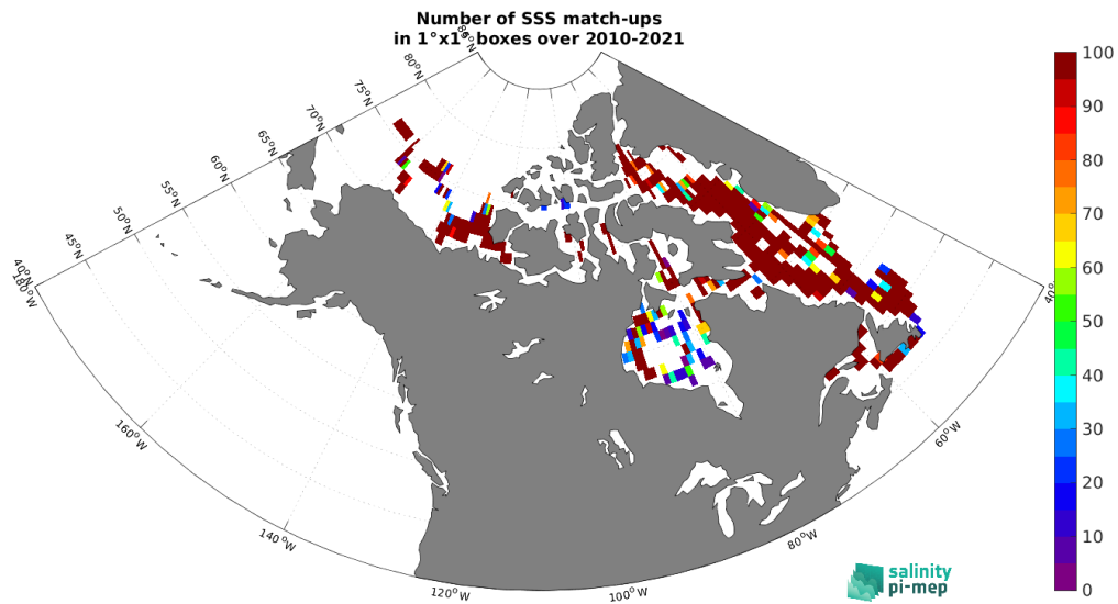
Figure 4: Number of SSS match-ups between TSG (Amundsen) SSS and the SMOS SSS L2Q v331 - No FLAG (CMEMS-CATDS-CPDC) SSS product for the Global Ocean Pi-MEP region over 1^\circ \times 1^\circ boxes and for the full satellite product period.
