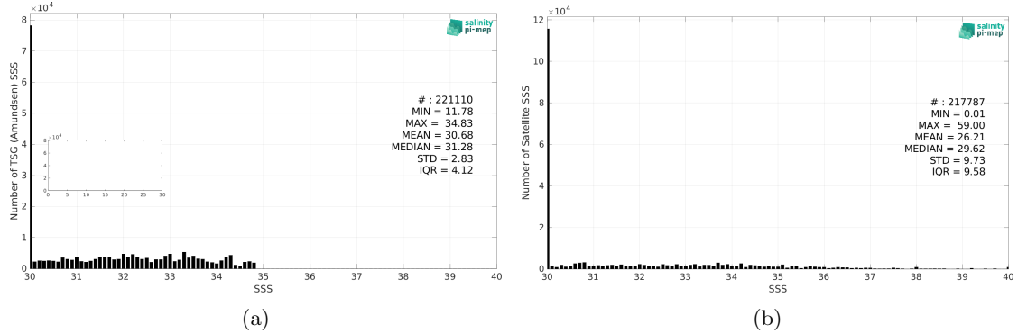
Figure 2: Histograms of SSS from TSG (Amundsen) (a) and SMOS SSS L2Q v331 - No FLAG (CMEMS-CATDS-CPDC) (b) considering all match-up pairs per bins of 0.1 over the Global Ocean Pi-MEP region and for the full satellite product period.
