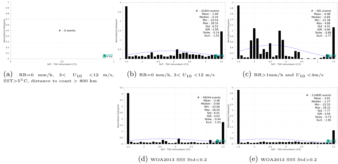
Figure 13: Normalized histogram of \Delta SSS (SMOS SSS L2Q v331 - No FLAG (CMEMS-CATDS-CPDC) - TSG (Amundsen)) for 5 different subdatasets corresponding to: RR=0 mm/h, 3 < U_{10} < 12 m/s, SST > 5°C, distance to coast > 800 km (a), RR=0 mm/h, 3 < U_{10} < 12 m/s (b), RR > 1mm/h and U_{10} < 4 m/s (c), WOA2013 SSS Std < 0.2 (d), WOA2013 SSS Std > 0.2 (e).
