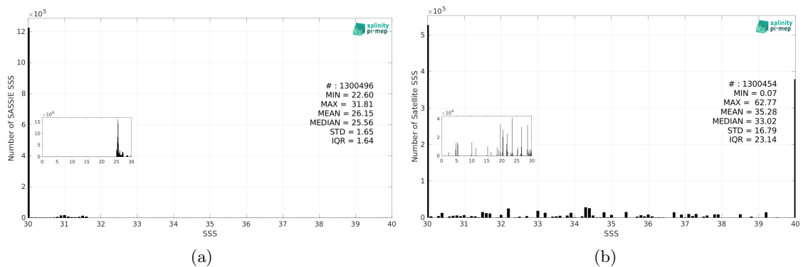
Figure 3: Histograms of SSS from SASSIE (a) and SMOS SSS L2Q v331 - No FLAG (CMEMS-CATDS-CPDC) (b) considering all match-up pairs per bins of 0.1 over the Global Ocean Pi-MEP region and for the full satellite product period.
