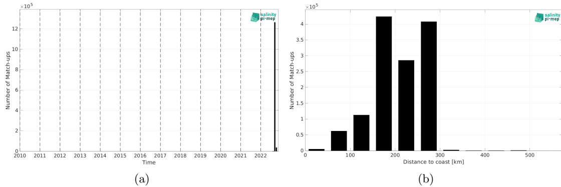
Figure 2: Number of match-ups between SASSIE and SMOS SSS L2Q v331 - No FLAG (CMEMS-CATDS-CPDC) SSS as a function of time (a) and as function of the distance to coast (b) over the Global Ocean Pi-MEP region and for the full satellite product period.
