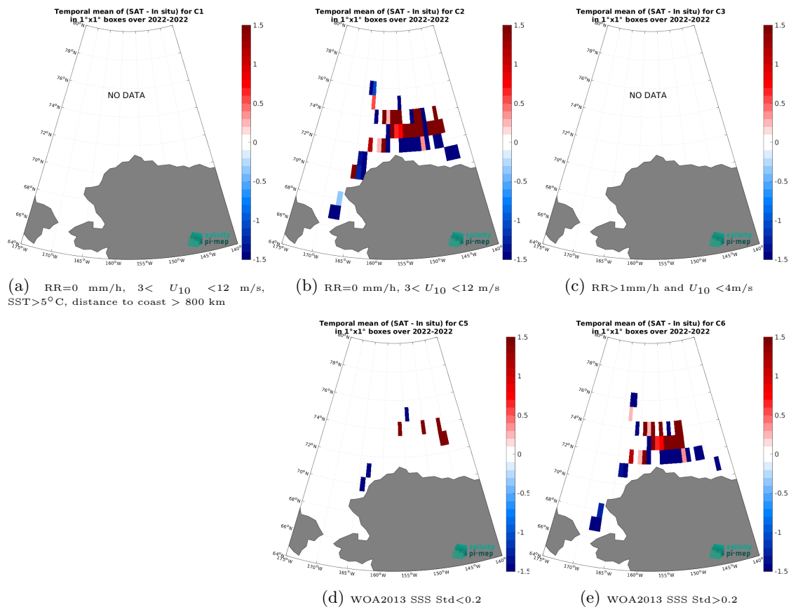
Figure 14: Temporal mean gridded over spatial boxes of size 1^\circ \times 1^\circ of \Delta SSS (SMOS SSS L2Q v331 - No FLAG (CMEMS-CATDS-CPDC) - SASSIE) for 5 different subdatasets corresponding to: RR=0 mm/h, 3 < U_{10} < 12 m/s, SST >5^\circ\text{C} , distance to coast > 800 km (a), RR=0 mm/h, 3 < U_{10} < 12 m/s (b), RR >1 mm/h and U_{10} < 4 m/s (c), WOA2013 SSS Std <0.2 (d), WOA2013 SSS Std >0.2 (e).
