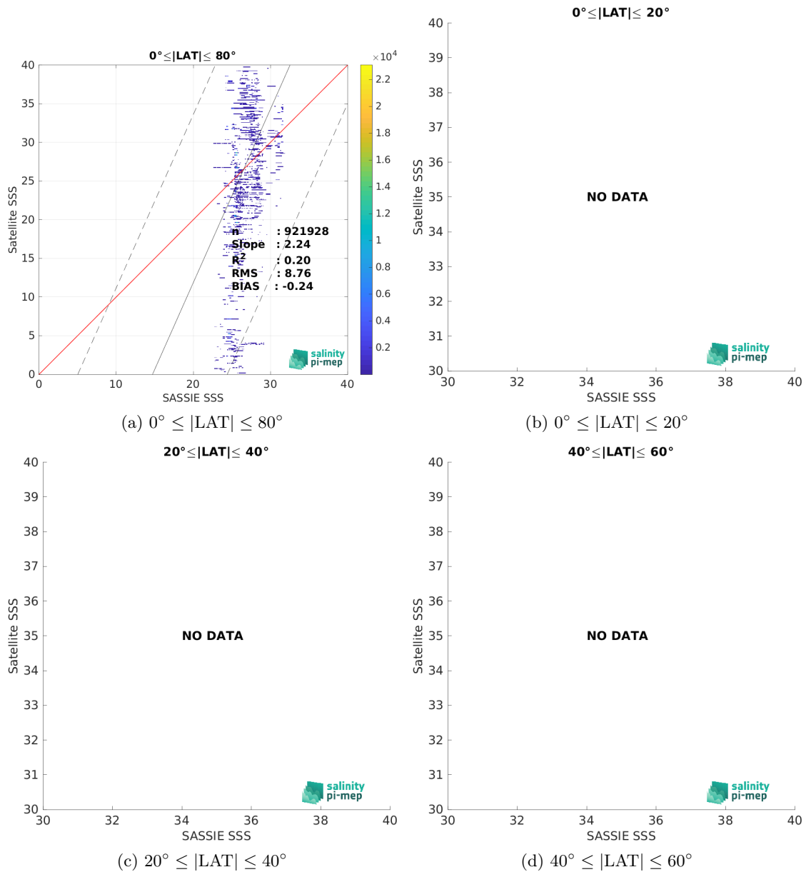
Figure 10: Contour maps of the concentration of SMOS SSS L2Q v331 - No FLAG (CMEMS-CATDS-CPDC) SSS (y-axis) versus SASSIE SSS (x-axis) at match-up pairs for different latitude bands. For each plot, the red line shows x=y . The black thin and dashed lines indicate a linear fit through the data cloud and the \pm 95\% confidence levels, respectively. The number match-up pairs n , the slope and R^2 coefficient of the linear fit, the root mean square (RMS) and the mean bias between satellite and in situ data are indicated for each latitude band in each plots.
