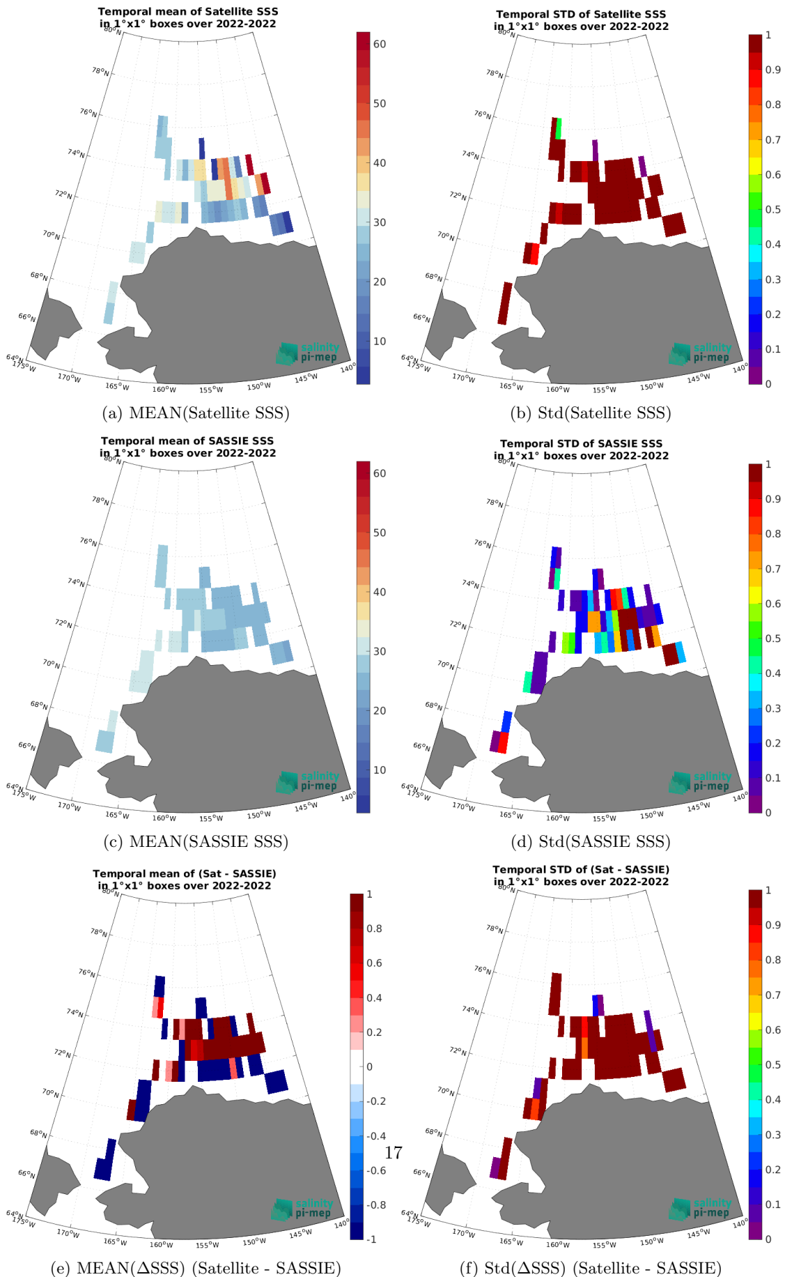
Figure 7: Temporal mean (left) and Std (right) of SSS from SMOS SSS L2Q v331 - No FLAG (CMEMS-CATDS-CPDC) (top), SASSIE (middle), and of \Delta SSS (Satellite - SASSIE). Only match-up pairs are used to generate these maps.
