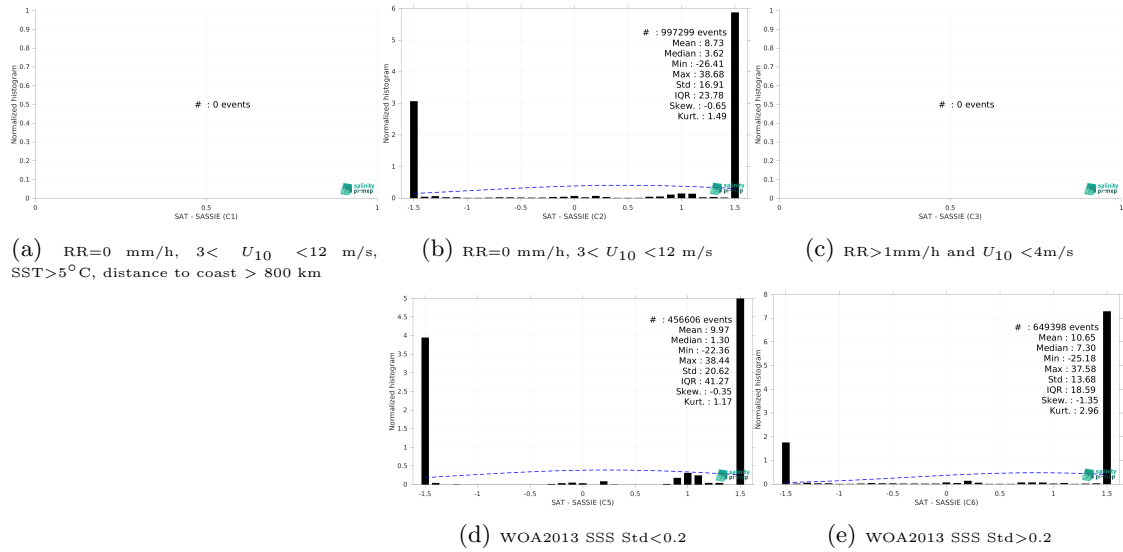
Figure 15: Normalized histogram of \Delta SSS (SMOS SSS L2Q v331 - No FLAG (CMEMS-CATDS-CPDC) - SASSIE) for 5 different subdatasets corresponding to: RR=0 mm/h, 3 < U_{10} < 12 m/s, SST > 5°C, distance to coast > 800 km (a), RR=0 mm/h, 3 < U_{10} < 12 m/s (b), RR > 1mm/h and U_{10} < 4 m/s (c), WOA2013 SSS Std < 0.2 (d), WOA2013 SSS Std > 0.2 (e).
