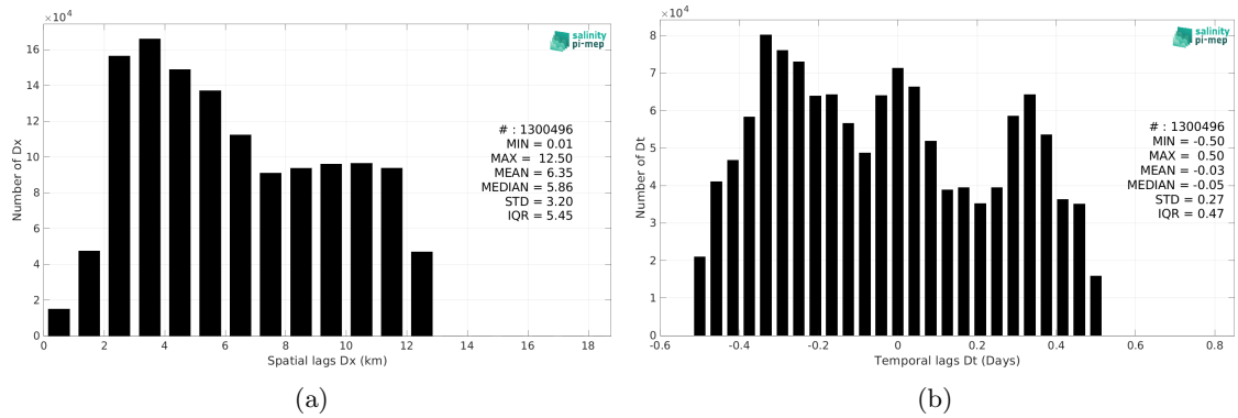
Figure 6: Histograms of the spatial (a) and temporal (b) lags between the location/time of the SASSIE measurement and the date of the corresponding SMOS SSS L2Q v331 - No FLAG (CMEMS-CATDS-CPDC) SSS pixel.
