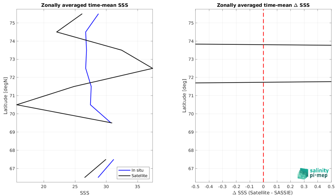
Figure 9: Left panel: Zonal mean SSS from SMOS SSS L2Q v331 - No FLAG (CMEMS-CATDS-CPDC) satellite product (black) and from SASSIE (blue). Right panel: Zonal mean of \Delta SSS (Satellite - SASSIE) for all the collected Pi-MEP match-up pairs estimated over the full satellite product period.
