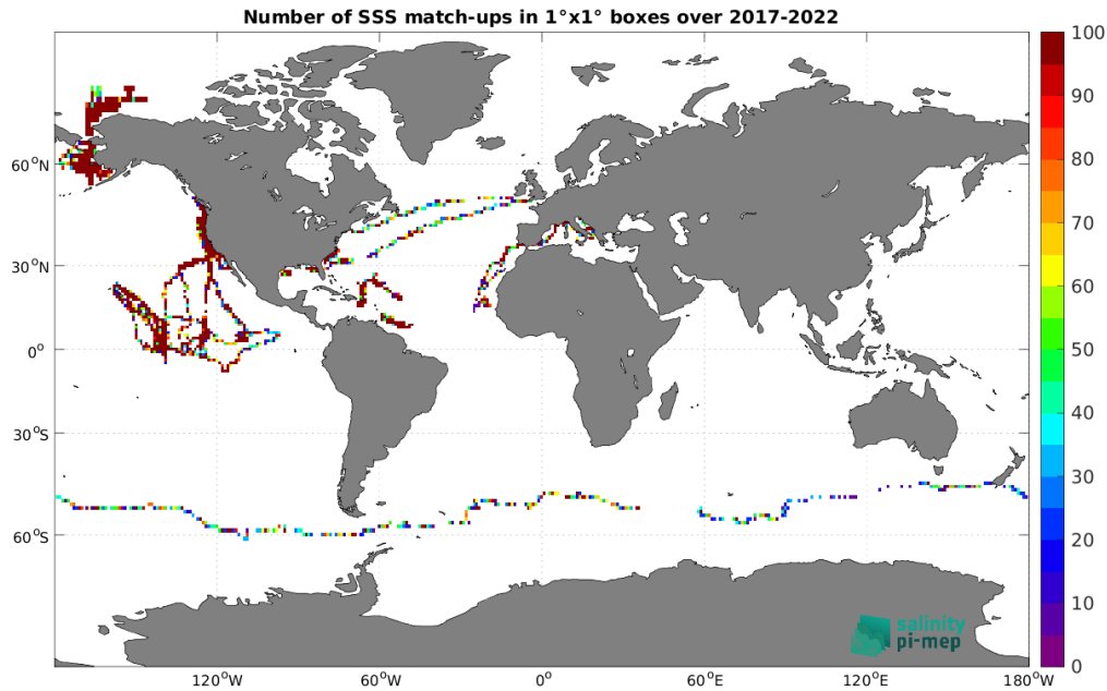
Figure 5: Number of SSS match-ups between Saildrone SSS and the SMOS SSS L2Q v331 - No FLAG (CMEMS-CATDS-CPDC) SSS product for the Global Ocean Pi-MEP region over 1^\circ \times 1^\circ boxes and for the full satellite product period.
