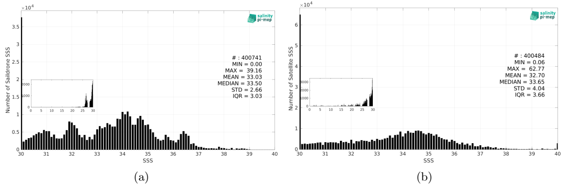
Figure 3: Histograms of SSS from Saildrone (a) and SMOS SSS L2Q v331 - No FLAG (CMEMS-CATDS-CPDC) (b) considering all match-up pairs per bins of 0.1 over the Global Ocean Pi-MEP region and for the full satellite product period.
