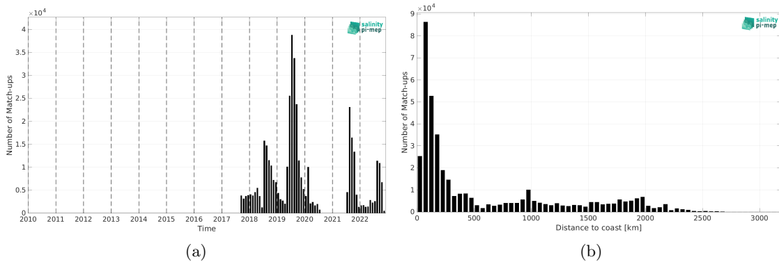
Figure 2: Number of match-ups between Saildrone and SMOS SSS L2Q v331 - No FLAG (CMEMS-CATDS-CPDC) SSS as a function of time (a) and as function of the distance to coast (b) over the Global Ocean Pi-MEP region and for the full satellite product period.
