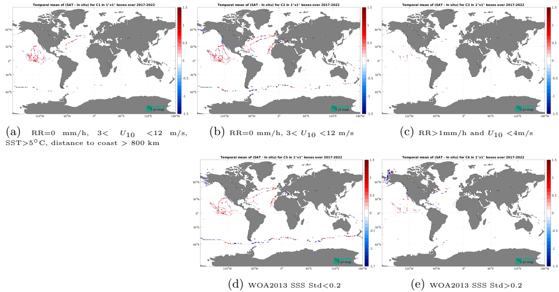
Figure 12: Temporal mean gridded over spatial boxes of size 1^\circ \times 1^\circ of \Delta SSS (SMOS SSS L2Q v331 - No FLAG (CMEMS-CATDS-CPDC) - Saildrone) for 5 different subdatasets corresponding to:RR=0 mm/h, 3 < U_{10} < 12 m/s, SST >5^\circ C, distance to coast > 800 km (a), RR=0 mm/h, 3 < U_{10} < 12 m/s (b), RR >1 mm/h and U_{10} < 4 m/s (c), WOA2013 SSS Std <0.2 (d), WOA2013 SSS Std >0.2 (e).
