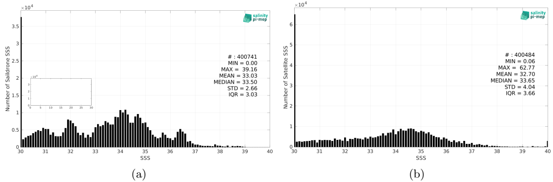
Figure 2: Histograms of SSS from Saildrone (a) and SMOS SSS L2Q v331 - No FLAG (CMEMS-CATDS-CPDC) (b) considering all match-up pairs per bins of 0.1 over the Global Ocean Pi-MEP region and for the full satellite product period.
