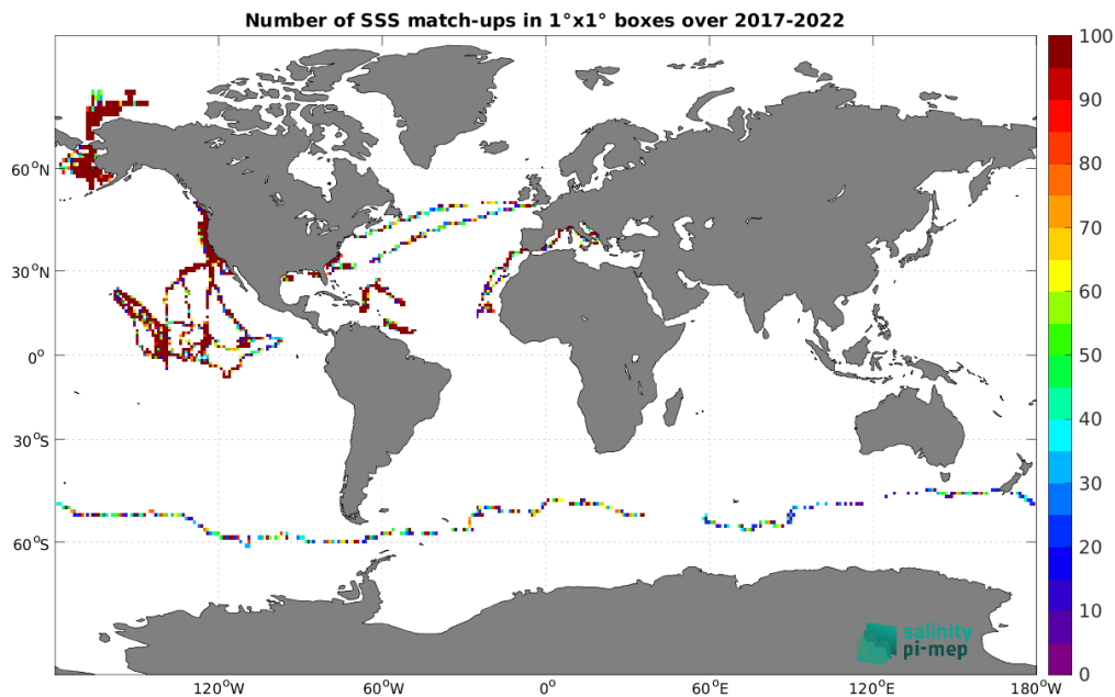
Figure 4: Number of SSS match-ups between Saildrone SSS and the SMOS SSS L2Q v331 - No FLAG (CMEMS-CATDS-CPDC) SSS product for the Global Ocean Pi-MEP region over 1^\circ \times 1^\circ boxes and for the full satellite product period.
