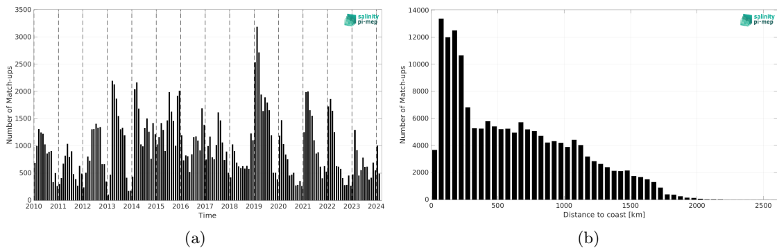
Figure 2: Number of match-ups between Marine mammals and SMOS SSS L2Q v331 - No FLAG (CMEMS-CATDS-CPDC) SSS as a function of time (a) and as function of the distance to coast (b) over the Global Ocean Pi-MEP region and for the full satellite product period.
