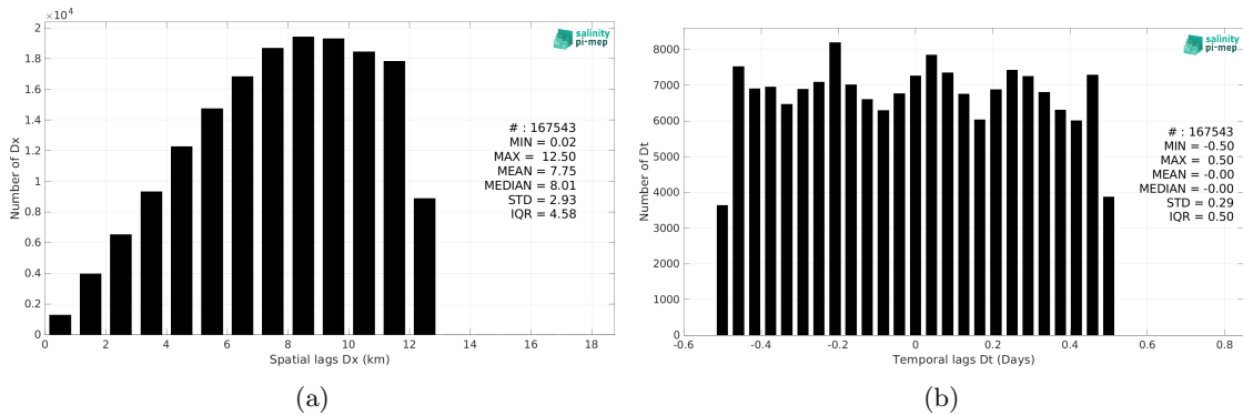
Figure 6: Histograms of the spatial (a) and temporal (b) lags between the location/time of the Marine mammals measurement and the date of the corresponding SMOS SSS L2Q v331 - No FLAG (CMEMS-CATDS-CPDC) SSS pixel.
