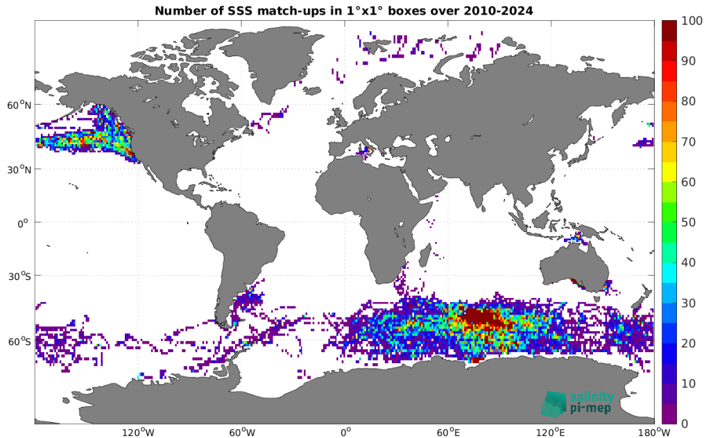
Figure 5: Number of SSS match-ups between Marine mammals SSS and the SMOS SSS L2Q v331 - No FLAG (CMEMS-CATDS-CPDC) SSS product for the Global Ocean Pi-MEP region over 1^\circ \times 1^\circ boxes and for the full satellite product period.
