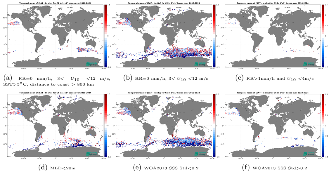
Figure 14: Temporal mean gridded over spatial boxes of size 1^\circ \times 1^\circ of \Delta SSS (SMOS SSS L2Q v331 - No FLAG (CMEMS-CATDS-CPDC) - Marine mammals) for 6 different subdatasets corresponding to:RR=0 mm/h, 3 < U_{10} < 12 m/s, SST>5°C, distance to coast > 800 km (a), RR=0 mm/h, 3 < U_{10} < 12 m/s (b), RR>1mm/h and U_{10} < 4 m/s (c),MLD<20m (d),WOA2013 SSS Std<0.2 (e),WOA2013 SSS Std>0.2 (f).
