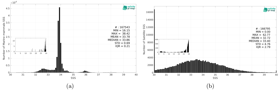
Figure 3: Histograms of SSS from Marine mammals (a) and SMOS SSS L2Q v331 - No FLAG (CMEMS-CATDS-CPDC) (b) considering all match-up pairs per bins of 0.1 over the Global Ocean Pi-MEP region and for the full satellite product period.
