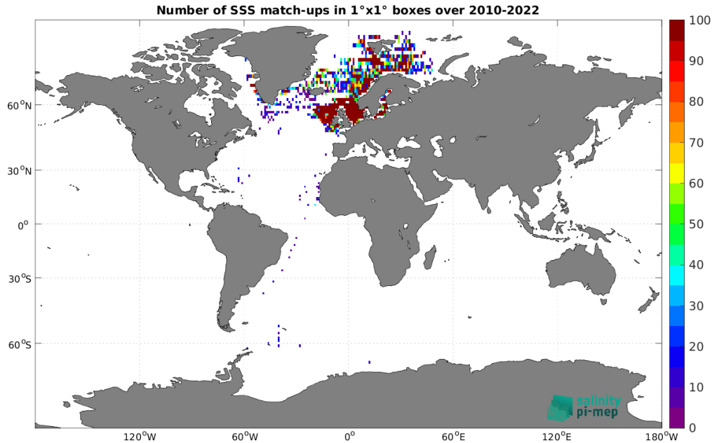
Figure 5: Number of SSS match-ups between ICES SSS and the SMOS SSS L2Q v331 - No FLAG (CMEMS-CATDS-CPDC) SSS product for the Global Ocean Pi-MEP region over 1^\circ \times 1^\circ boxes and for the full satellite product period.
