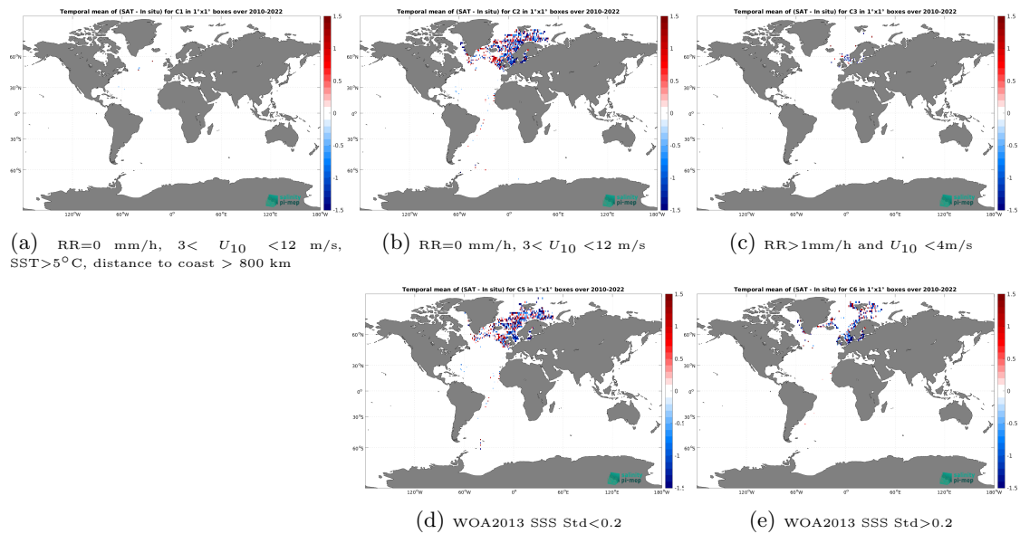
Figure 14: Temporal mean gridded over spatial boxes of size 1^\circ \times 1^\circ of \Delta SSS (SMOS SSS L2Q v331 - No FLAG (CMEMS-CATDS-CPDC) - ICES) for 5 different subdatasets corresponding to: RR=0 mm/h, 3 < U_{10} < 12 m/s, SST > 5^\circ\text{C} , distance to coast > 800 km (a), RR=0 mm/h, 3 < U_{10} < 12 m/s (b), RR > 1 mm/h and U_{10} < 4 m/s (c), WOA2013 SSS Std < 0.2 (d), WOA2013 SSS Std > 0.2 (e).
