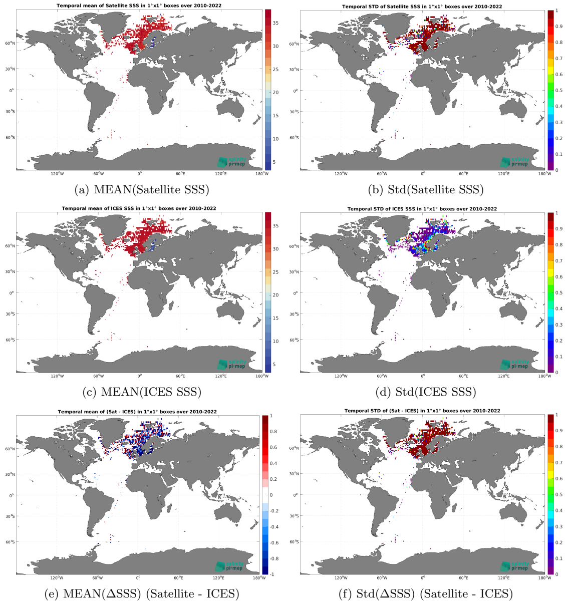
Figure 7: Temporal mean (left) and Std (right) of SSS from SMOS SSS L2Q v331 - No FLAG (CMEMS-CATDS-CPDC) (top), ICES (middle), and of \Delta SSS (Satellite - ICES). Only match-up pairs are used to generate these maps.
