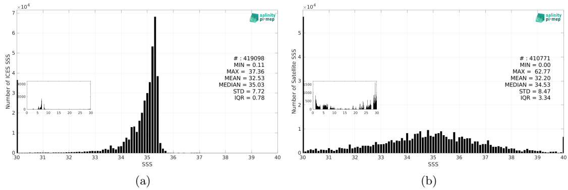
Figure 3: Histograms of SSS from ICES (a) and SMOS SSS L2Q v331 - No FLAG (CMEMS-CATDS-CPDC) (b) considering all match-up pairs per bins of 0.1 over the Global Ocean Pi-MEP region and for the full satellite product period.
