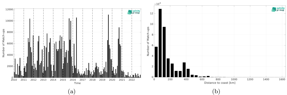
Figure 1: Number of match-ups between ICES and SMOS SSS L2Q v331 - No FLAG (CMEMS-CATDS-CPDC) SSS as a function of time (a) and as function of the distance to coast (b) over the Global Ocean Pi-MEP region and for the full satellite product period.
