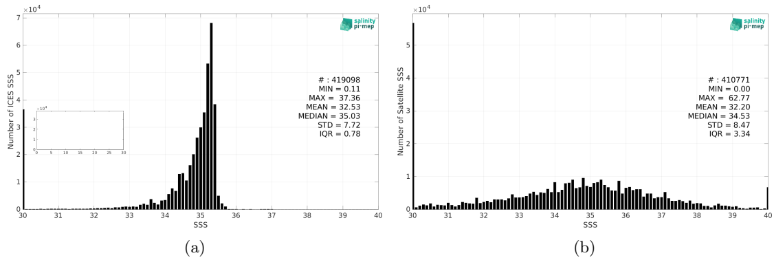
Figure 2: Histograms of SSS from ICES (a) and SMOS SSS L2Q v331 - No FLAG (CMEMS-CATDS-CPDC) (b) considering all match-up pairs per bins of 0.1 over the Global Ocean Pi-MEP region and for the full satellite product period.
