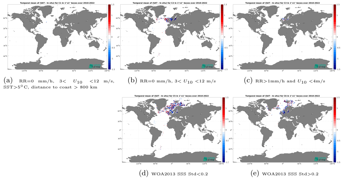
Figure 12: Temporal mean gridded over spatial boxes of size 1^\circ \times 1^\circ of \Delta SSS (SMOS SSS L2Q v331 - No FLAG (CMEMS-CATDS-CPDC) - ICES) for 5 different subdatasets corresponding to:RR=0 mm/h, 3 < U_{10} < 12 m/s, SST >5^\circ C, distance to coast > 800 km (a), RR=0 mm/h, 3 < U_{10} < 12 m/s (b), RR >1 mm/h and U_{10} < 4 m/s (c), WOA2013 SSS Std <0.2 (d), WOA2013 SSS Std >0.2 (e).
