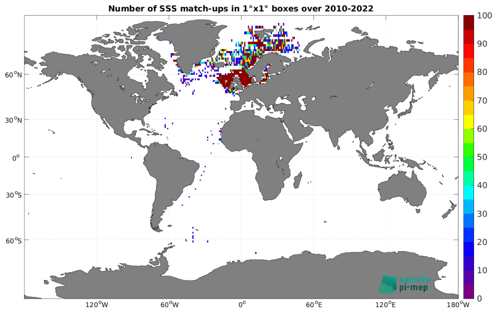
Figure 4: Number of SSS match-ups between ICES SSS and the SMOS SSS L2Q v331 - No FLAG (CMEMS-CATDS-CPDC) SSS product for the Global Ocean Pi-MEP region over 1°×1° boxes and for the full satellite product period.
