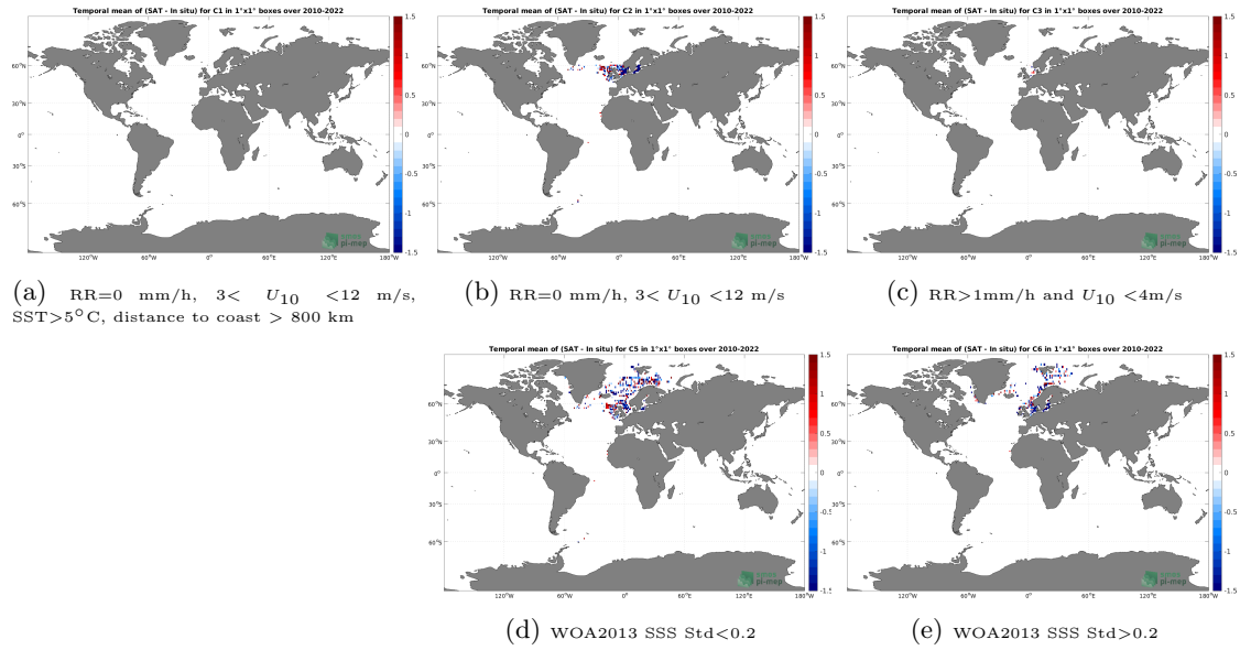
Figure 12: Temporal mean gridded over spatial boxes of size 1^\circ \times 1^\circ of \Delta SSS (SMOS SSS L2Q v331 - No FLAG (CMEMS-CATDS-CPDC) - ICES) for 5 different subdatasets corresponding to: RR=0 mm/h, 3 < U_{10} < 12 m/s, SST > 5^\circ\text{C} , distance to coast > 800 km (a), RR=0 mm/h, 3 < U_{10} < 12 m/s (b), RR > 1 mm/h and U_{10} < 4 m/s (c), WOA2013 SSS Std < 0.2 (d), WOA2013 SSS Std > 0.2 (e).
