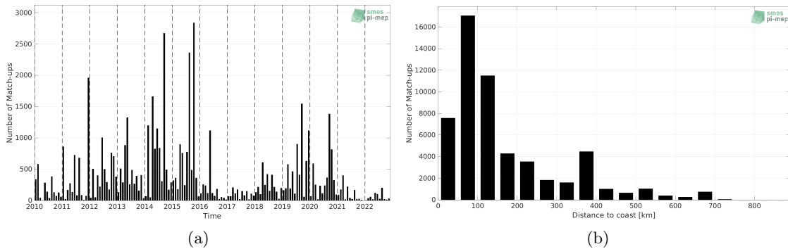
Figure 1: Number of match-ups between ICES and SMOS SSS L2Q v331 - No FLAG (CMEMS-CATDS-CPDC) SSS as a function of time (a) and as function of the distance to coast (b) over the Global Ocean Pi-MEP region and for the full satellite product period.
