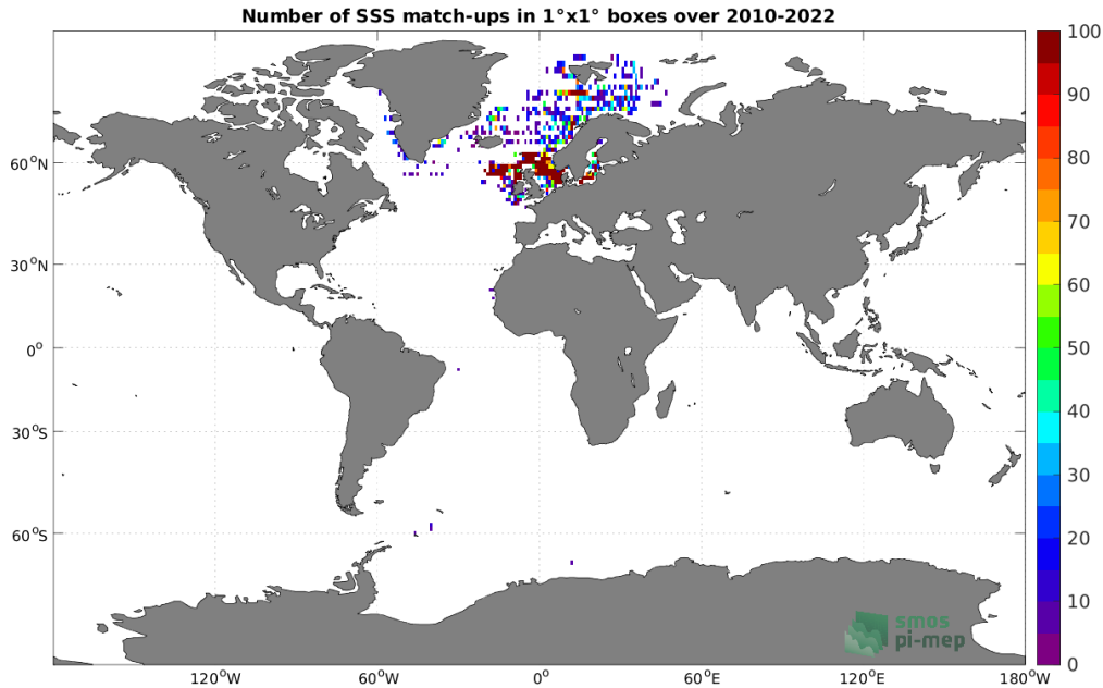
Figure 4: Number of SSS match-ups between ICES SSS and the SMOS SSS L2Q v331 - No FLAG (CMEMS-CATDS-CPDC) SSS product for the Global Ocean Pi-MEP region over 1^\circ \times 1^\circ boxes and for the full satellite product period.
