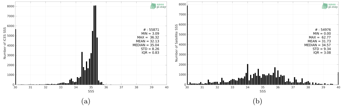
Figure 2: Histograms of SSS from ICES (a) and SMOS SSS L2Q v331 - No FLAG (CMEMS-CATDS-CPDC) (b) considering all match-up pairs per bins of 0.1 over the Global Ocean Pi-MEP region and for the full satellite product period.
