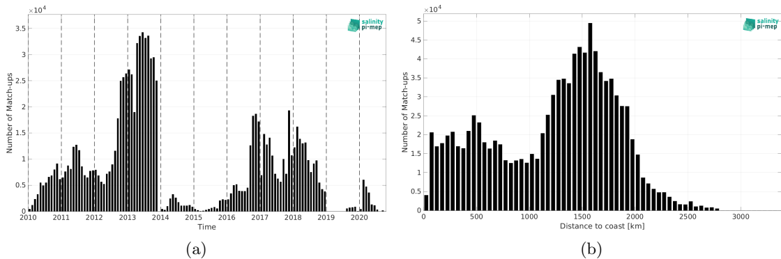
Figure 2: Number of match-ups between Surface drifters and SMOS SSS L2Q v331 - No FLAG (CMEMS-CATDS-CPDC) SSS as a function of time (a) and as function of the distance to coast (b) over the Global Ocean Pi-MEP region and for the full satellite product period.
