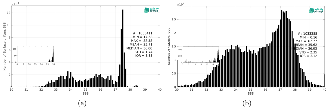
Figure 3: Histograms of SSS from Surface drifters (a) and SMOS SSS L2Q v331 - No FLAG (CMEMS-CATDS-CPDC) (b) considering all match-up pairs per bins of 0.1 over the Global Ocean Pi-MEP region and for the full satellite product period.
