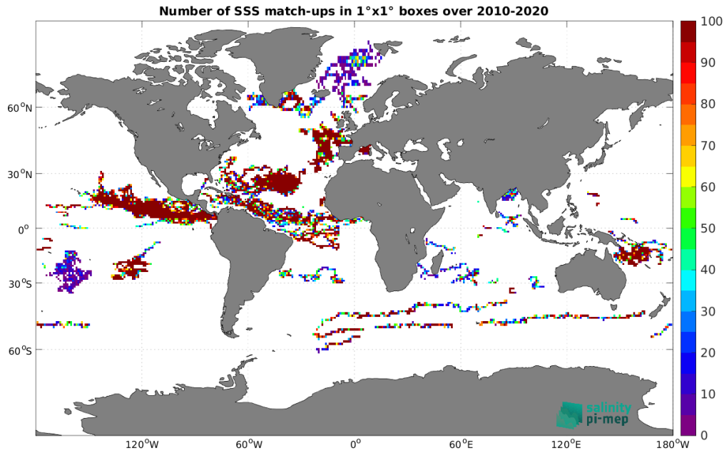
Figure 4: Number of SSS match-ups between Surface drifters SSS and the SMOS SSS L2Q v331 - No FLAG (CMEMS-CATDS-CPDC) SSS product for the Global Ocean Pi-MEP region over 1^\circ \times 1^\circ boxes and for the full satellite product period.
