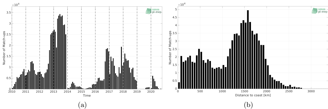
Figure 1: Number of match-ups between Surface drifters and SMOS SSS L2Q v331 - No FLAG (CMEMS-CATDS-CPDC) SSS as a function of time (a) and as function of the distance to coast (b) over the Global Ocean Pi-MEP region and for the full satellite product period.
