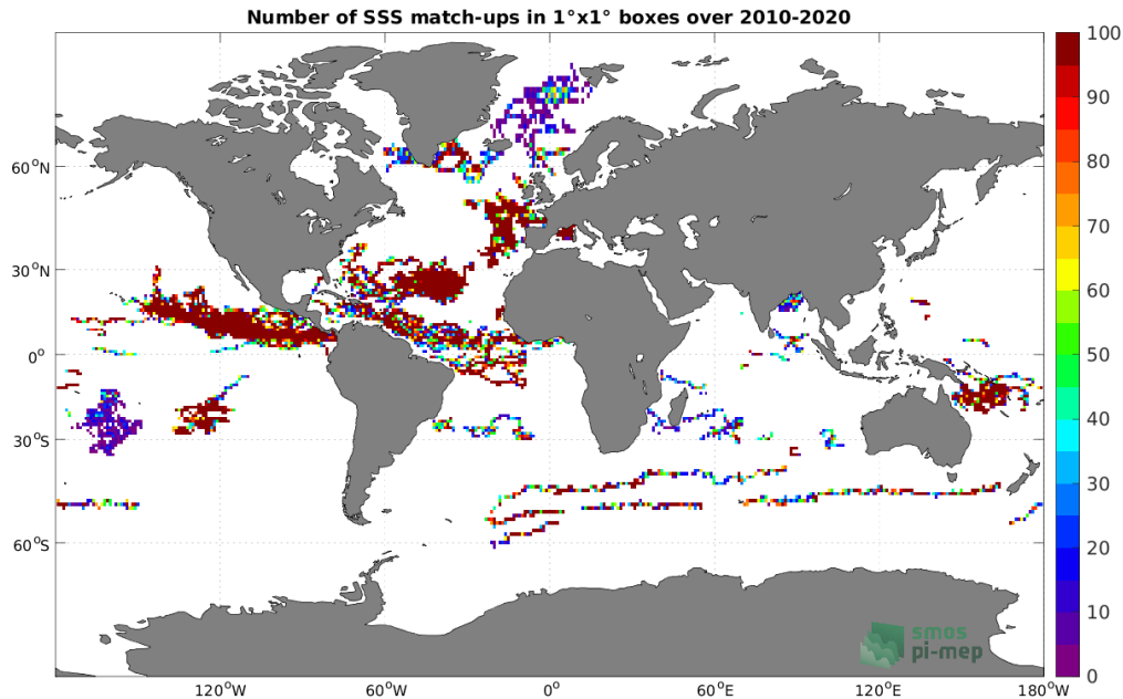
Figure 3: Number of SSS match-ups between Surface drifters SSS and the SMOS SSS L2Q v331 - No FLAG (CMEMS-CATDS-CPDC) SSS product for the Global Ocean Pi-MEP region over 1^\circ \times 1^\circ boxes and for the full satellite product period.
