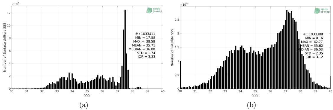
Figure 2: Histograms of SSS from Surface drifters (a) and SMOS SSS L2Q v331 - No FLAG (CMEMS-CATDS-CPDC) (b) considering all match-up pairs per bins of 0.1 over the Global Ocean Pi-MEP region and for the full satellite product period.
