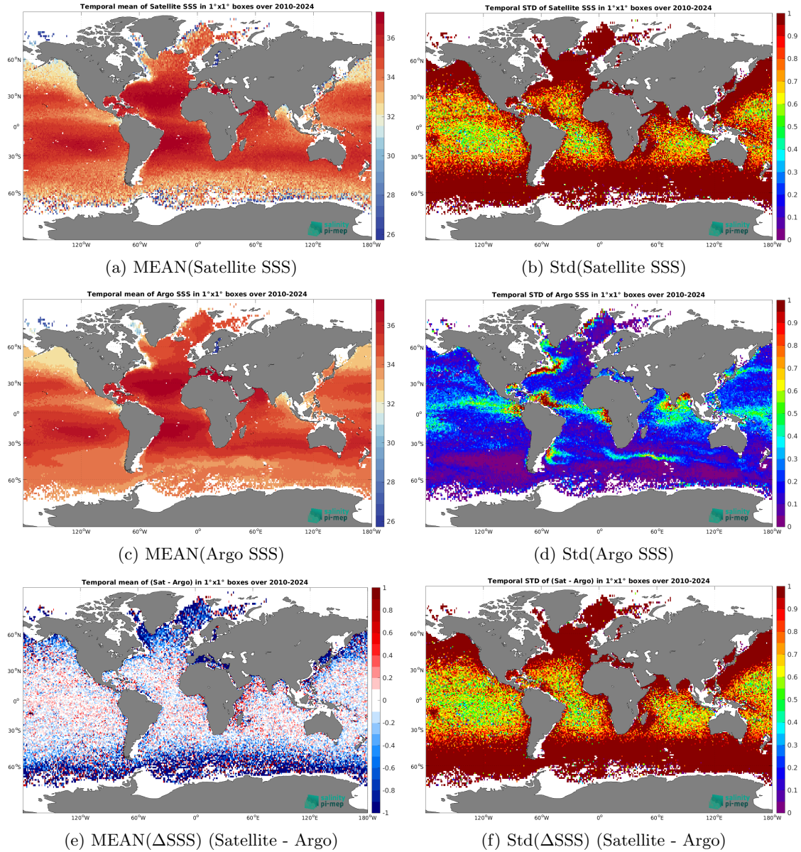
Figure 7: Temporal mean (left) and Std (right) of SSS from SMOS SSS L2Q v331 - No FLAG (CMEMS-CATDS-CPDC) (top), Argo (middle), and of \Delta SSS (Satellite - Argo). Only match-up pairs are used to generate these maps.
