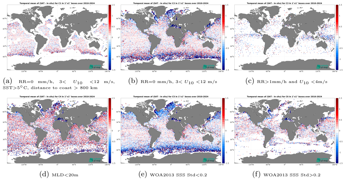
Figure 14: Temporal mean gridded over spatial boxes of size 1^\circ \times 1^\circ of \Delta SSS (SMOS SSS L2Q v331 - No FLAG (CMEMS-CATDS-CPDC) - Argo) for 6 different subdatasets corresponding to:RR=0 mm/h, 3 < U_{10} < 12 m/s, SST>5°C, distance to coast > 800 km (a), RR=0 mm/h, 3 < U_{10} < 12 m/s (b), RR>1mm/h and U_{10} < 4 m/s (c),MLD<20m (d),WOA2013 SSS Std<0.2 (e),WOA2013 SSS Std>0.2 (f).
