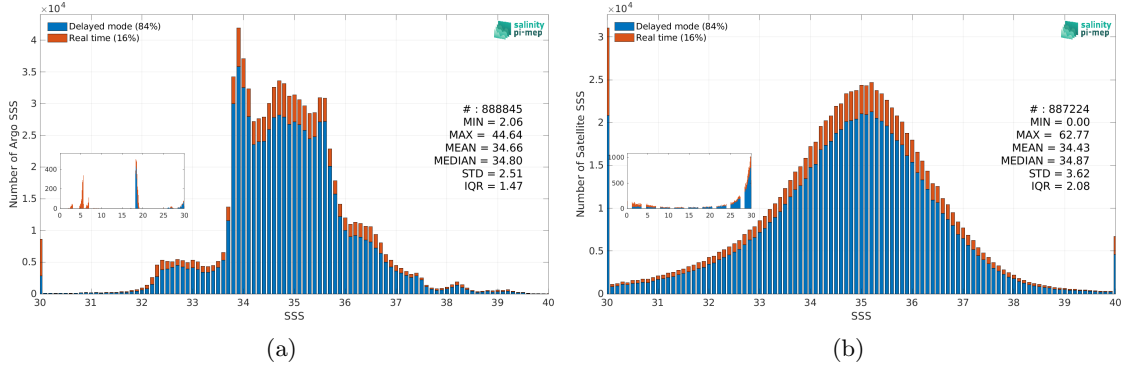
Figure 3: Histograms of SSS from Argo (a) and SMOS SSS L2Q v331 - No FLAG (CMEMS-CATDS-CPDC) (b) considering all match-up pairs per bins of 0.1 over the Global Ocean Pi-MEP region and for the full satellite product period.
