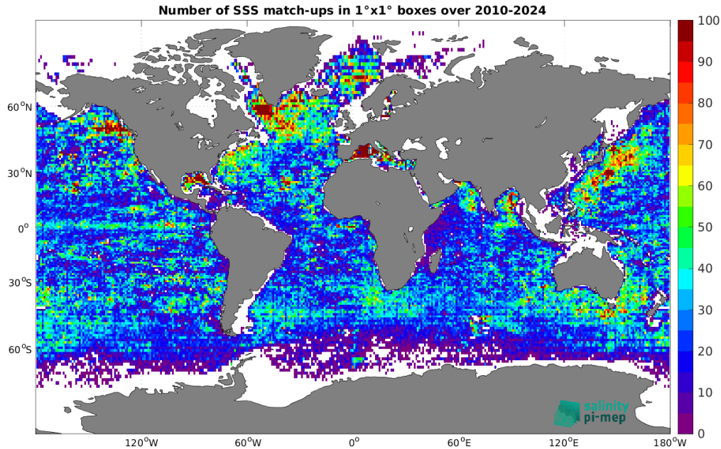
Figure 5: Number of SSS match-ups between Argo SSS and the SMOS SSS L2Q v331 - No FLAG (CMEMS-CATDS-CPDC) SSS product for the Global Ocean Pi-MEP region over 1°x1° boxes and for the full satellite product period.
