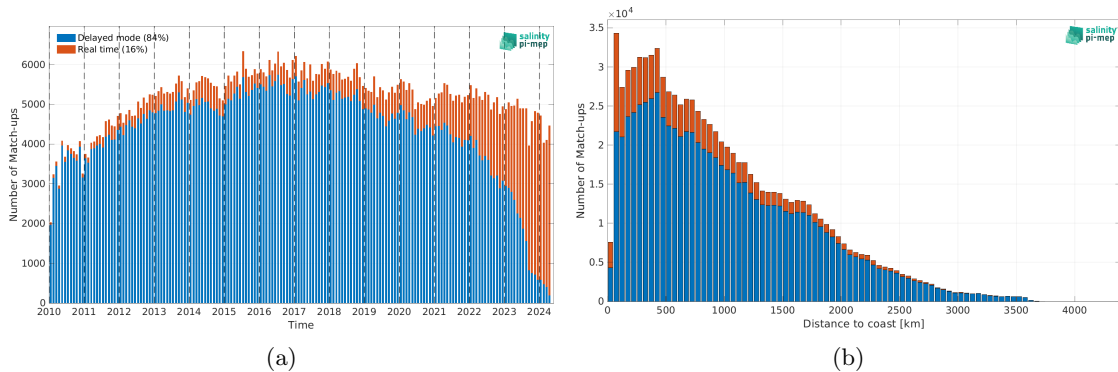
Figure 2: Number of match-ups between Argo and SMOS SSS L2Q v331 - No FLAG (CMEMS-CATDS-CPDC) SSS as a function of time (a) and as function of the distance to coast (b) over the Global Ocean Pi-MEP region and for the full satellite product period.
