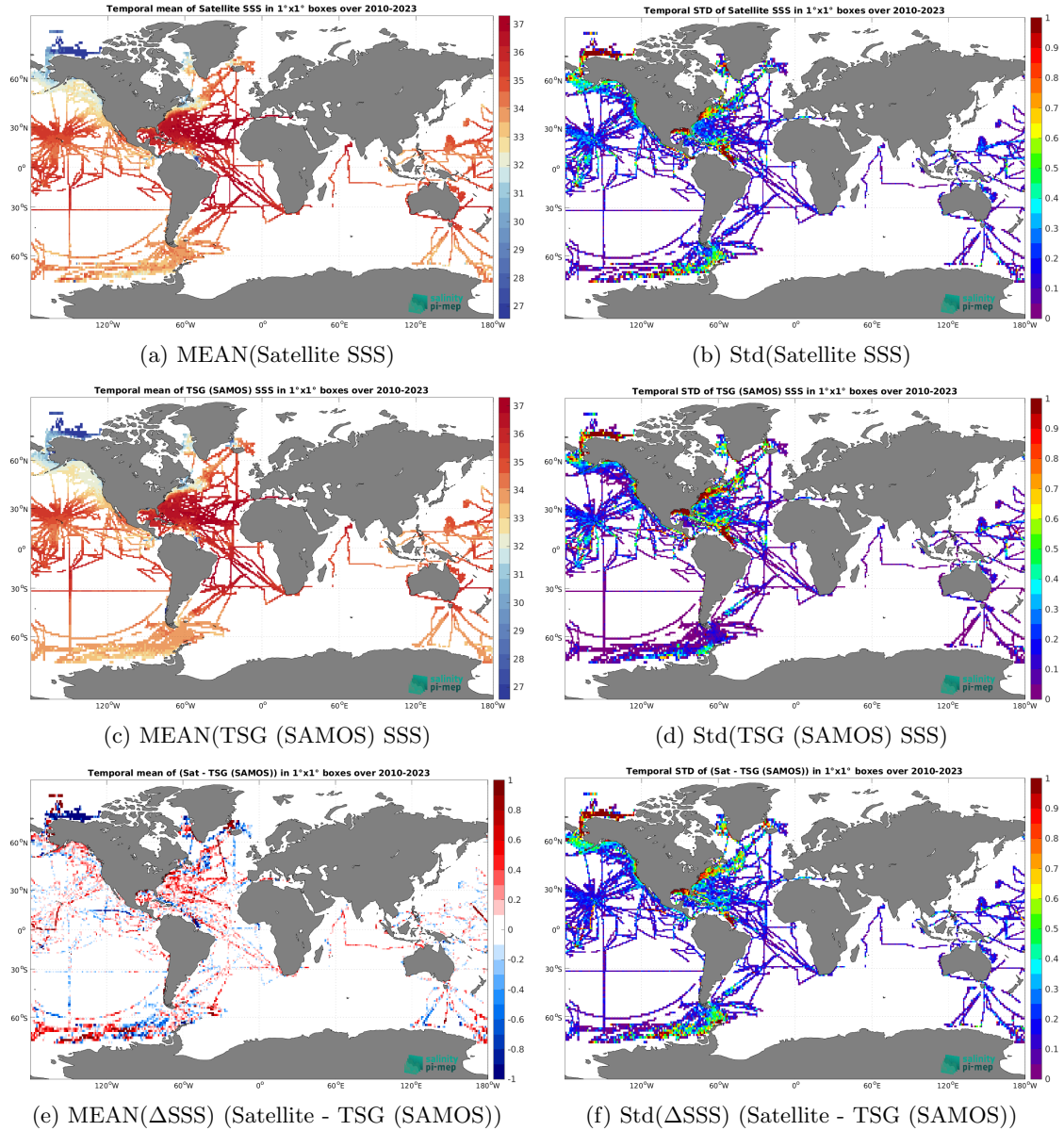
Figure 6: Temporal mean (left) and Std (right) of SSS from SMOS SSS L3 v9 - 9 Days (CATDS-CEC-LOCEAN) (top), TSG (SAMOS) (middle), and of \Delta SSS (Satellite - TSG (SAMOS)). Only match-up pairs are used to generate these maps.
