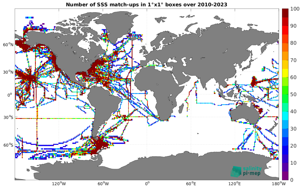
Figure 4: Number of SSS match-ups between TSG (SAMOS) SSS and the SMOS SSS L3 v9 - 9 Days (CATDS-CEC-LOCEAN) SSS product for the Global Ocean Pi-MEP region over 1^\circ \times 1^\circ boxes and for the full satellite product period.
