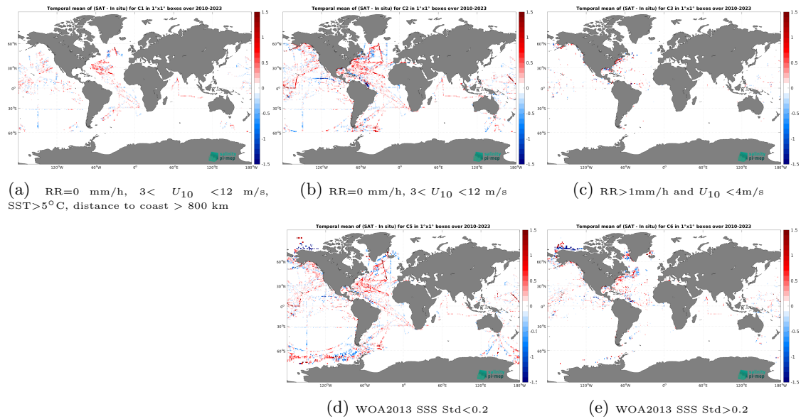
Figure 12: Temporal mean gridded over spatial boxes of size 1^\circ \times 1^\circ of \Delta SSS (SMOS SSS L3 v9 - 9 Days (CATDS-CEC-LOCEAN) - TSG (SAMOS)) for 5 different subdatasets corresponding to:RR=0 mm/h, 3 < U_{10} < 12 m/s, SST >5^\circ C, distance to coast > 800 km (a), RR=0 mm/h, 3 < U_{10} < 12 m/s (b), RR >1 mm/h and U_{10} < 4 m/s (c), WOA2013 SSS Std <0.2 (d), WOA2013 SSS Std >0.2 (e).
