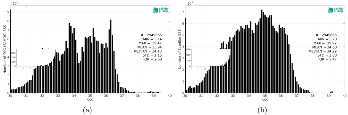
Figure 2: Histograms of SSS from TSG (SAMOS) (a) and SMOS SSS L3 v9 - 9 Days (CATDS-CEC-LOCEAN) (b) considering all match-up pairs per bins of 0.1 over the Global Ocean Pi-MEP region and for the full satellite product period.
