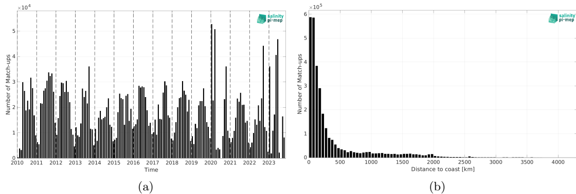
Figure 1: Number of match-ups between TSG (SAMOS) and SMOS SSS L3 v9 - 9 Days (CATDS-CEC-LOCEAN) SSS as a function of time (a) and as function of the distance to coast (b) over the Global Ocean Pi-MEP region and for the full satellite product period.
