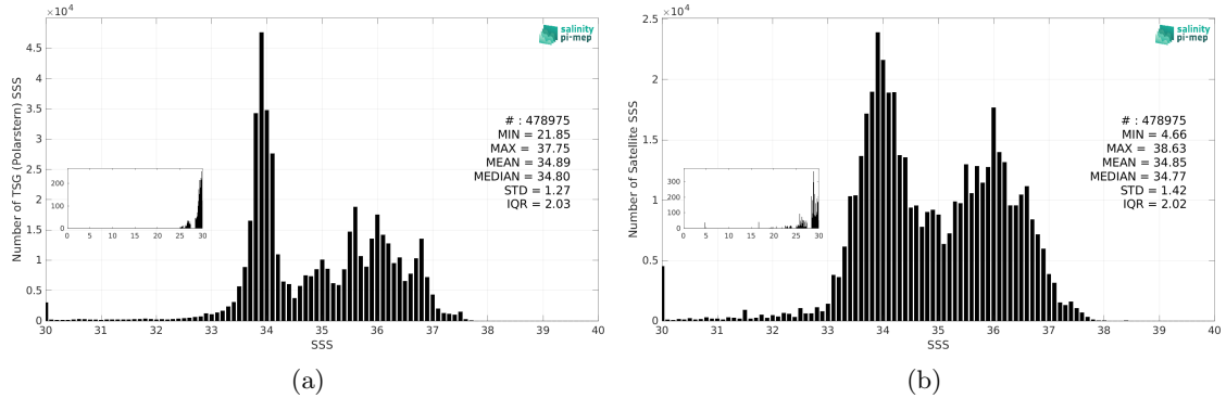
Figure 2: Histograms of SSS from TSG (Polarstern) (a) and SMOS SSS L3 v9 - 9 Days (CATDS-CEC-LOCEAN) (b) considering all match-up pairs per bins of 0.1 over the Global Ocean Pi-MEP region and for the full satellite product period.
