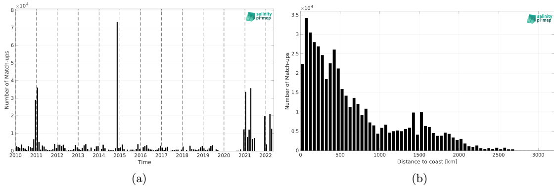
Figure 1: Number of match-ups between TSG (Polarstern) and SMOS SSS L3 v9 - 9 Days (CATDS-CEC-LOCEAN) SSS as a function of time (a) and as function of the distance to coast (b) over the Global Ocean Pi-MEP region and for the full satellite product period.
