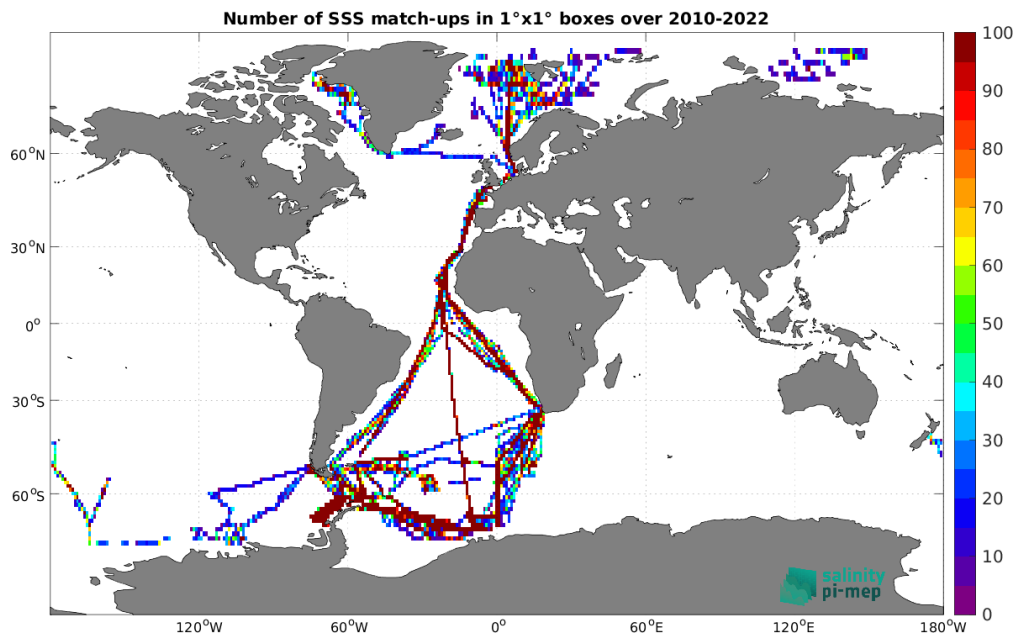
Figure 4: Number of SSS match-ups between TSG (Polarstern) SSS and the SMOS SSS L3 v9 - 9 Days (CATDS-CEC-LOCEAN) SSS product for the Global Ocean Pi-MEP region over 1^\circ \times 1^\circ boxes and for the full satellite product period.
