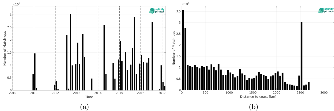
Figure 2: Number of match-ups between TSG (NCEI-0170743) and SMOS SSS L3 v9 - 9 Days (CATDS-CEC-LOCEAN) SSS as a function of time (a) and as function of the distance to coast (b) over the Global Ocean Pi-MEP region and for the full satellite product period.
