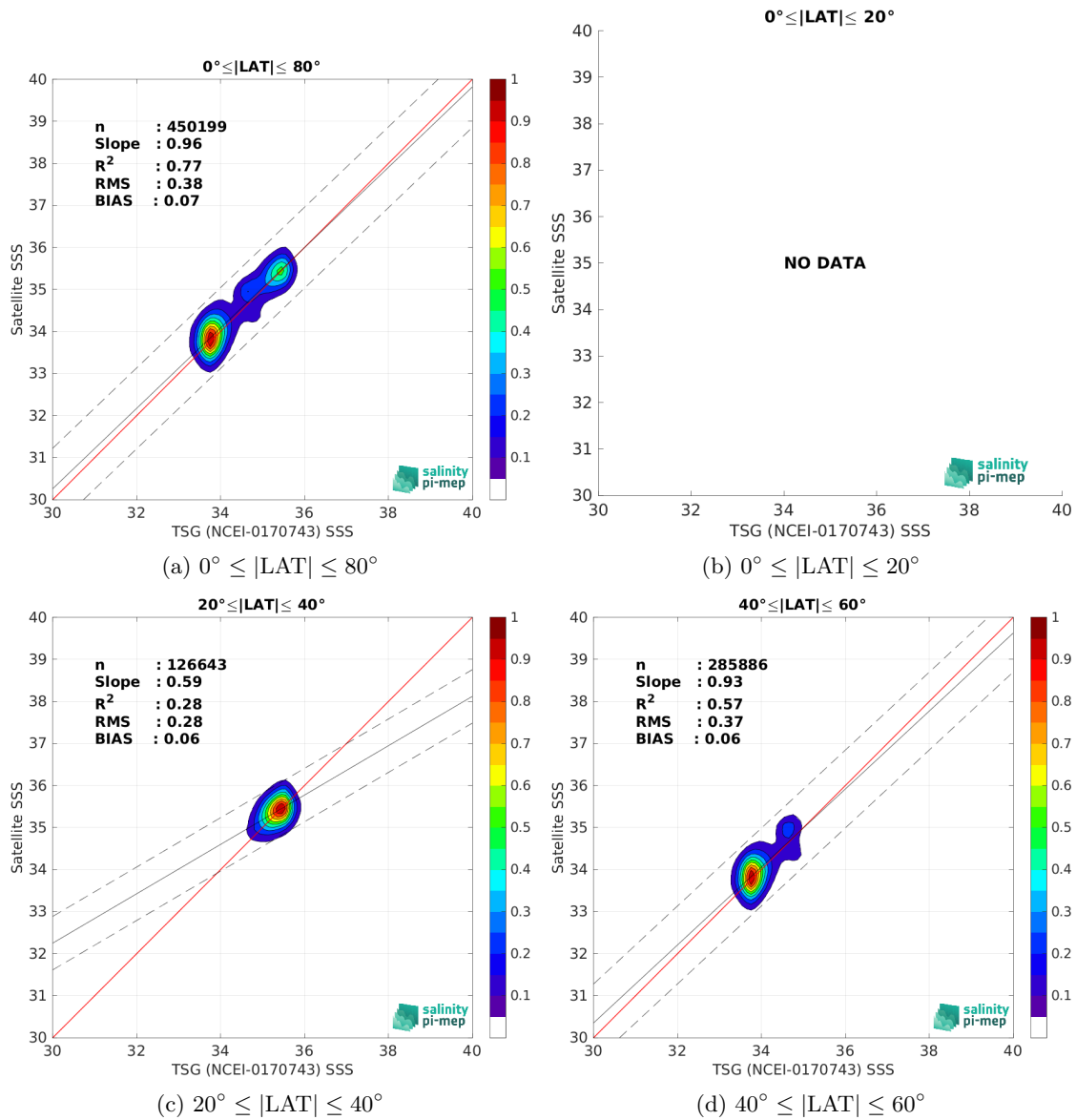
Figure 10: Contour maps of the concentration of SMOS SSS L3 v9 - 9 Days (CATDS-CEC-LOCEAN) SSS (y-axis) versus TSG (NCEI-0170743) SSS (x-axis) at match-up pairs for different latitude bands. For each plot, the red line shows x=y . The black thin and dashed lines indicate a linear fit through the data cloud and the \pm 95\% confidence levels, respectively. The number match-up pairs n , the slope and R^2 coefficient of the linear fit, the root mean square (RMS) and the mean bias between satellite and in situ data are indicated for each latitude band in each plots.
