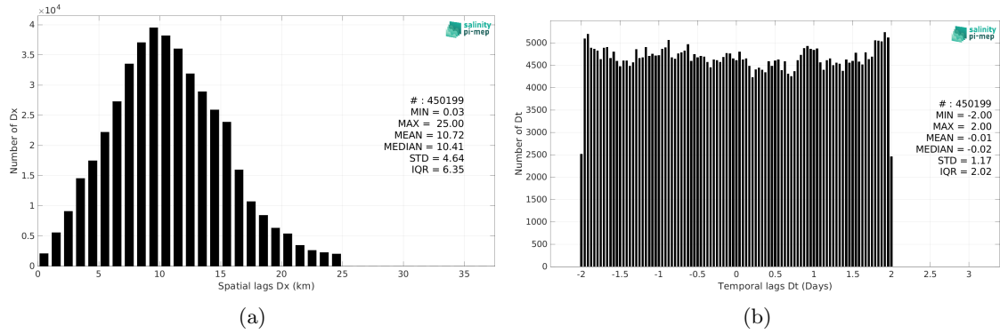
Figure 6: Histograms of the spatial (a) and temporal (b) lags between the location/time of the TSG (NCEI-0170743) measurement and the date of the corresponding SMOS SSS L3 v9 - 9 Days (CATDS-CEC-LOCEAN) SSS pixel.
