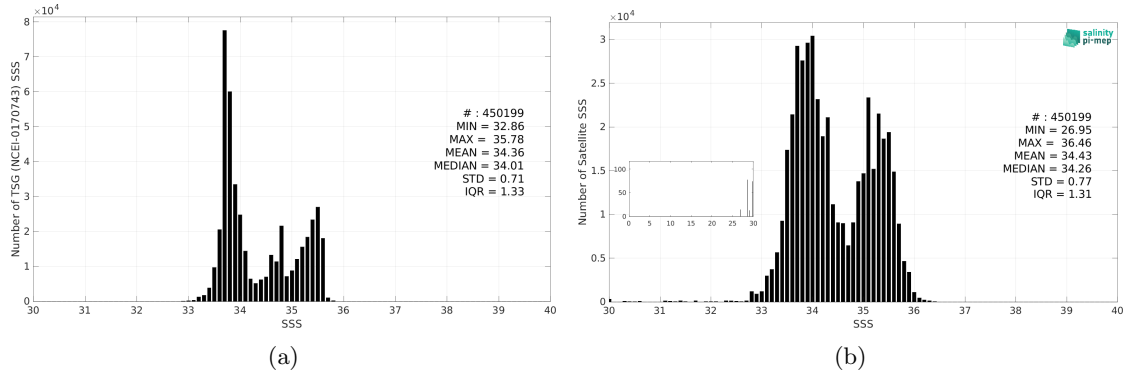
Figure 3: Histograms of SSS from TSG (NCEI-0170743) (a) and SMOS SSS L3 v9 - 9 Days (CATDS-CEC-LOCEAN) (b) considering all match-up pairs per bins of 0.1 over the Global Ocean Pi-MEP region and for the full satellite product period.
