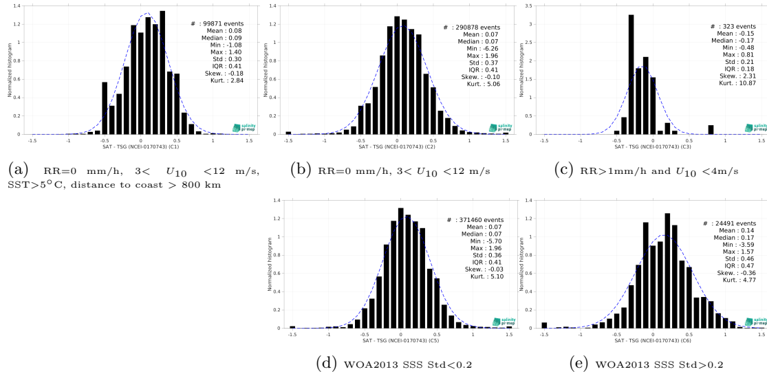
Figure 15: Normalized histogram of \Delta SSS (SMOS SSS L3 v9 - 9 Days (CATDS-CEC-LOCEAN) - TSG (NCEI-0170743)) for 5 different subdatasets corresponding to: RR=0 mm/h, 3 < U_{10} < 12 m/s, SST>5°C, distance to coast > 800 km (a), RR=0 mm/h, 3 < U_{10} < 12 m/s (b), RR>1mm/h and U_{10} < 4 m/s (c), WOA2013 SSS Std<0.2 (d), WOA2013 SSS Std>0.2 (e).
