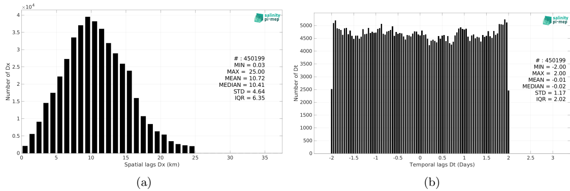
Figure 5: Histograms of the spatial (a) and temporal (b) lags between the location/time of the TSG (NCEI-0170743) measurement and the date of the corresponding SMOS SSS L3 v9 - 9 Days (CATDS-CEC-LOCEAN) SSS pixel.
