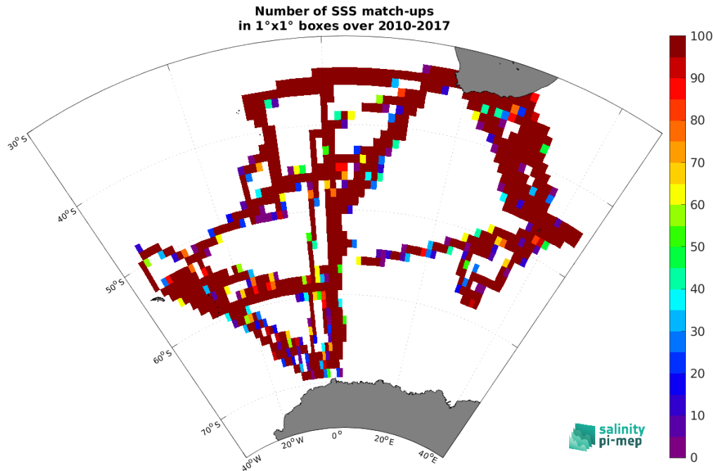
Figure 4: Number of SSS match-ups between TSG (NCEI-0170743) SSS and the SMOS SSS L3 v9 - 9 Days (CATDS-CEC-LOCEAN) SSS product for the Global Ocean Pi-MEP region over 1^\circ \times 1^\circ boxes and for the full satellite product period.
