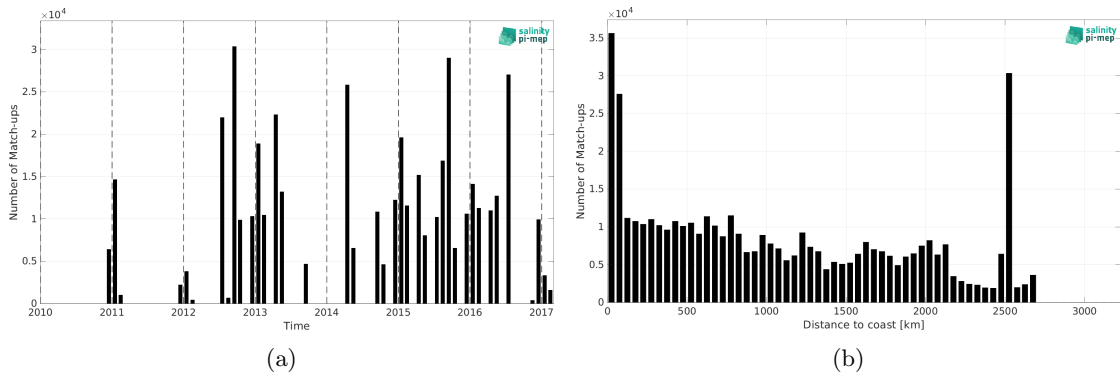
Figure 1: Number of match-ups between TSG (NCEI-0170743) and SMOS SSS L3 v9 - 9 Days (CATDS-CEC-LOCEAN) SSS as a function of time (a) and as function of the distance to coast (b) over the Global Ocean Pi-MEP region and for the full satellite product period.
