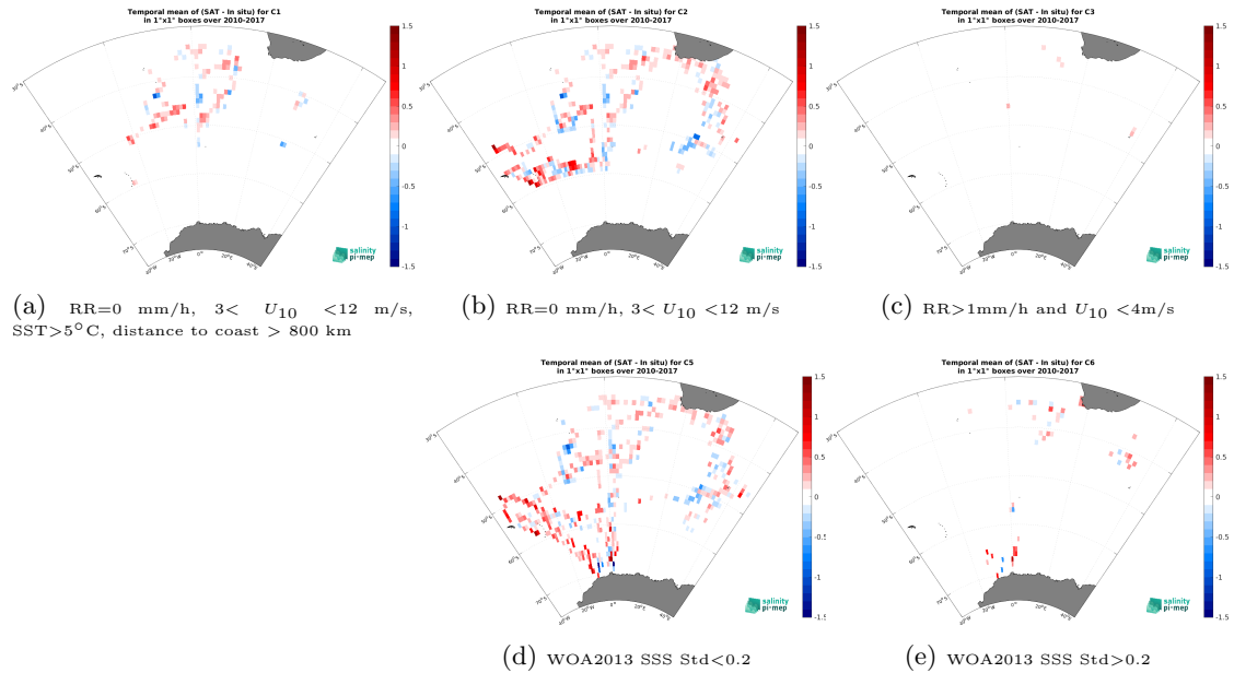
Figure 12: Temporal mean gridded over spatial boxes of size 1^{\circ}\times 1^{\circ} of \Delta\text{SSS} (SMOS SSS L3 v9 - 9 Days (CATDS-CEC-LOCEAN) - TSG (NCEI-0170743)) for 5 different subdatasets corresponding to:RR=0 mm/h, 3 < U_{10} < 12 m/s, SST >5^{\circ}\text{C} , distance to coast > 800 km (a), RR=0 mm/h, 3 < U_{10} < 12 m/s (b), RR >1 mm/h and U_{10} < 4 m/s (c), WOA2013 SSS Std <0.2 (d), WOA2013 SSS Std >0.2 (e).
