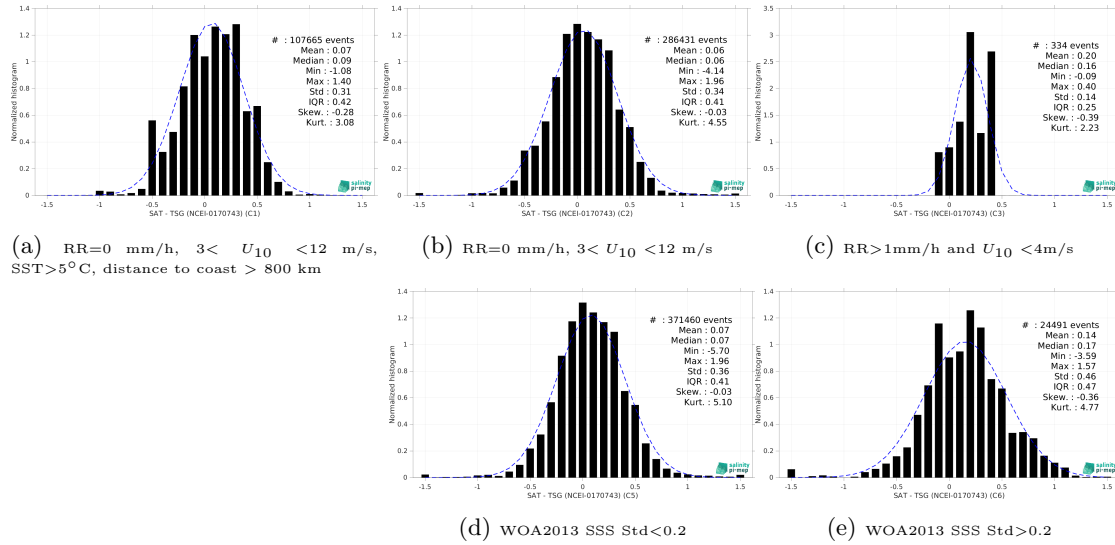
Figure 13: Normalized histogram of \Delta SSS (SMOS SSS L3 v9 - 9 Days (CATDS-CEC-LOCEAN) - TSG (NCEI-0170743)) for 5 different subdatasets corresponding to: RR=0 mm/h, 3 < U_{10} < 12 m/s, SST > 5°C, distance to coast > 800 km (a), RR=0 mm/h, 3 < U_{10} < 12 m/s (b), RR > 1mm/h and U_{10} < 4 m/s (c), WOA2013 SSS Std < 0.2 (d), WOA2013 SSS Std > 0.2 (e).
