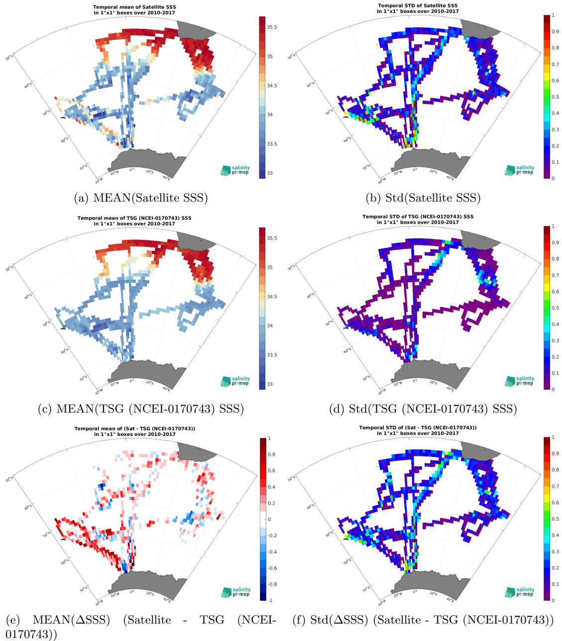
Figure 6: Temporal mean (left) and Std (right) of SSS from SMOS SSS L3 v9 - 9 Days (CATDS-CEC-LOCEAN) (top), TSG (NCEI-0170743) (middle), and of \Delta SSS (Satellite - TSG (NCEI-0170743)). Only match-up pairs are used to generate these maps.
