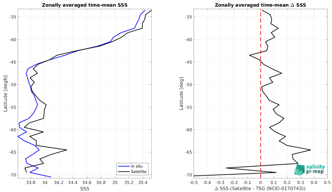
Figure 8: Left panel: Zonal mean SSS from SMOS SSS L3 v9 - 9 Days (CATDS-CEC-LOCEAN) satellite product (black) and from TSG (NCEI-0170743) (blue). Right panel: Zonal mean of \Delta SSS (Satellite - TSG (NCEI-0170743)) for all the collected Pi-MEP match-up pairs estimated over the full satellite product period.
