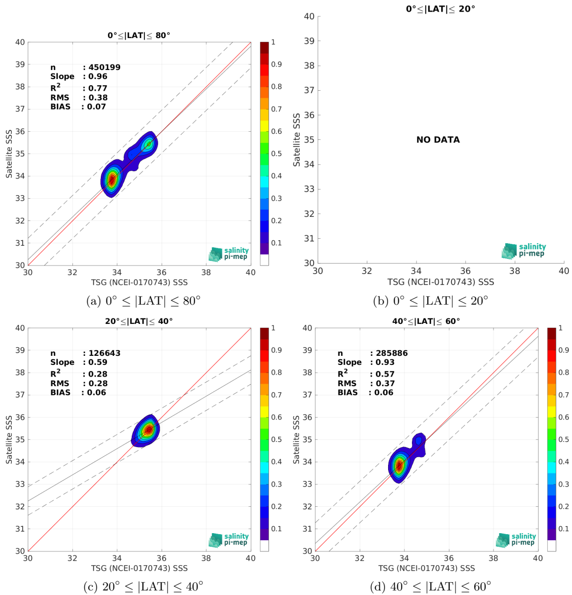
Figure 9: Contour maps of the concentration of SMOS SSS L3 v9 - 9 Days (CATDS-CEC-LOCEAN) SSS (y-axis) versus TSG (NCEI-0170743) SSS (x-axis) at match-up pairs for different latitude bands. For each plot, the red line shows x=y . The black thin and dashed lines indicate a linear fit through the data cloud and the \pm 95\% confidence levels, respectively. The number match-up pairs n , the slope and R^2 coefficient of the linear fit, the root mean square (RMS) and the mean bias between satellite and in situ data are indicated for each latitude band in each plots.
