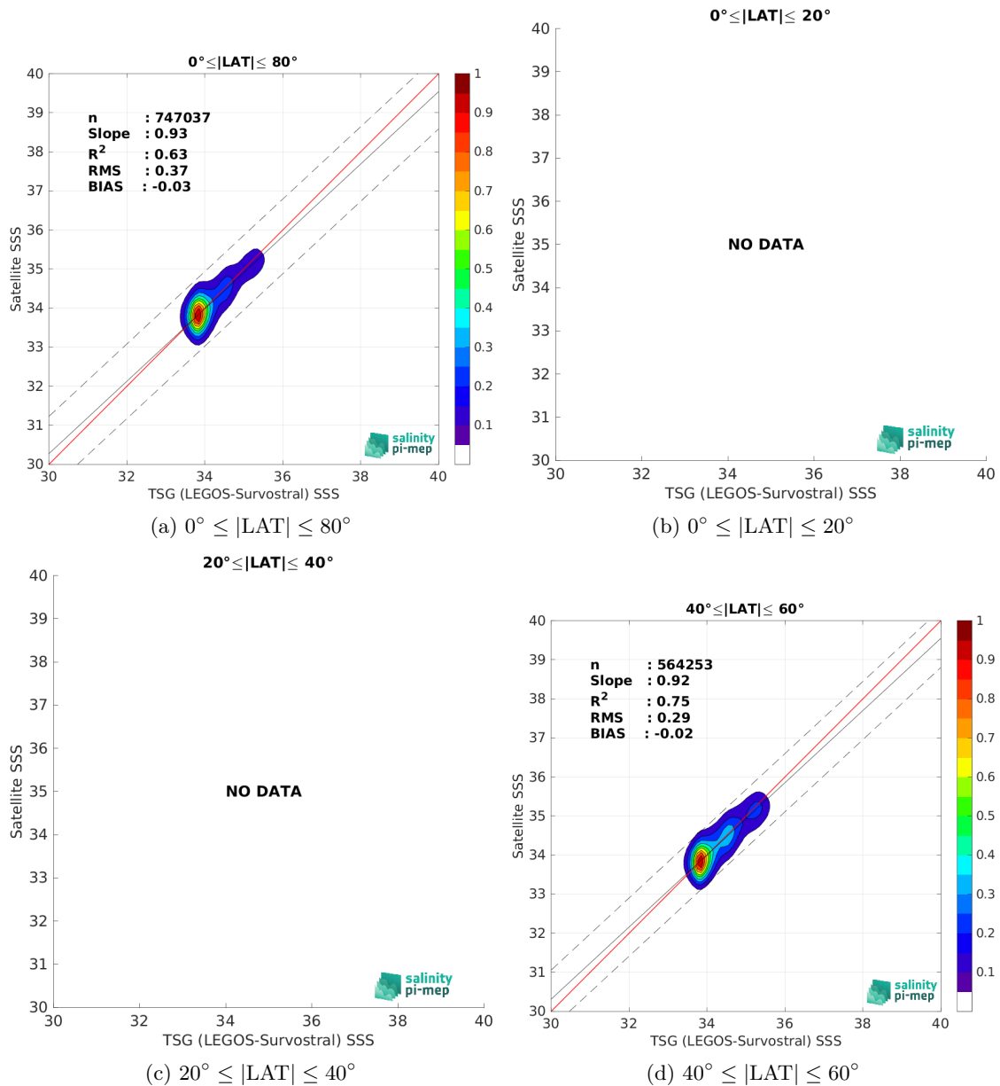
Figure 10: Contour maps of the concentration of SMOS SSS L3 v9 - 9 Days (CATDS-CEC-LOCEAN) SSS (y-axis) versus TSG (LEGOS-Survostral) SSS (x-axis) at match-up pairs for different latitude bands. For each plot, the red line shows x=y . The black thin and dashed lines indicate a linear fit through the data cloud and the \pm 95\% confidence levels, respectively. The number match-up pairs n , the slope and R^2 coefficient of the linear fit, the root mean square (RMS) and the mean bias between satellite and in situ data are indicated for each latitude band in each plots.
