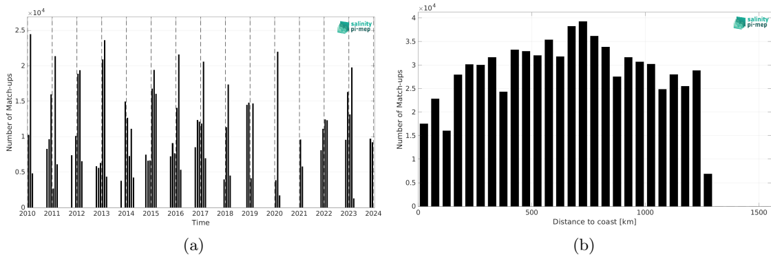
Figure 2: Number of match-ups between TSG (LEGOS-Survostral) and SMOS SSS L3 v9 - 9 Days (CATDS-CEC-LOCEAN) SSS as a function of time (a) and as function of the distance to coast (b) over the Global Ocean Pi-MEP region and for the full satellite product period.
