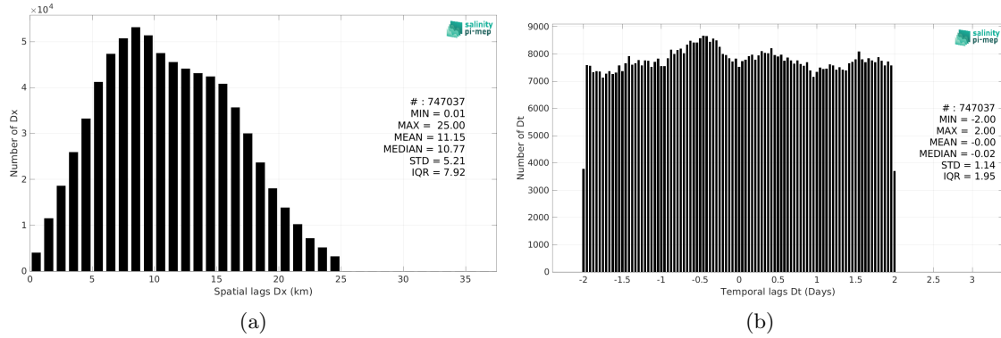
Figure 6: Histograms of the spatial (a) and temporal (b) lags between the location/time of the TSG (LEGOS-Survostral) measurement and the date of the corresponding SMOS SSS L3 v9 - 9 Days (CATDS-CEC-LOCEAN) SSS pixel.
