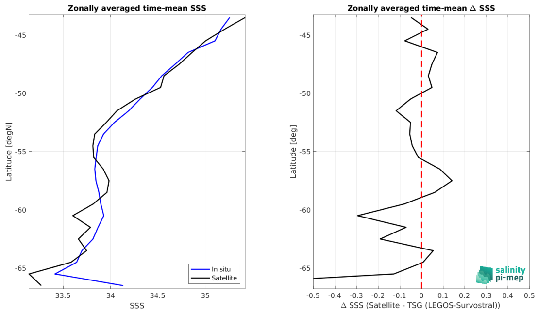
Figure 9: Left panel: Zonal mean SSS from SMOS SSS L3 v9 - 9 Days (CATDS-CEC-LOCEAN) satellite product (black) and from TSG (LEGOS-Survostral) (blue). Right panel: Zonal mean of \Delta SSS (Satellite - TSG (LEGOS-Survostral)) for all the collected Pi-MEP match-up pairs estimated over the full satellite product period.
