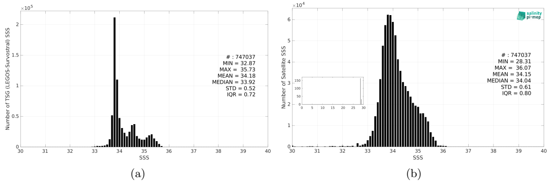
Figure 3: Histograms of SSS from TSG (LEGOS-Survostral) (a) and SMOS SSS L3 v9 - 9 Days (CATDS-CEC-LOCEAN) (b) considering all match-up pairs per bins of 0.1 over the Global Ocean Pi-MEP region and for the full satellite product period.
