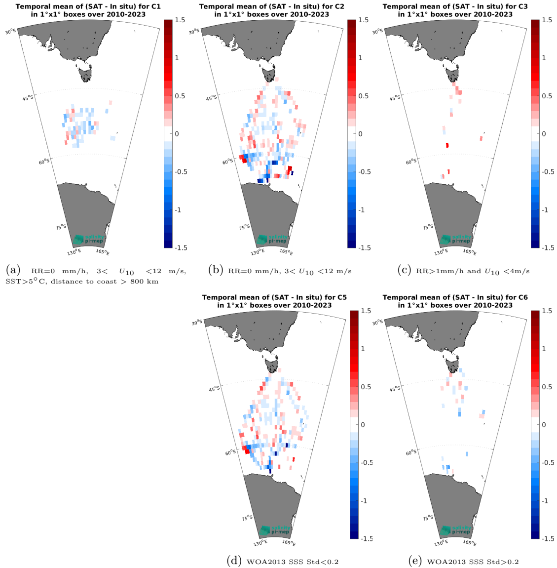
Figure 14: Temporal mean gridded over spatial boxes of size 1^\circ \times 1^\circ of \Delta\text{SSS} (SMOS SSS L3 v9 - 9 Days (CATDS-CEC-LOCEAN) - TSG (LEGOS-Survostral)) for 5 different subdatasets corresponding to: RR=0 mm/h, 3 < U_{10} < 12 m/s, SST > 5^\circ\text{C} , distance to coast > 800 km (a), RR=0 mm/h, 3 < U_{10} < 12 m/s (b), RR > 1 mm/h and U_{10} < 4 m/s (c), WOA2013 SSS Std < 0.2 (d), WOA2013 SSS Std > 0.2 (e).
