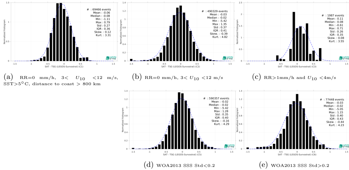
Figure 15: Normalized histogram of \Delta SSS (SMOS SSS L3 v9 - 9 Days (CATDS-CEC-LOCEAN) - TSG (LEGOS-Survostral)) for 5 different subdatasets corresponding to: RR=0 mm/h, 3 < U_{10} < 12 m/s, SST > 5°C, distance to coast > 800 km (a), RR=0 mm/h, 3 < U_{10} < 12 m/s (b), RR > 1mm/h and U_{10} < 4 m/s (c), WOA2013 SSS Std < 0.2 (d), WOA2013 SSS Std > 0.2 (e).
